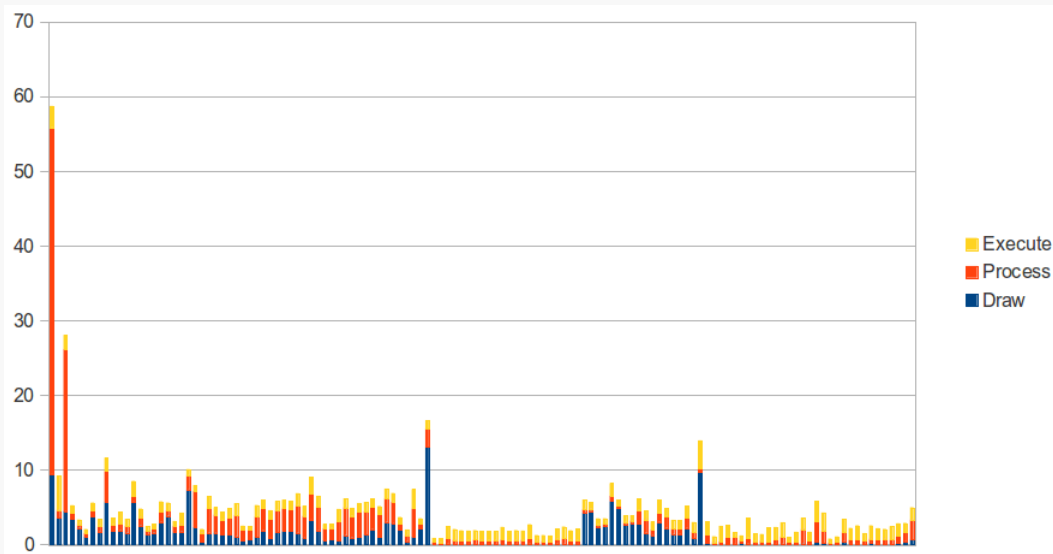
Figure 1020: gfxinfo Output of Revised ThreePaneDemoBC
