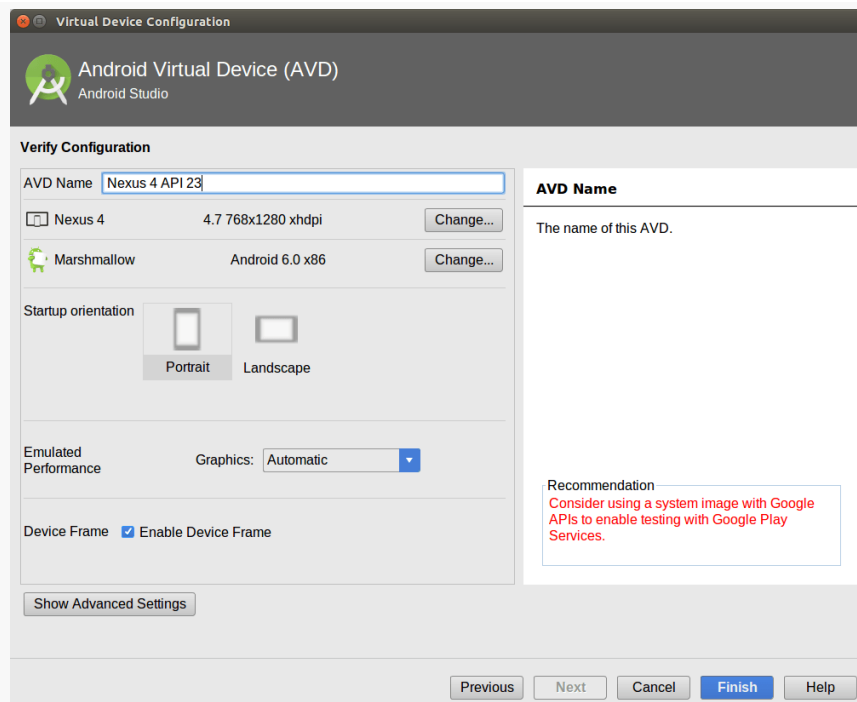
Figure 30: Android Studio Virtual Device Configuration Wizard, Third Page
