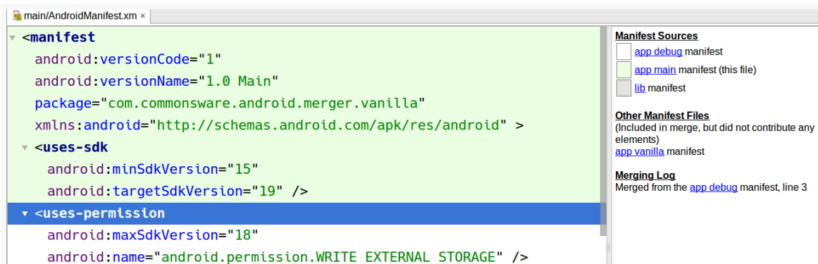
Figure 357: Merged Manifest View, Showing Merged Element
