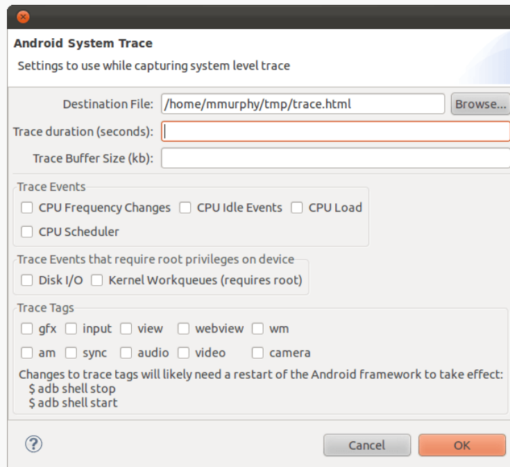
Figure 1004: Systrace Dialog in Android Device Monitor
