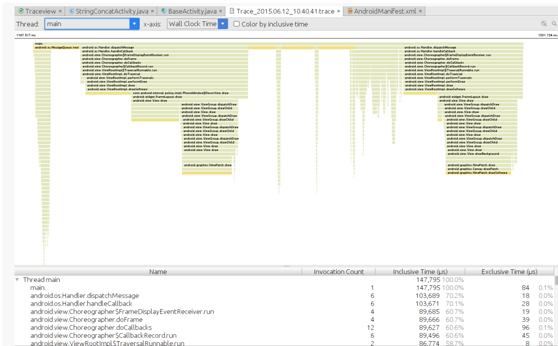
Figure 996: Android Studio, Trace Results Tab
