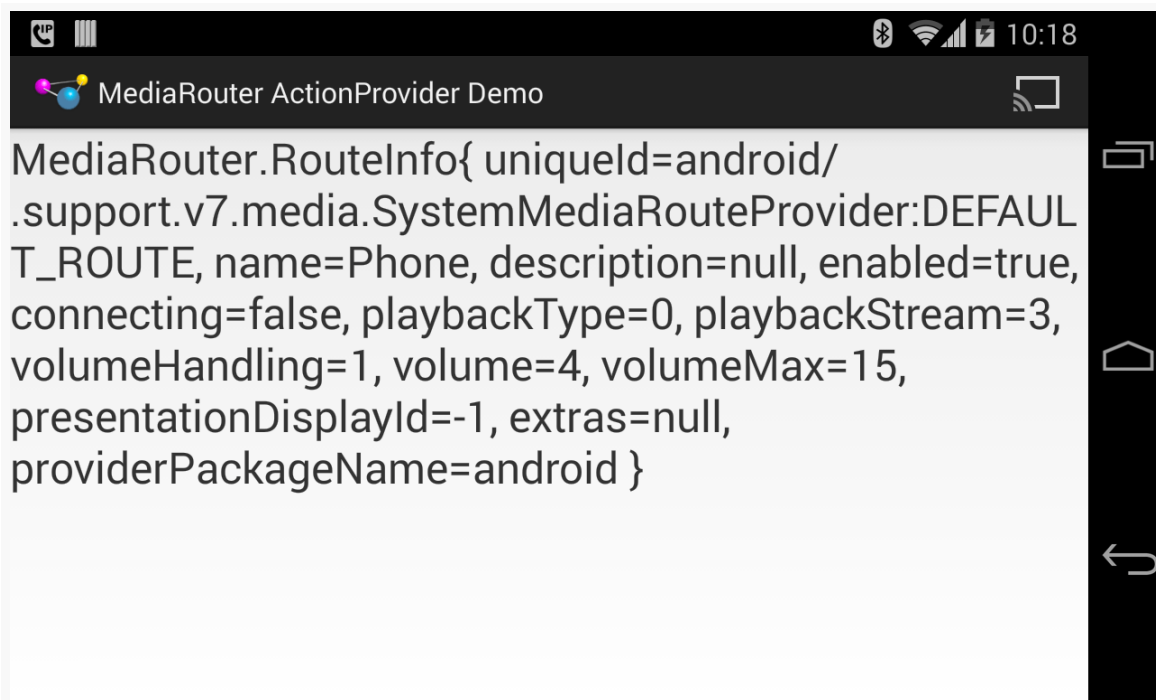
Figure 822: MediaRouter ActionProvider Demo, on a Nexus 4, Showing ActionProvider
