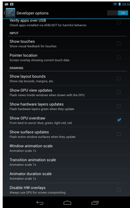
Figure 1011: Nexus 7 Developer Options, with “Show GPU overdraw”
