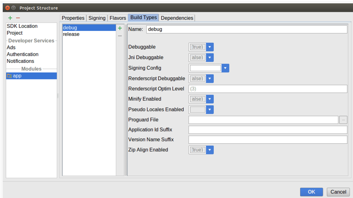
Figure 933: Project Structure Dialog, Module Category, Build Types Tab
