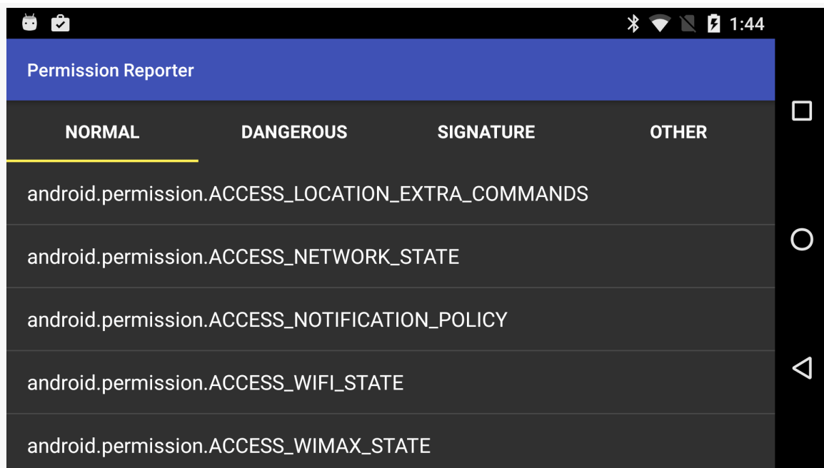
Figure 858: PermissionReporter, Normal Tab, on Android 6.0
