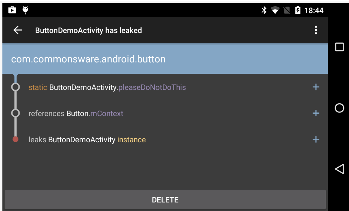
Figure 1051: LeakCanary Diagnostic Activity, As Launched From the Notification
