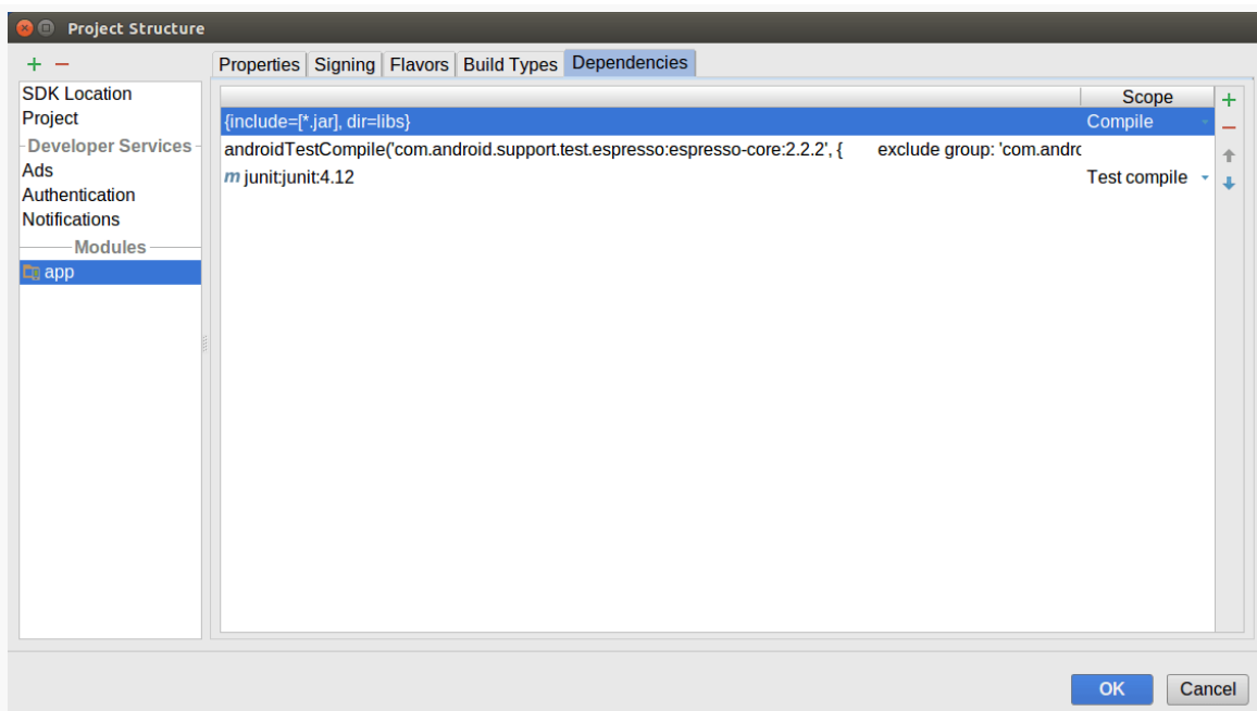
Figure 934: Project Structure Dialog, Module Category, Dependencies Tab
