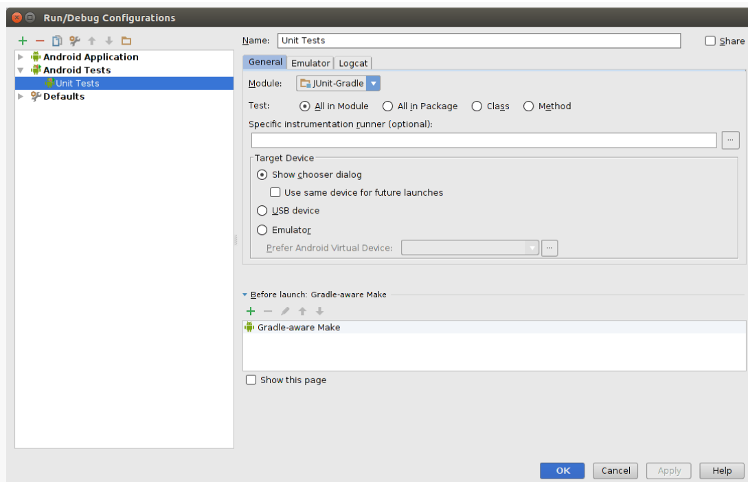
Figure 374: Android Studio, Showing New “Tests” Run Configuration
