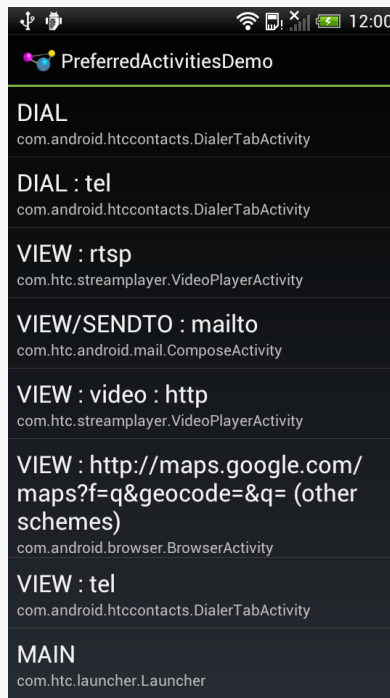
Figure 910: Preferred Activities on a Stock HTC One S
