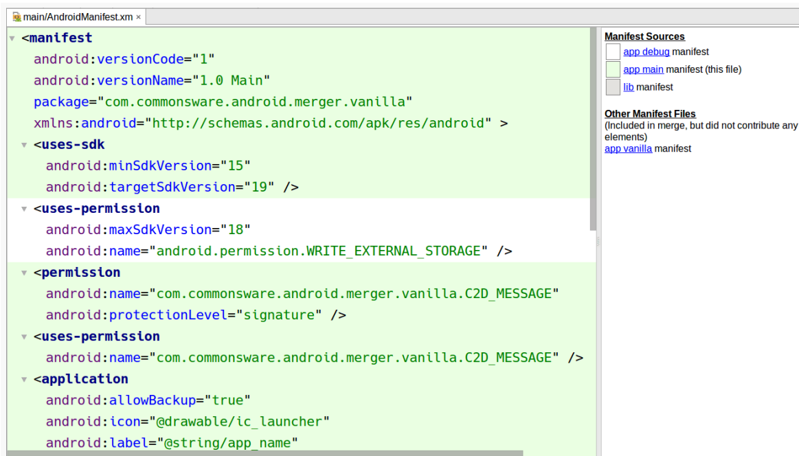
Figure 355: Merged Manifest Tab
