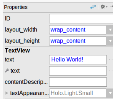
Figure 90: Properties Pane, Showing TextView “text” Property
