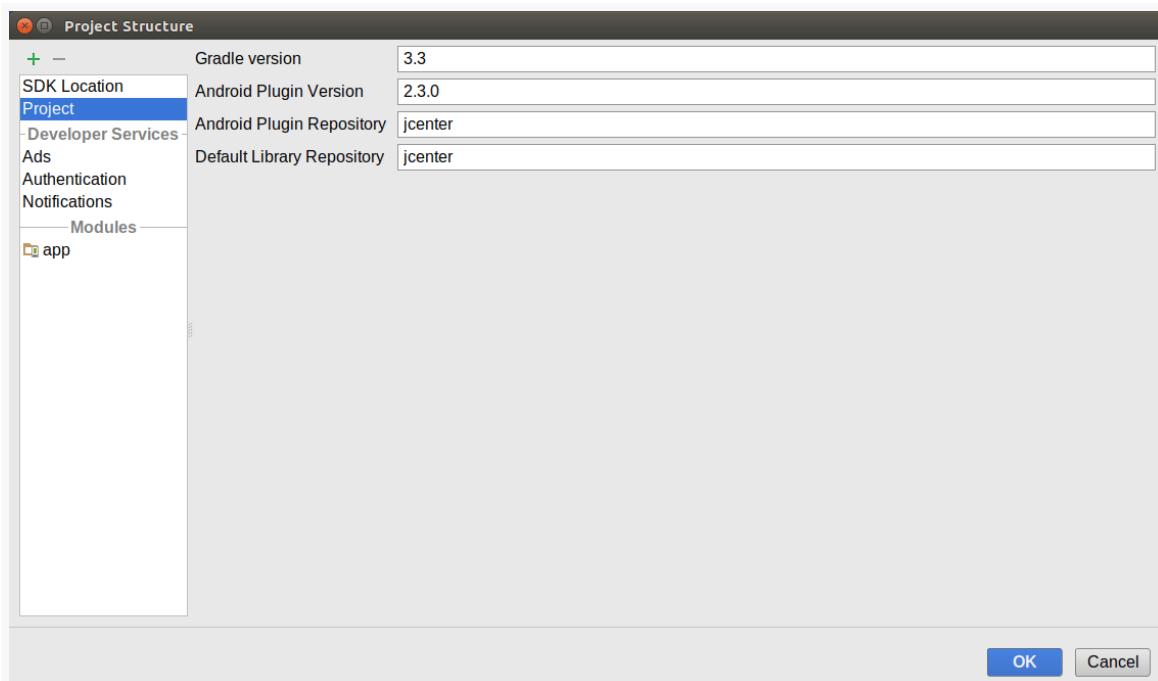
Figure 928: Project Structure Dialog, Project Settings Category
