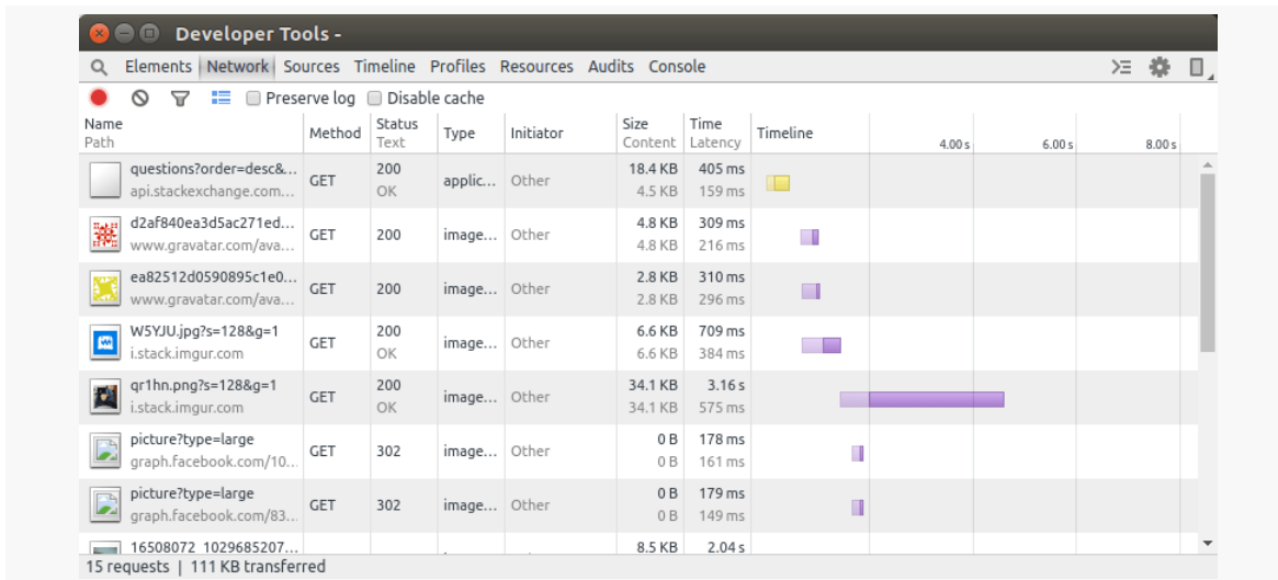
Figure 983: Network Tool, Showing HTTP Requests from Sample App Refresh
