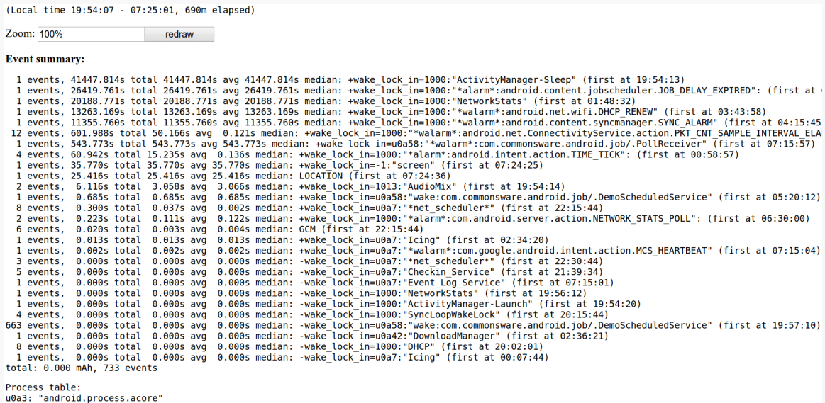
Figure 1063: Battery Historian Timeline, Zoom and “Event summary”
