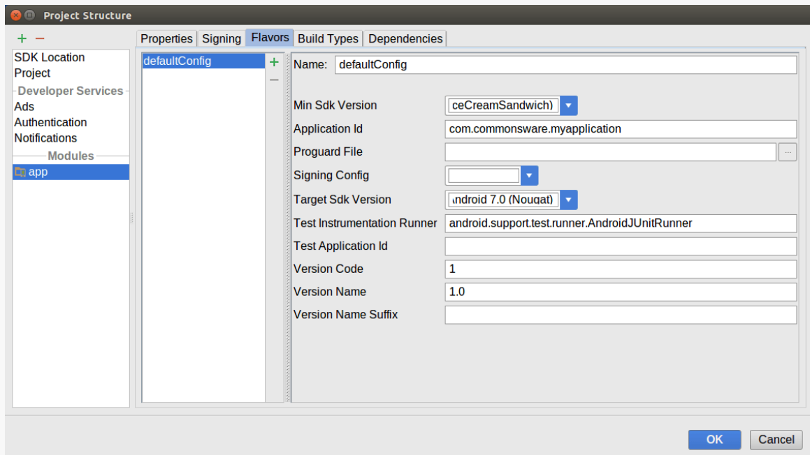
Figure 932: Project Structure Dialog, Module Category, Flavors Tab
