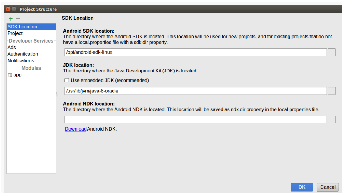
Figure 927: Project Structure Dialog, SDK Location Category
