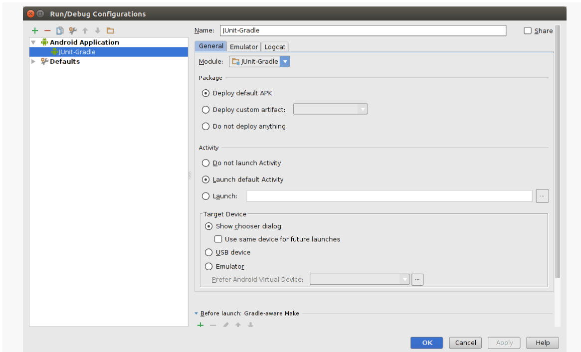
Figure 372: Android Studio Run Configurations Dialog
