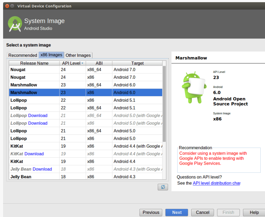
Figure 29: Android Studio Virtual Device Configuration Wizard, After Choosing Image
