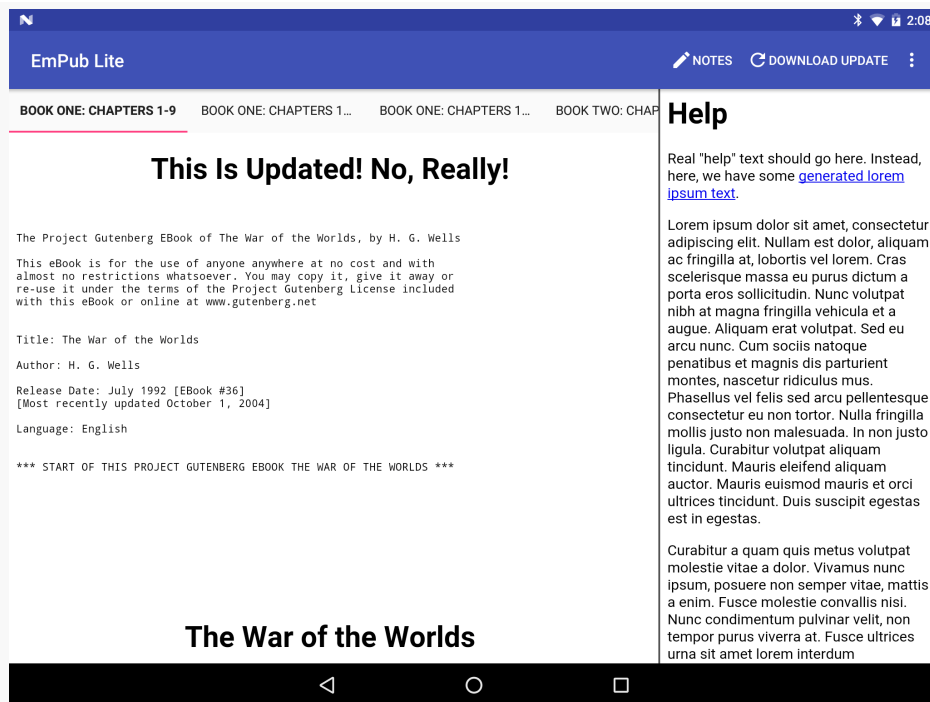
Figure 342: EmPubLite, on a Tablet-Sized Emulator, With Help
