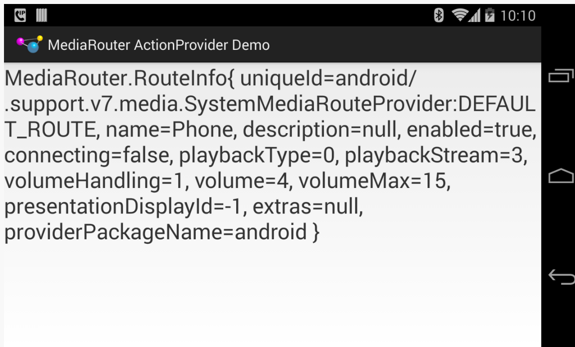
Figure 816: MediaRouter ActionProvider Demo, on a Nexus 4, Showing Default Route
