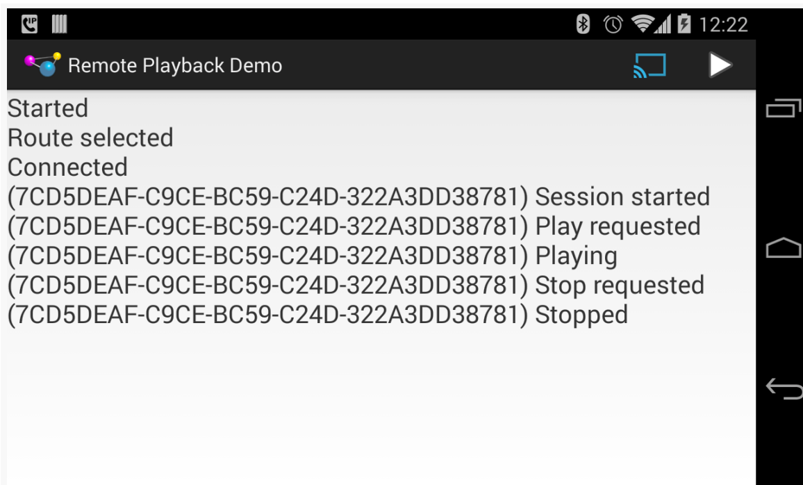
Figure 831: RemotePlaybackClient Demo, on a Nexus 4, After Playback Has Stopped
