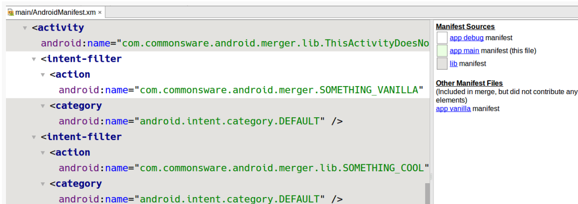
Figure 359: Merged Manifest View, Showing Merged Element
