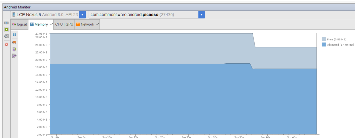
Figure 1033: Android Studio, Android Monitor, Memory Tab, Showing Shrunk Heap
