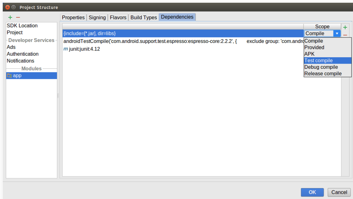
Figure 935: Dependencies Tab, Showing Scope Drop-Down
