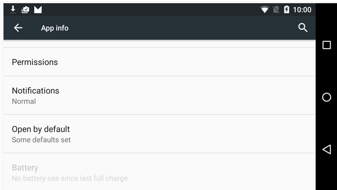
Figure 899: URLHandlerMNC in Settings, “Open by default” Visible
