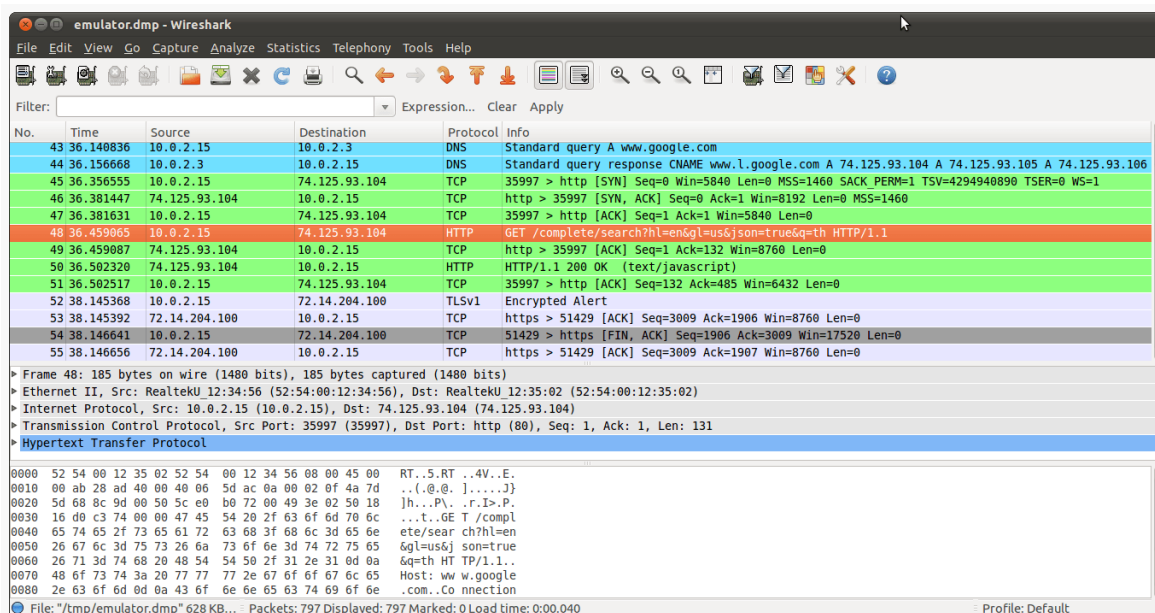
Figure 1026: Wireshark examining captured emulator packets
