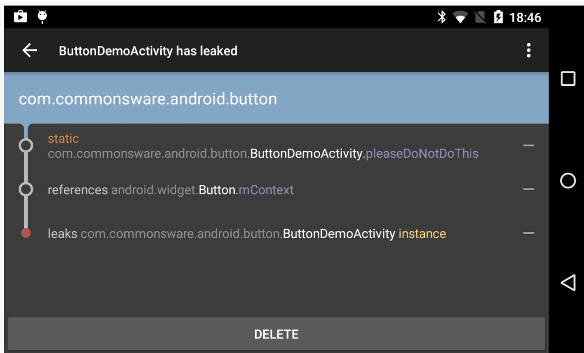
Figure 1052: LeakCanary Diagnostic Activity, Showing Full Package Names
