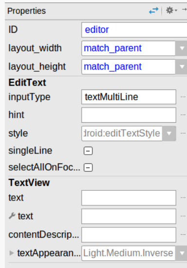
Figure 169: Graphical Layout Editor Properties Pane
