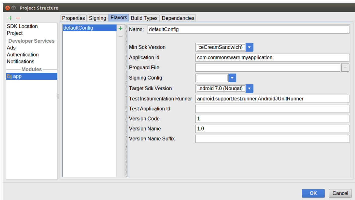
Figure 929: Project Structure Dialog, Module Category, Flavors Tab
