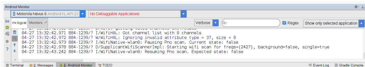
Figure 113: Android DDMS Tool Window, Showing LogCat
