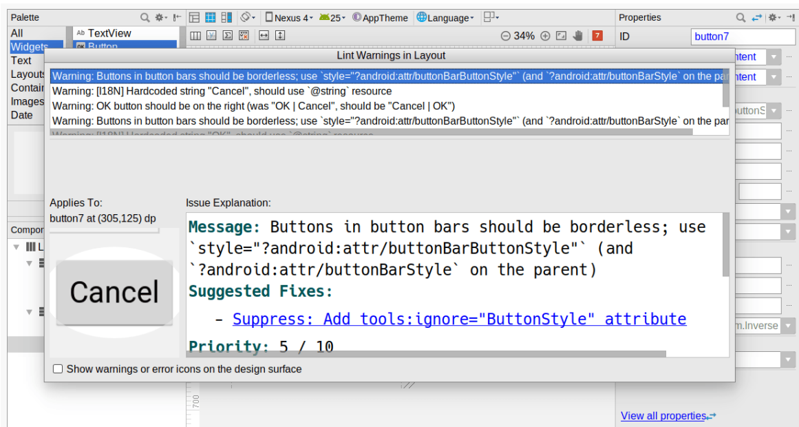
Figure 136: Layout Warning Messages
