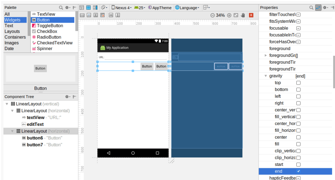
Figure 134: Two Smaller Right-Flush Buttons in Lower Horizontal LinearLayout
