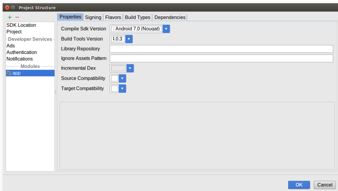
Figure 927: Project Structure Dialog, Module Category, Properties Tab
