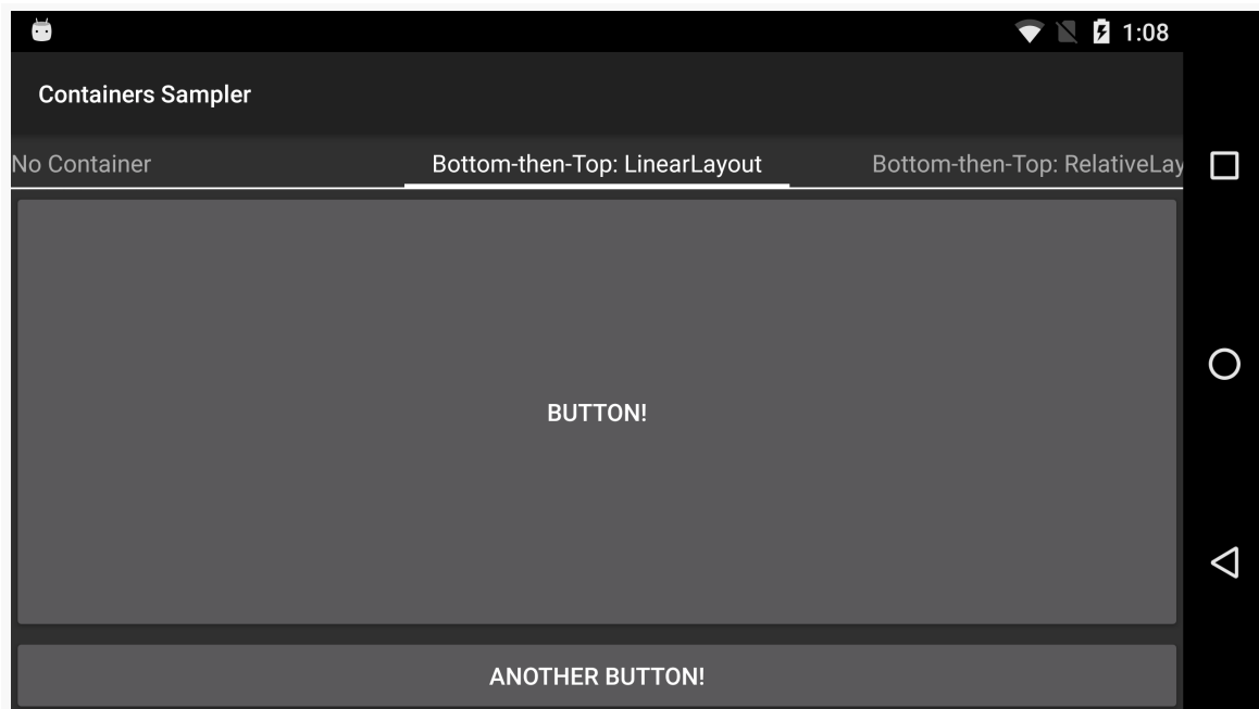
Figure 119: Bottom-then-Top Layout, Using LinearLayout
