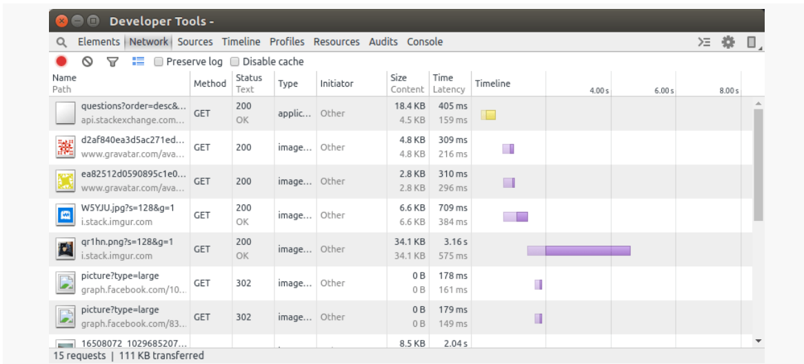
Figure 975: Network Tool, Showing HTTP Requests from Sample App Refresh
