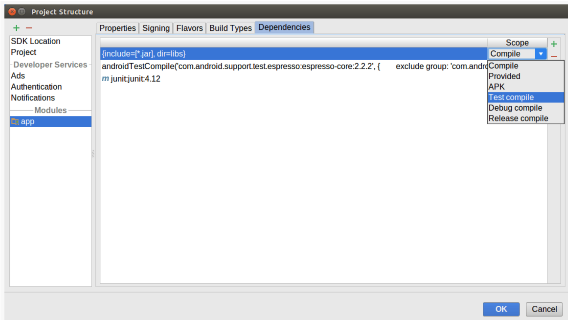
Figure 927: Dependencies Tab, Showing Scope Drop-Down
