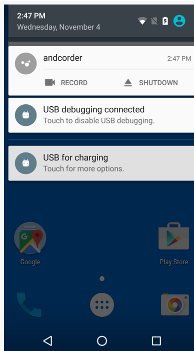
Figure 846: andcorder Notification, Showing Record and Shutdown Actions
