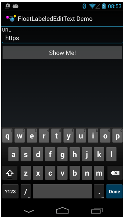
Figure 538: FloatingLabelNative Sample, As Initially Launched
