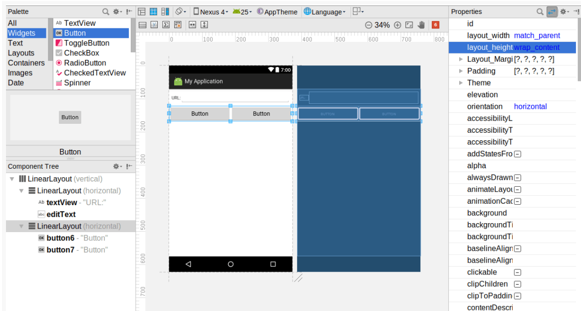
Figure 130: Two Buttons in Lower Horizontal LinearLayout
