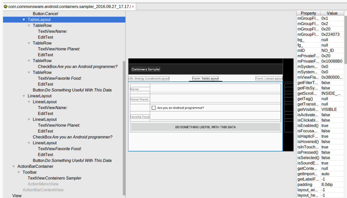
Figure 960: Layout Inspector, As Initially Launched
