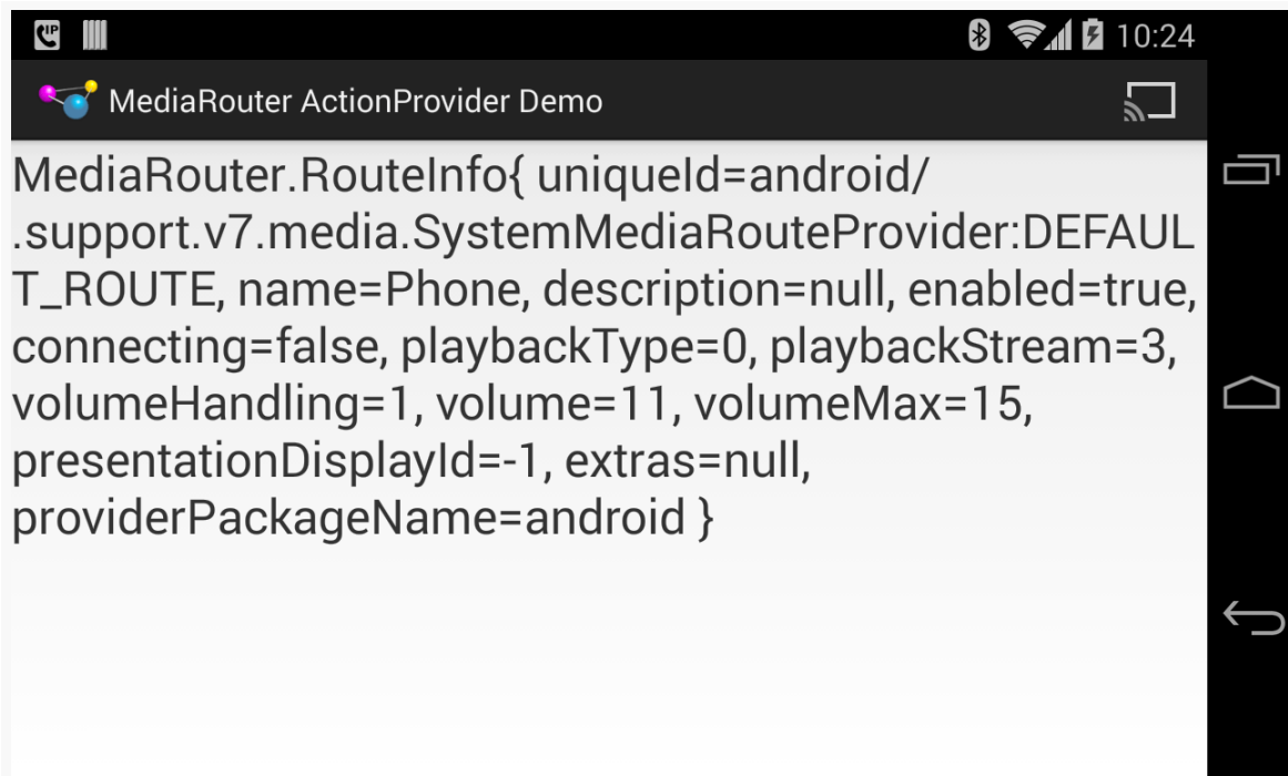
Figure 812: MediaRouter ActionProvider Demo, on a Nexus 4, Showing Default Route and Provider
