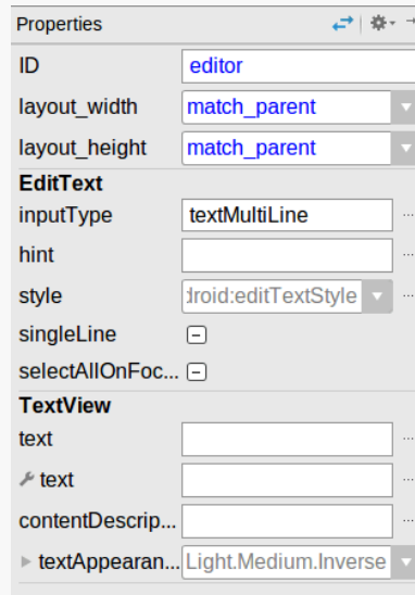
Figure 167: Graphical Layout Editor Properties Pane
