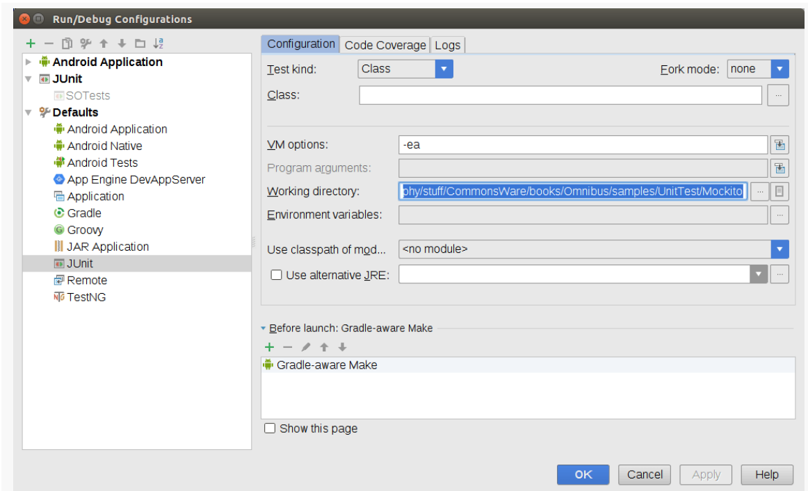
Figure 397: Run/Debug Configurations, JUnit Defaults, Unmodified
