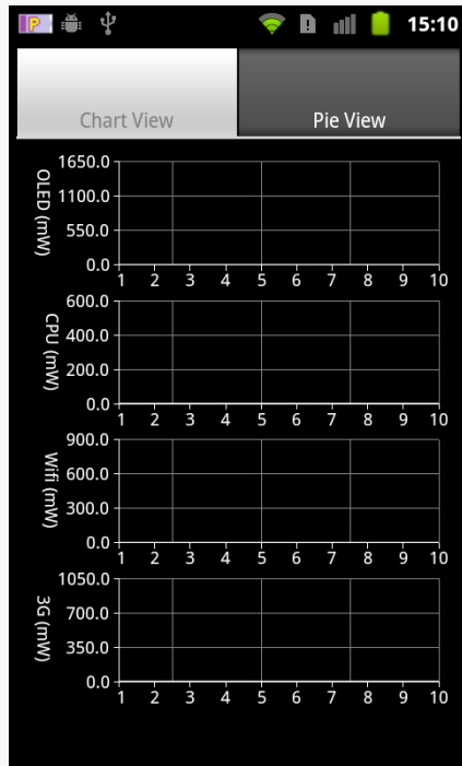
Figure 1057: The PowerTutor live charts for a single process current power consumption
