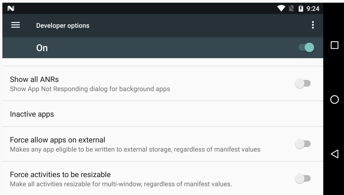
Figure 463: Resizable Windows Developer Setting
