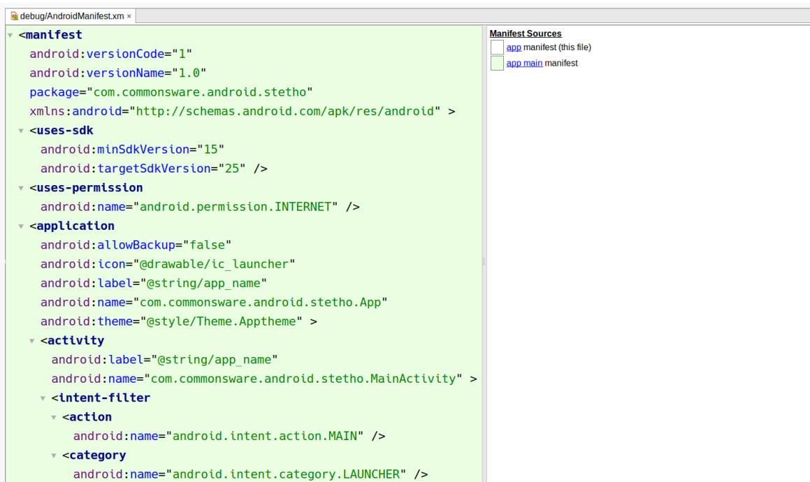
Figure 971: Merged Manifest for Release Build, Showing No StethoApp
