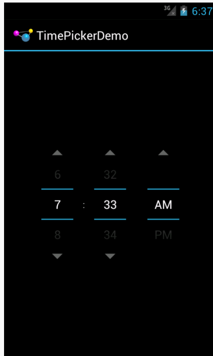
Figure 1097: Android 4.0.3
