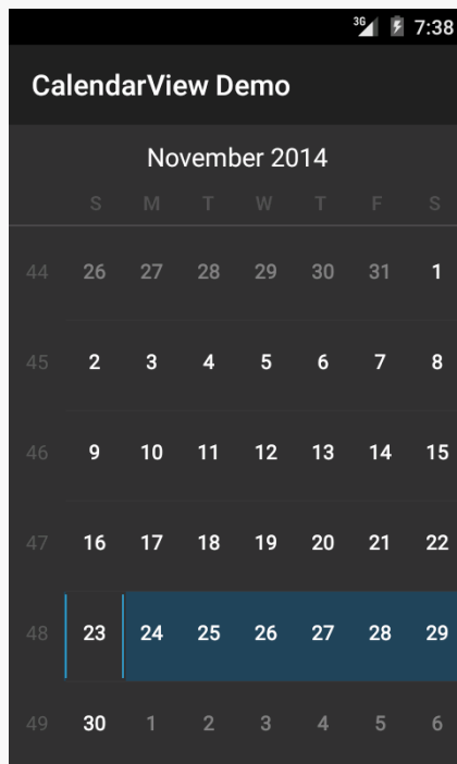
Figure 1077: Android 5.0
