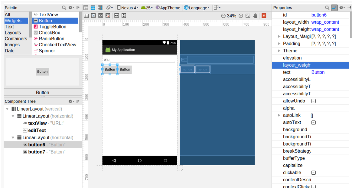
Figure 131: Two Smaller Buttons in Lower Horizontal LinearLayout
