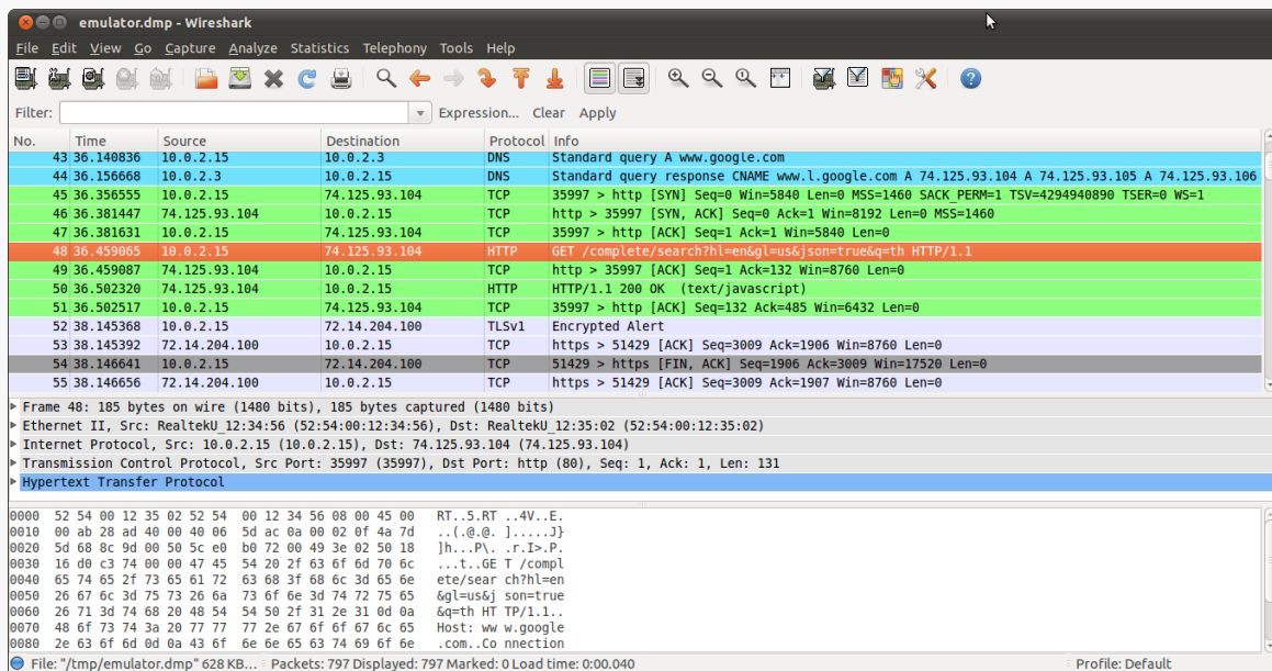
Figure 1017: Wireshark examining captured emulator packets
