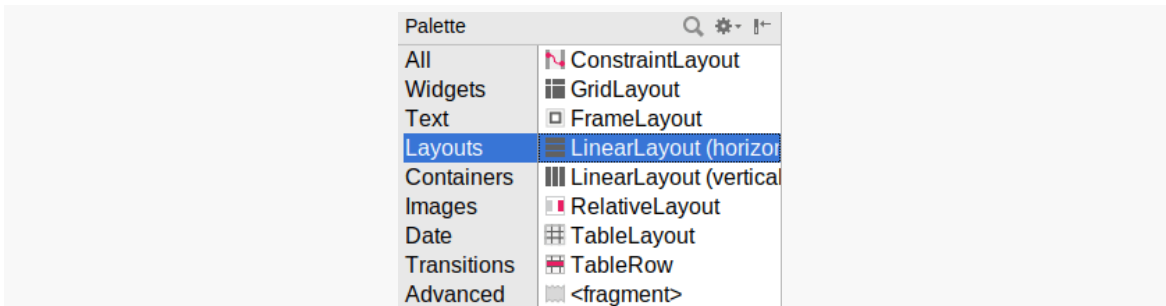
Figure 114: Layouts Palette in Android Studio Graphical Layout Editor
