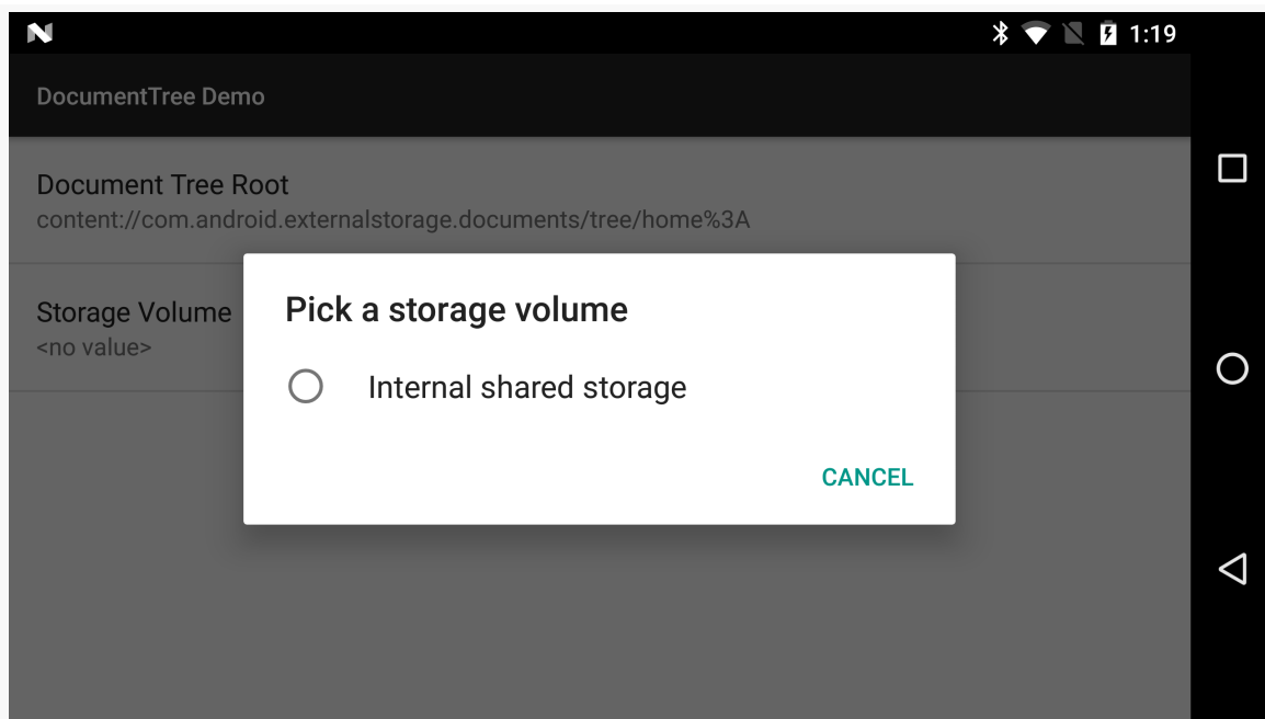
Figure 776: DocumentTree Demo, Showing Available Storage Volume(s)
