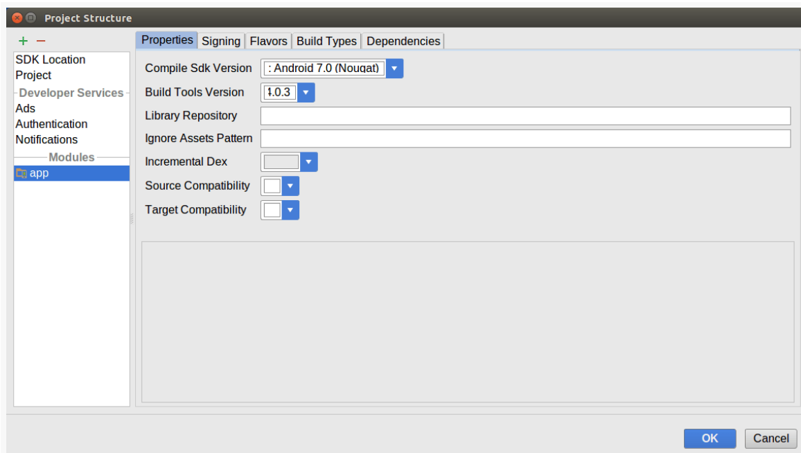
Figure 922: Project Structure Dialog, Module Category, Properties Tab
