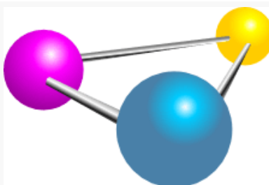
Figure 61: CommonsWare
