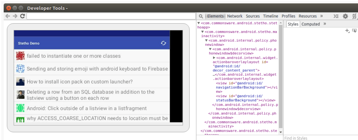
Figure 979: Stetho Screenshot
