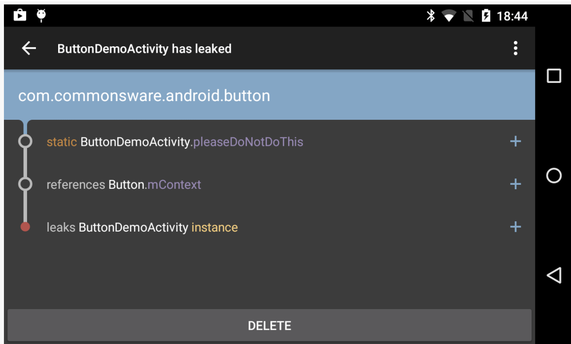
Figure 1042: LeakCanary Diagnostic Activity, As Launched From the Notification
