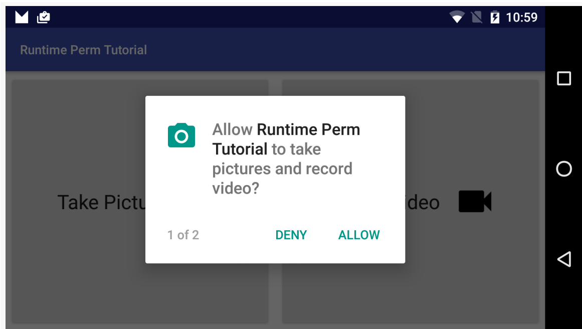
Figure 282: Tutorial App, Showing CAMERA Permission Request
