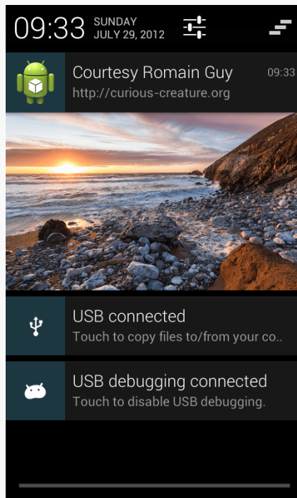
Figure 411: BigPicture Notification
