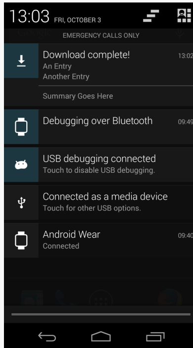
Figure 423: Stacked Notifications, Summary on Primary Device
