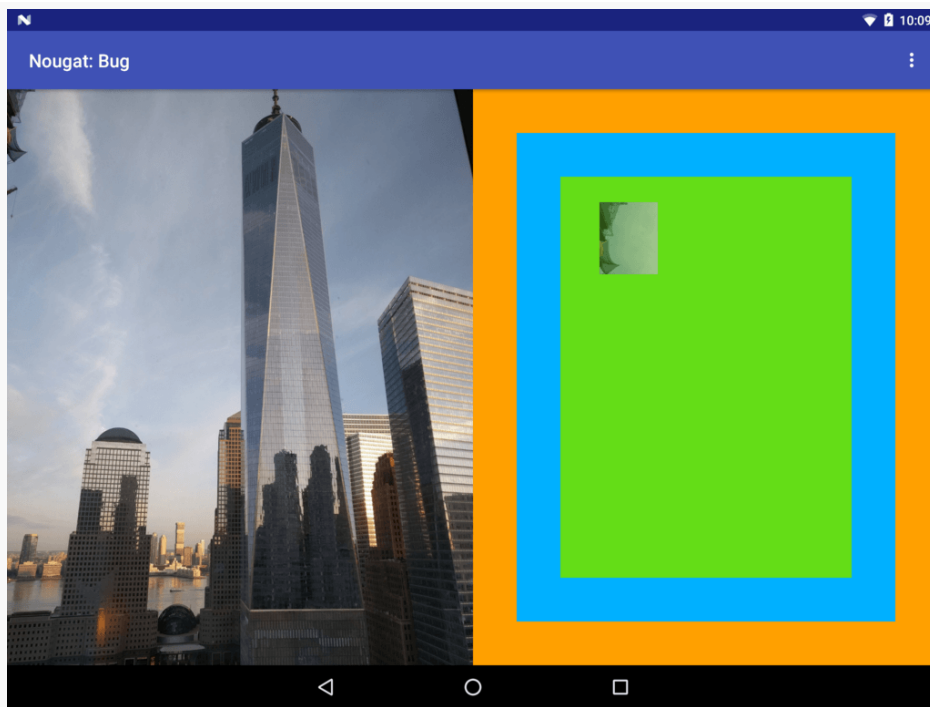
Figure 737: Dragging Over ImageView Drop Target on Android 7.0
