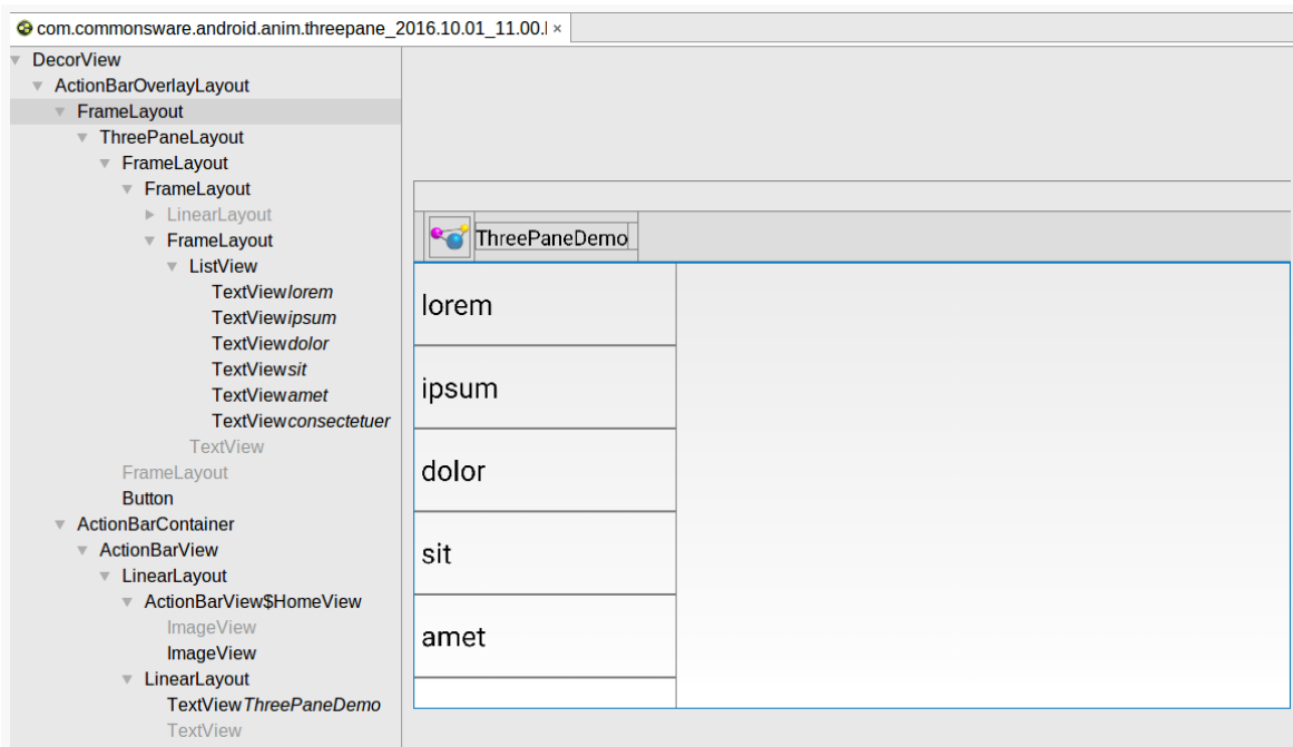
Figure 1009: Three-Pane Demo in Layout Inspector, Showing More Hierarchy
