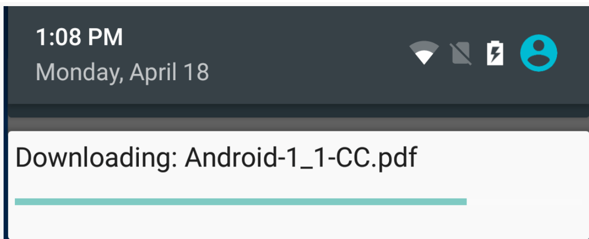
Figure 452: Custom Notification
