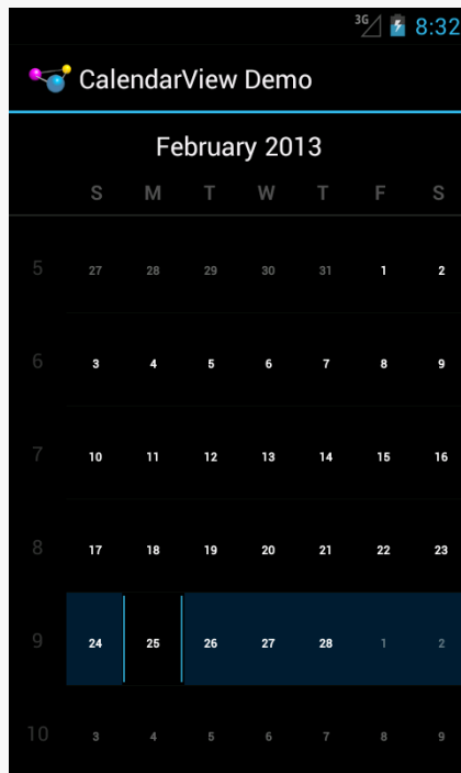
Figure 1076: Android 4.1
