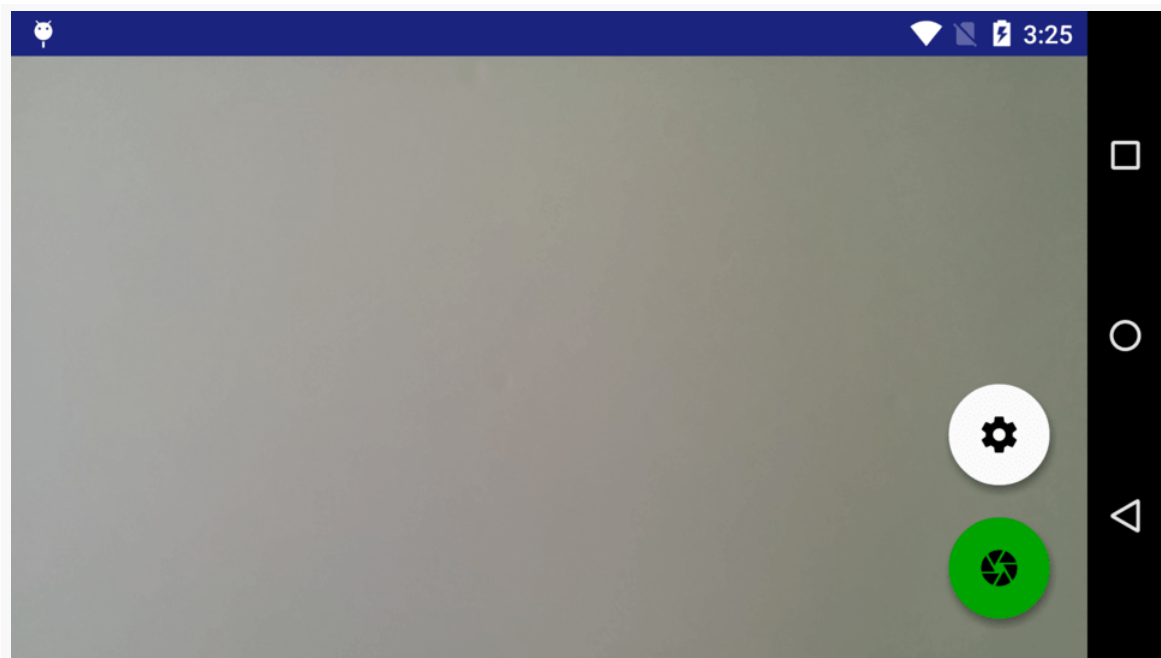
Figure 805: CWAC-Cam2 CameraActivity
