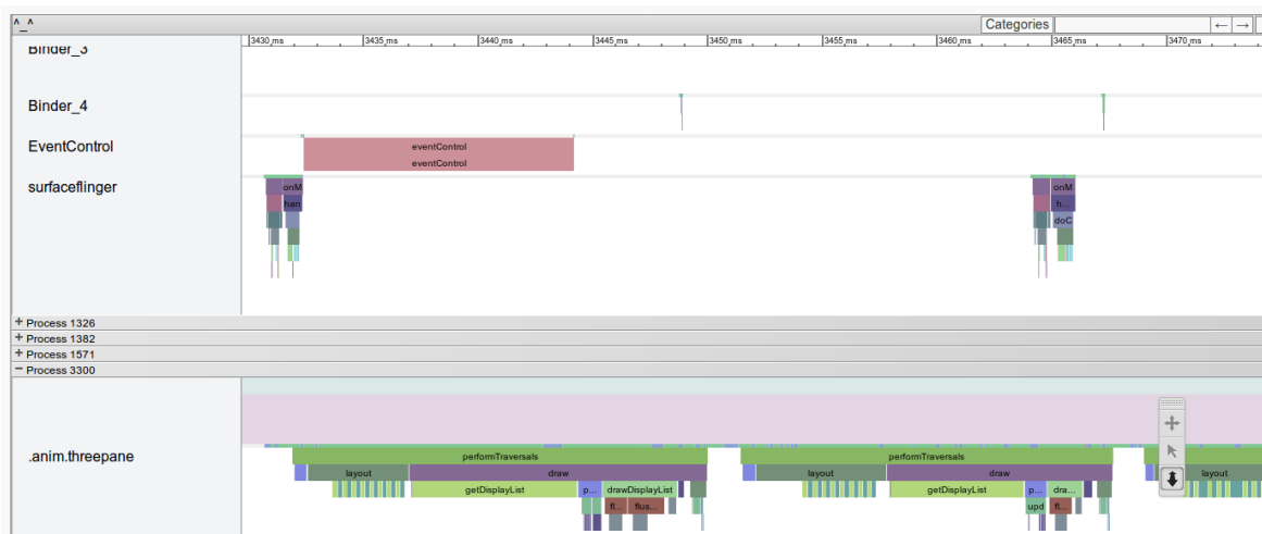
Figure 984: Systrace Output, Zoomed In on 40 Milliseconds of Profiling
