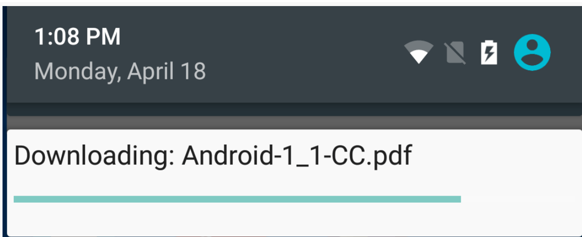
Figure 453: Custom Notification
