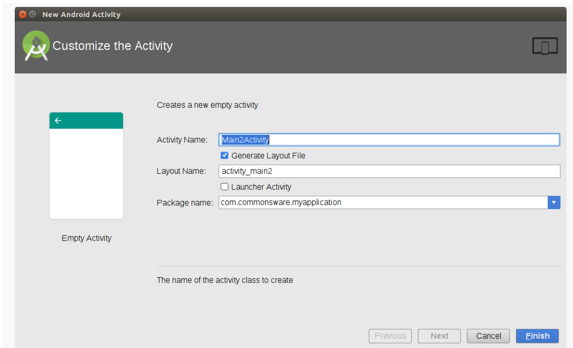
Figure 246: Android Studio New-Activity Wizard, Showing Empty Activity Template
