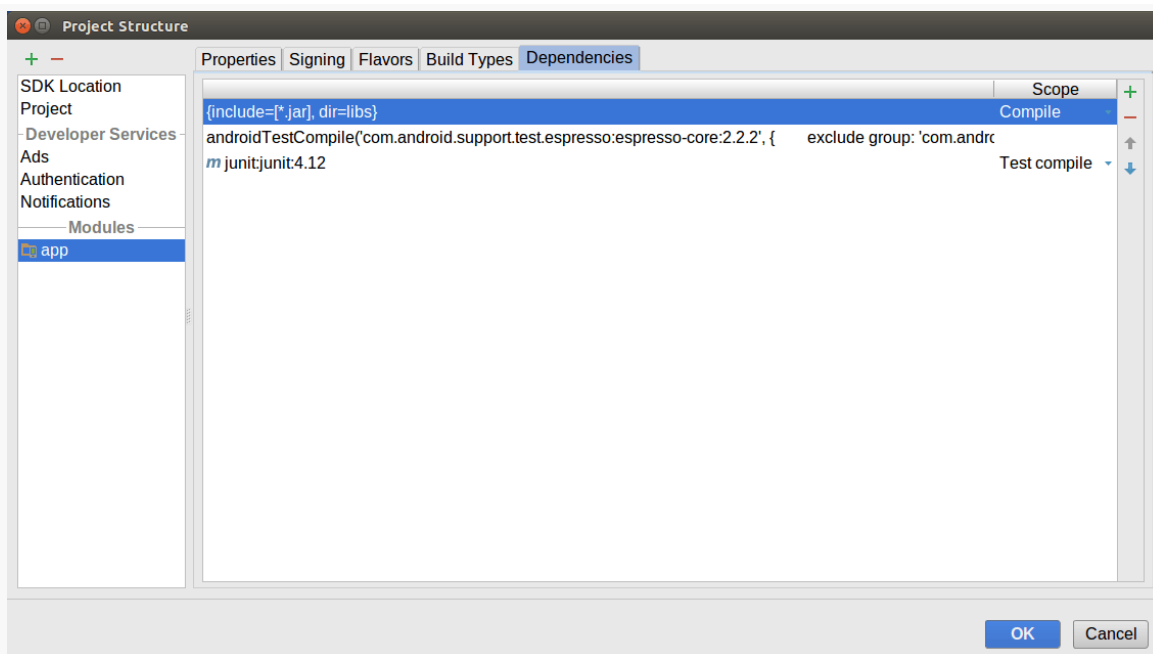
Figure 925: Project Structure Dialog, Module Category, Dependencies Tab
