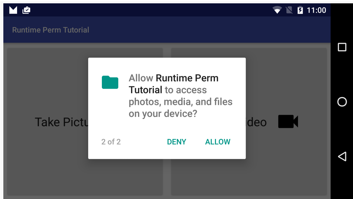
Figure 287: Tutorial App, Showing WRITE_EXTERNAL_STORAGE Permission Request
