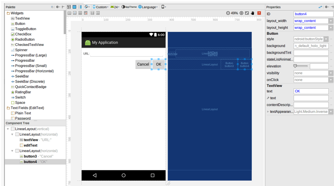
Figure 133: Buttons with Desired Captions
