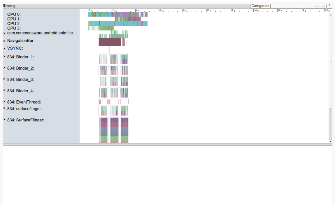
Figure 982: Systrace Output, As Initially Viewed
