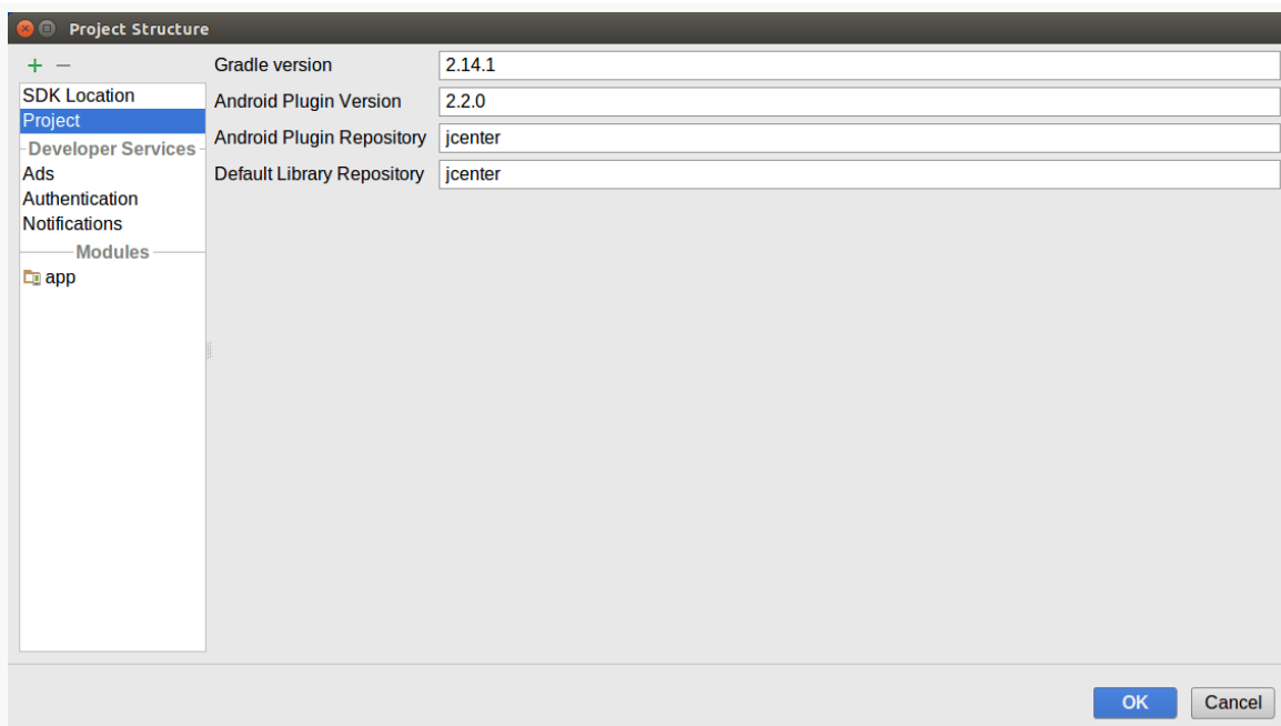
Figure 919: Project Structure Dialog, Project Settings Category
