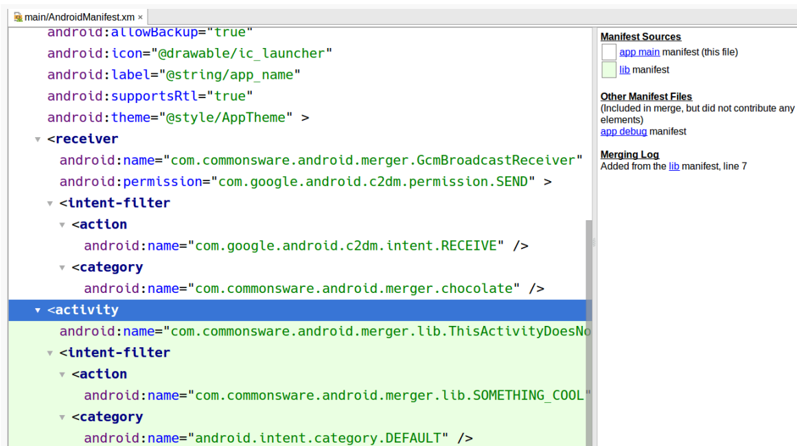
Figure 362: Merged Manifest View, Showing Merged Element
