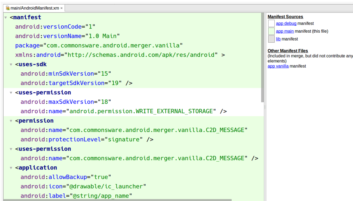
Figure 359: Merged Manifest Tab
