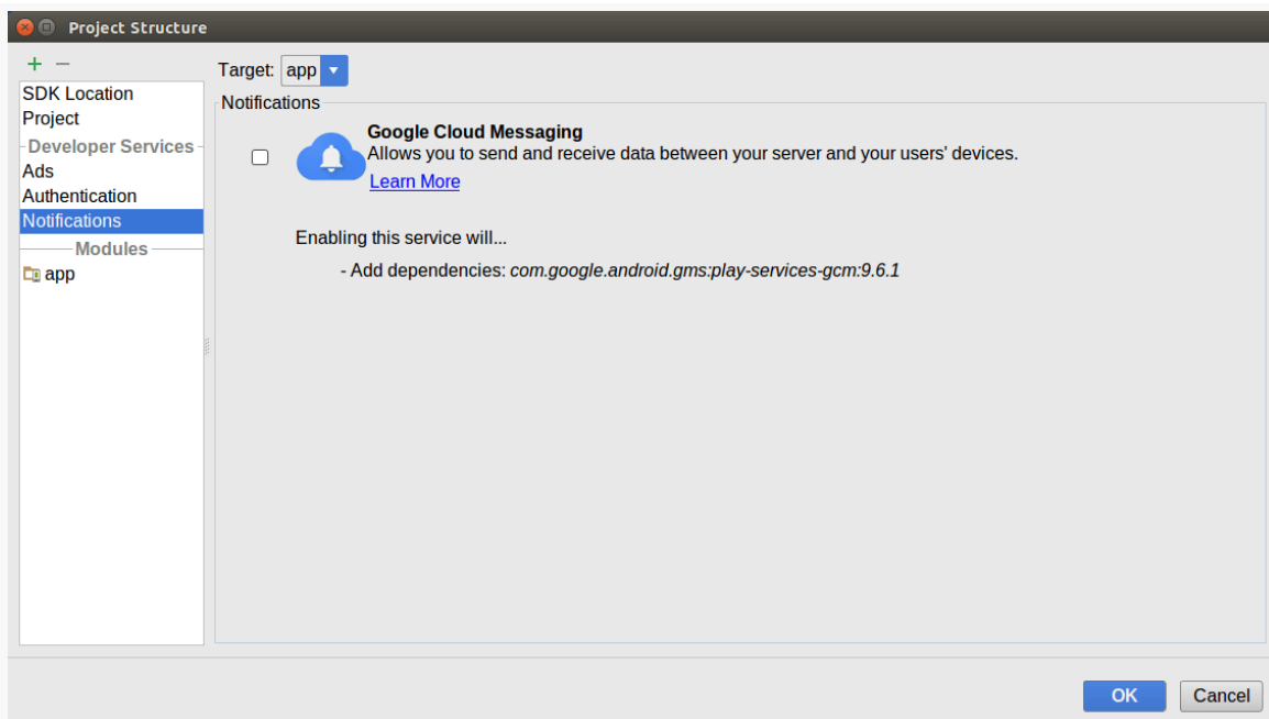
Figure 920: Project Structure Dialog, Notifications Category
