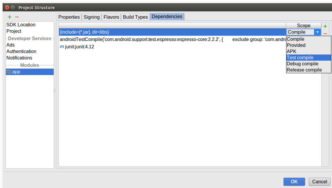
Figure 926: Dependencies Tab, Showing Scope Drop-Down
