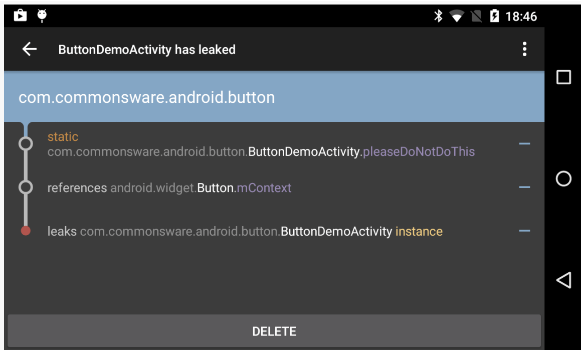
Figure 1028: LeakCanary Diagnostic Activity, Showing Full Package Names
