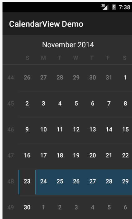
Figure 1062: Android 5.0
