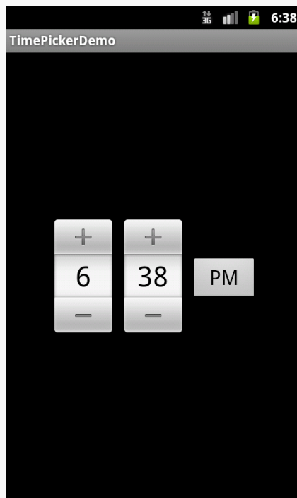
Figure 1081: Android 2.3.3
