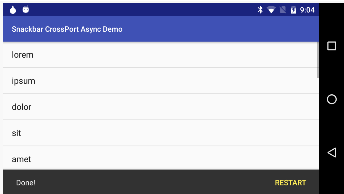
Figure 520: CWAC-CrossPort Snackbar
