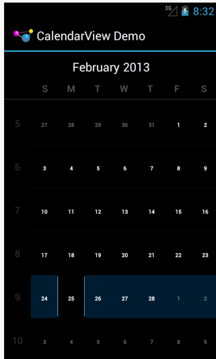
Figure 1061: Android 4.1
