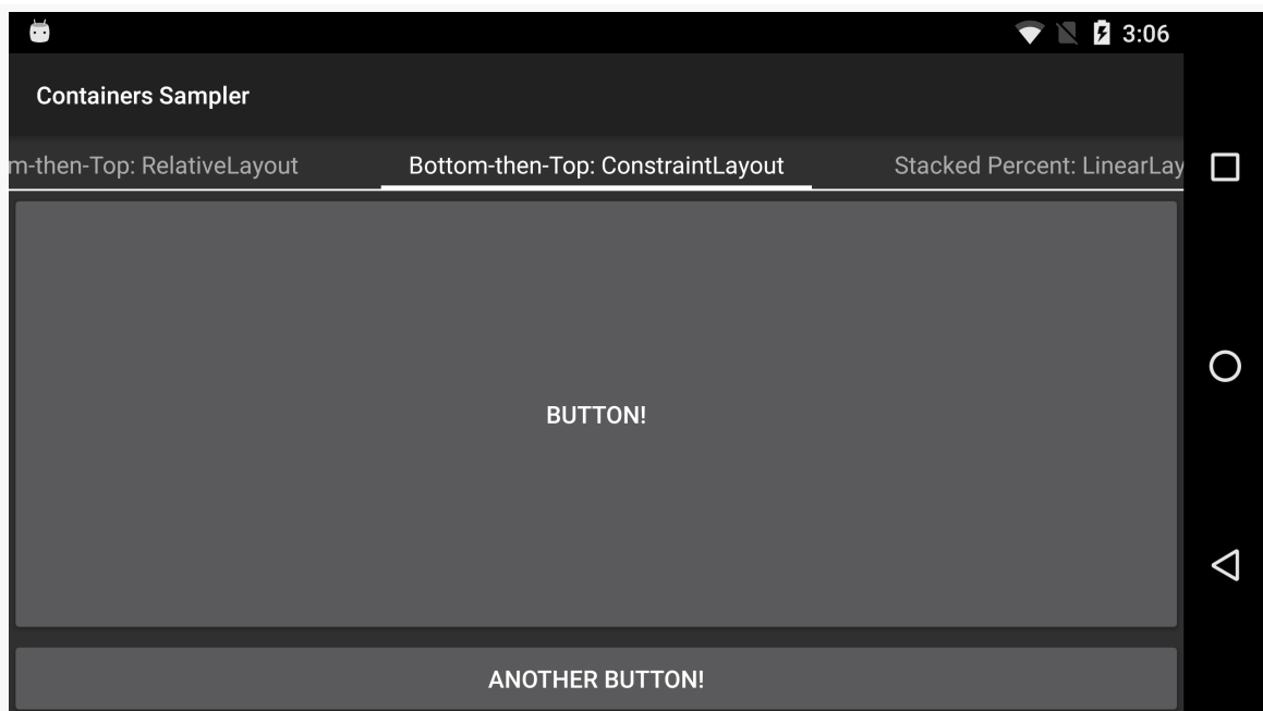
Figure 195: Bottom-then-Top Layout, Using ConstraintLayout
