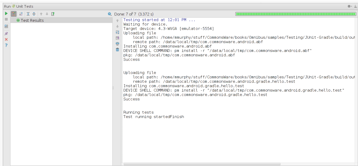
Figure 375: Android Studio, Showing Run Unit Tests Results
