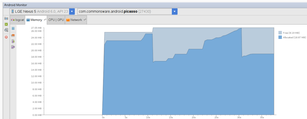
Figure 997: Android Studio, Android Monitor, Memory Tab
