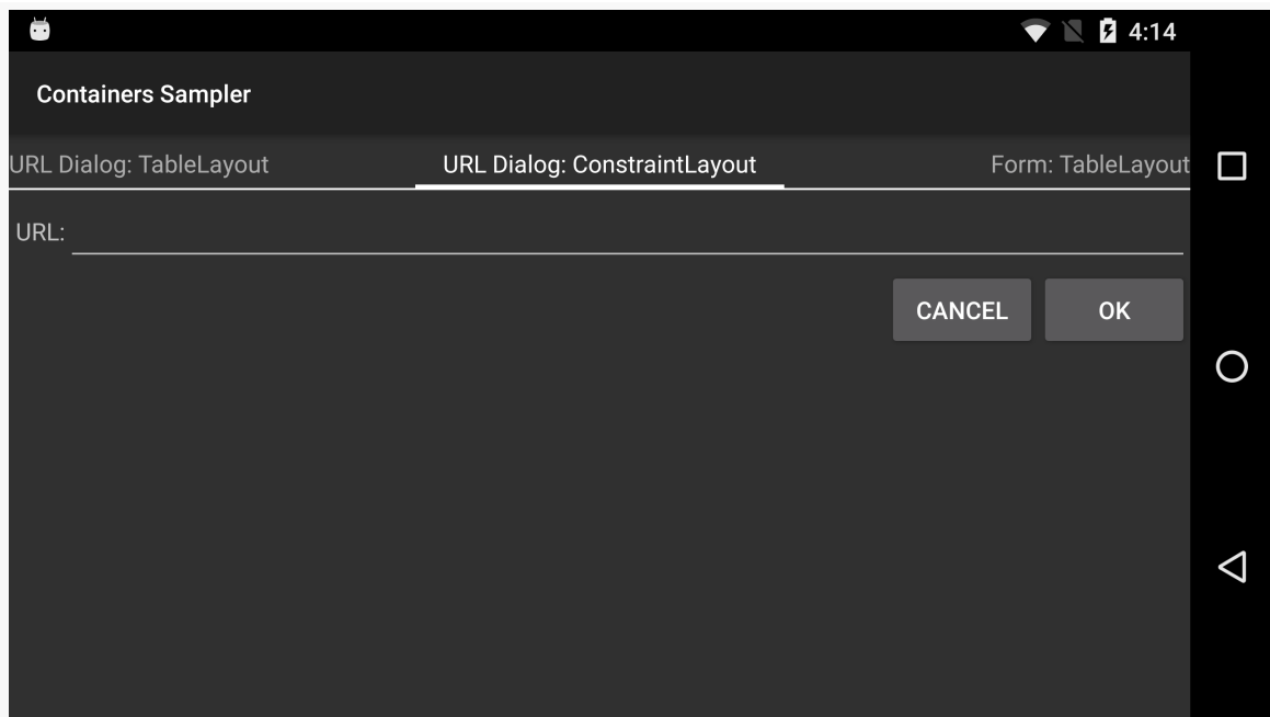
Figure 200: URL Dialog Layout, Using ConstraintLayout
