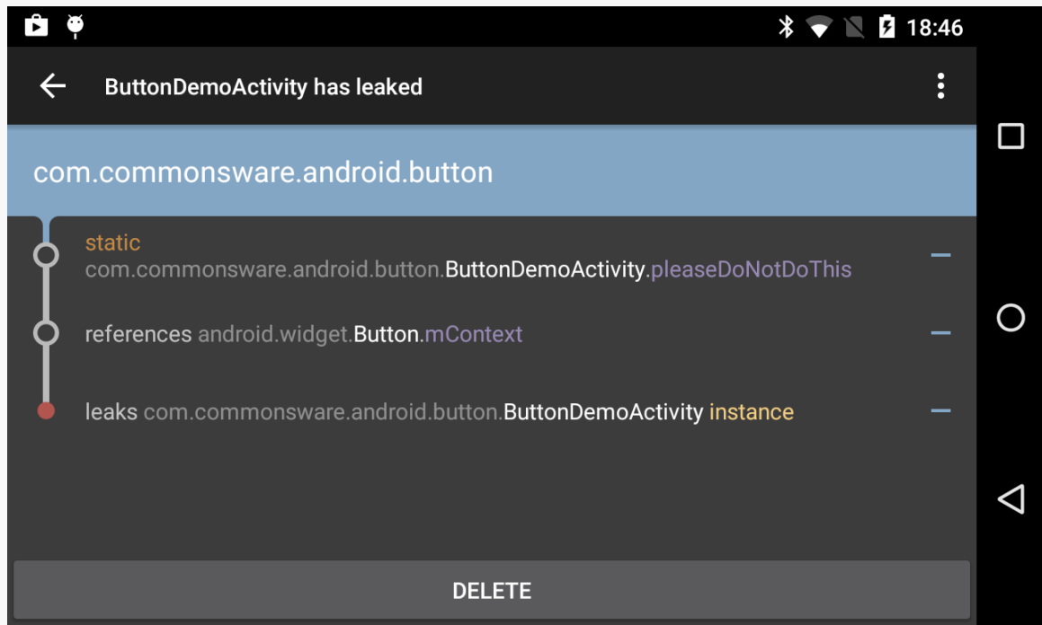
Figure 1017: LeakCanary Diagnostic Activity, Showing Full Package Names
