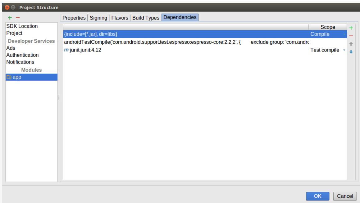
Figure 914: Project Structure Dialog, Module Category, Dependencies Tab
