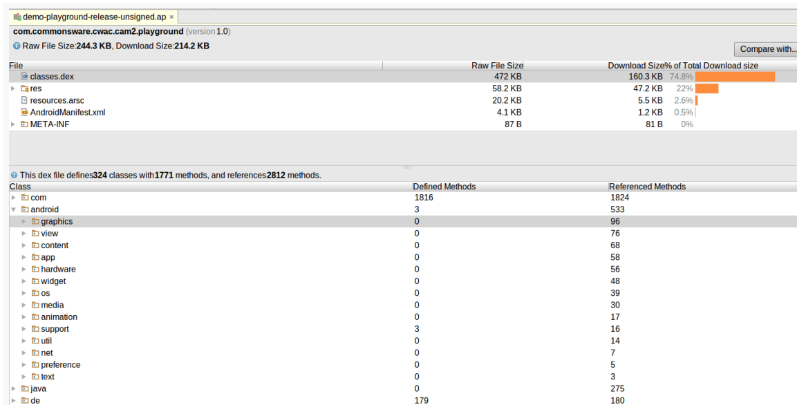
Figure 1039: APK Analyzer, Looking for Referenced Methods
