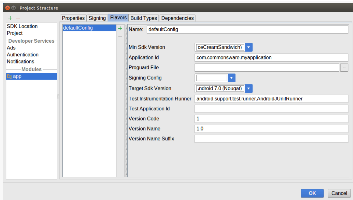
Figure 912: Project Structure Dialog, Module Category, Flavors Tab
