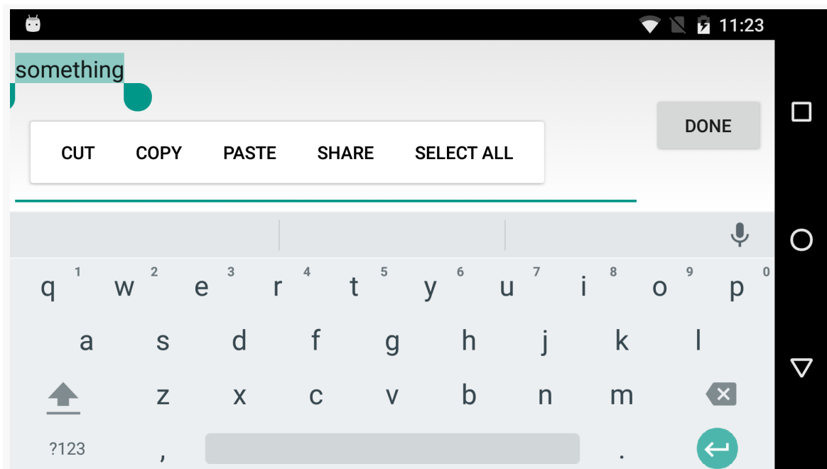
Figure 903: Landscape EditText, Sans ACTION_PROCESS_TEXT Options
