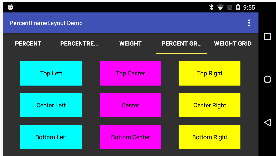
Figure 474: Percent Comparison Demo, Showing PercentFrameLayout Grid
