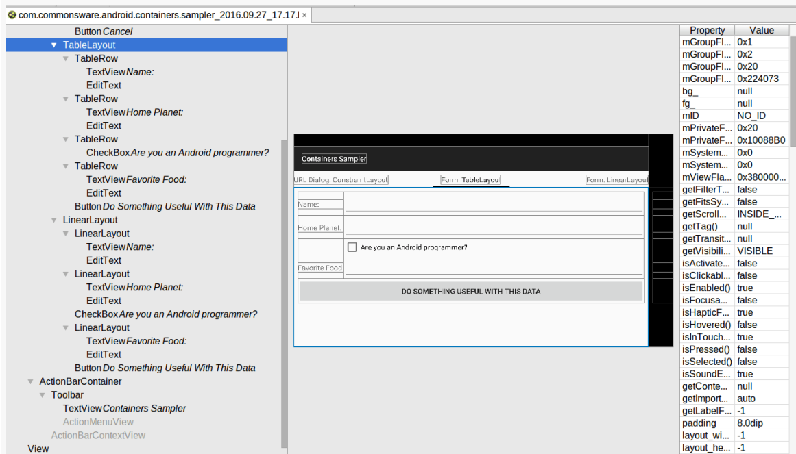
Figure 949: Layout Inspector, As Initially Launched
