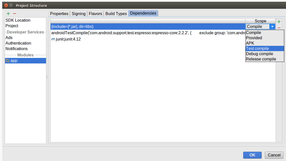
Figure 915: Dependencies Tab, Showing Scope Drop-Down
