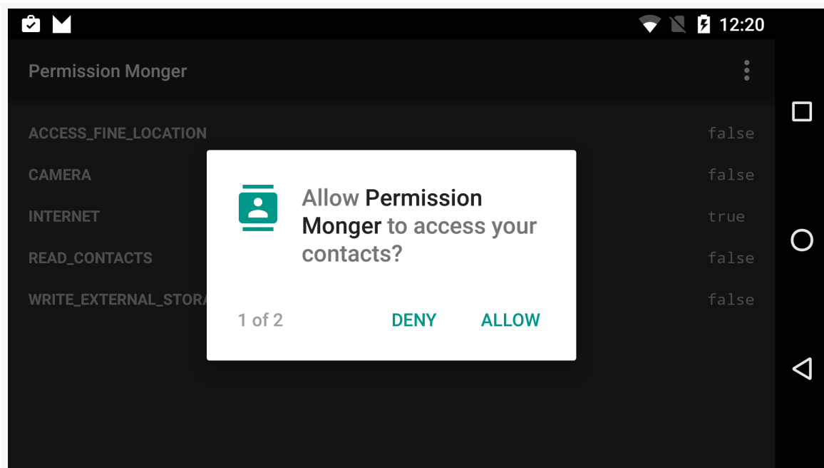
Figure 272: Permission Monger, Requesting READ_CONTACTS Permission
