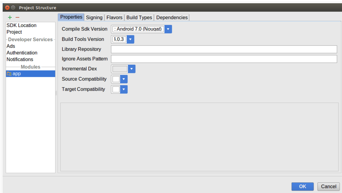
Figure 910: Project Structure Dialog, Module Category, Properties Tab
