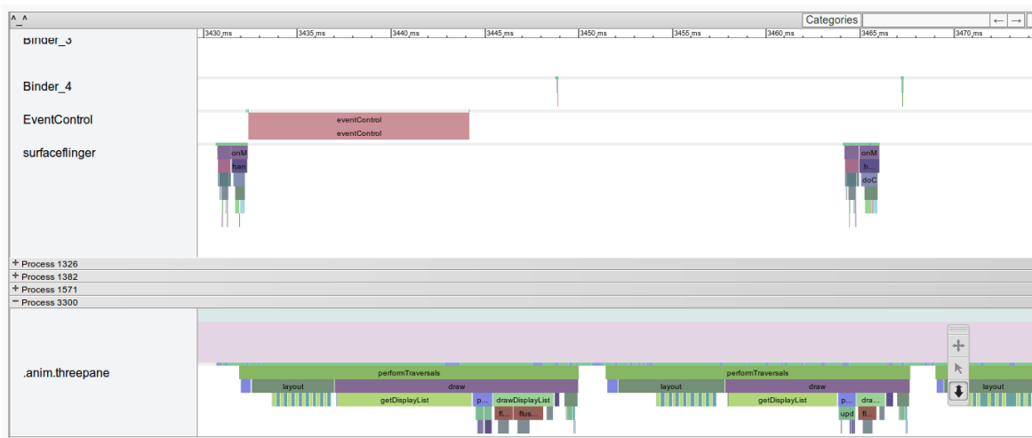
Figure 974: Systrace Output, Zoomed In on 40 Milliseconds of Profiling
