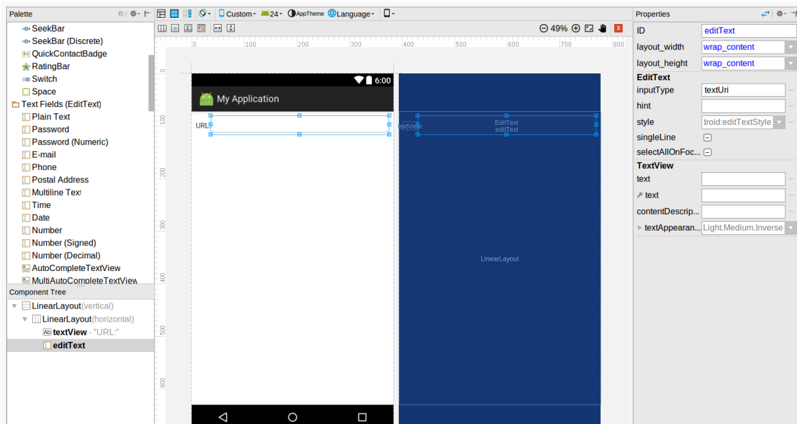
Figure 126: Horizontal LinearLayout with TextView and EditText
