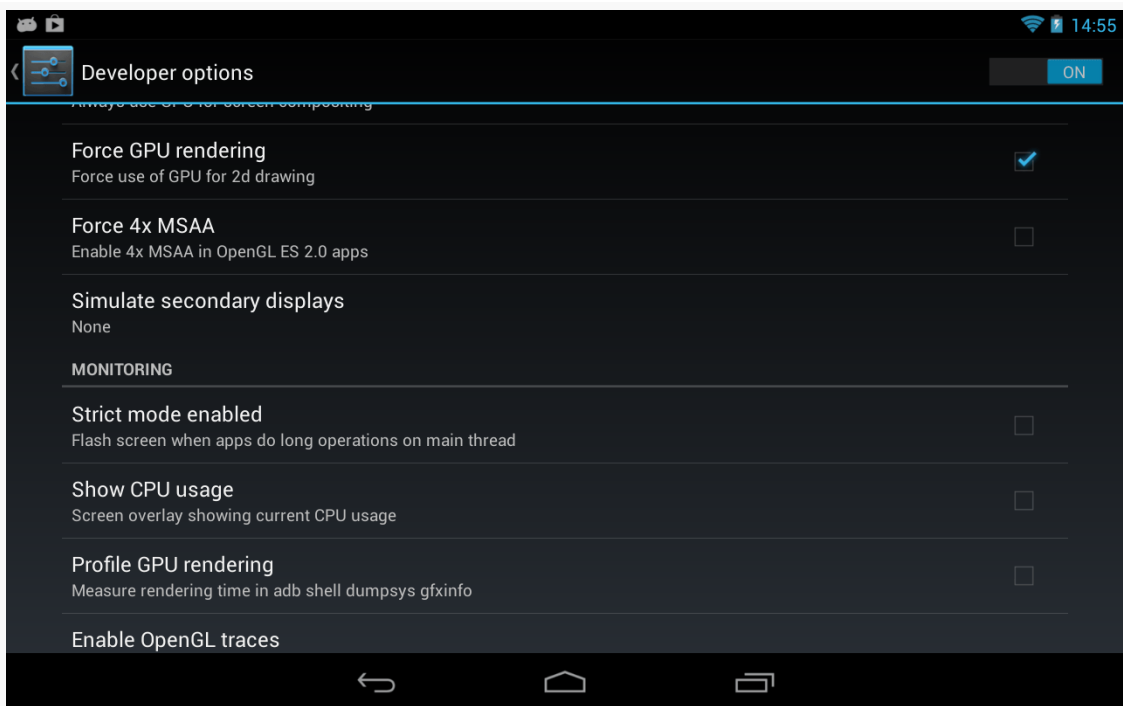
Figure 967: Developer Options, Showing “Force GPU rendering” and “Profile GPU rendering”
