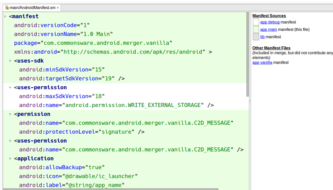
Figure 354: Merged Manifest Tab
