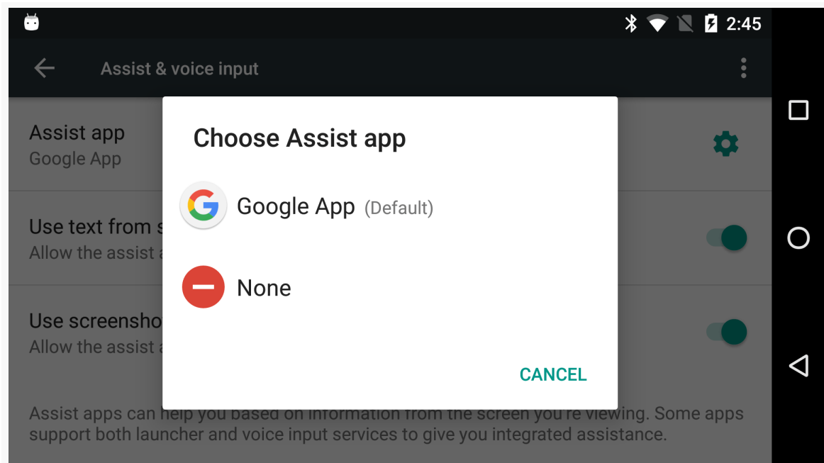
Figure 708: Android 6.0 Assist & Voice Input Options in Settings
