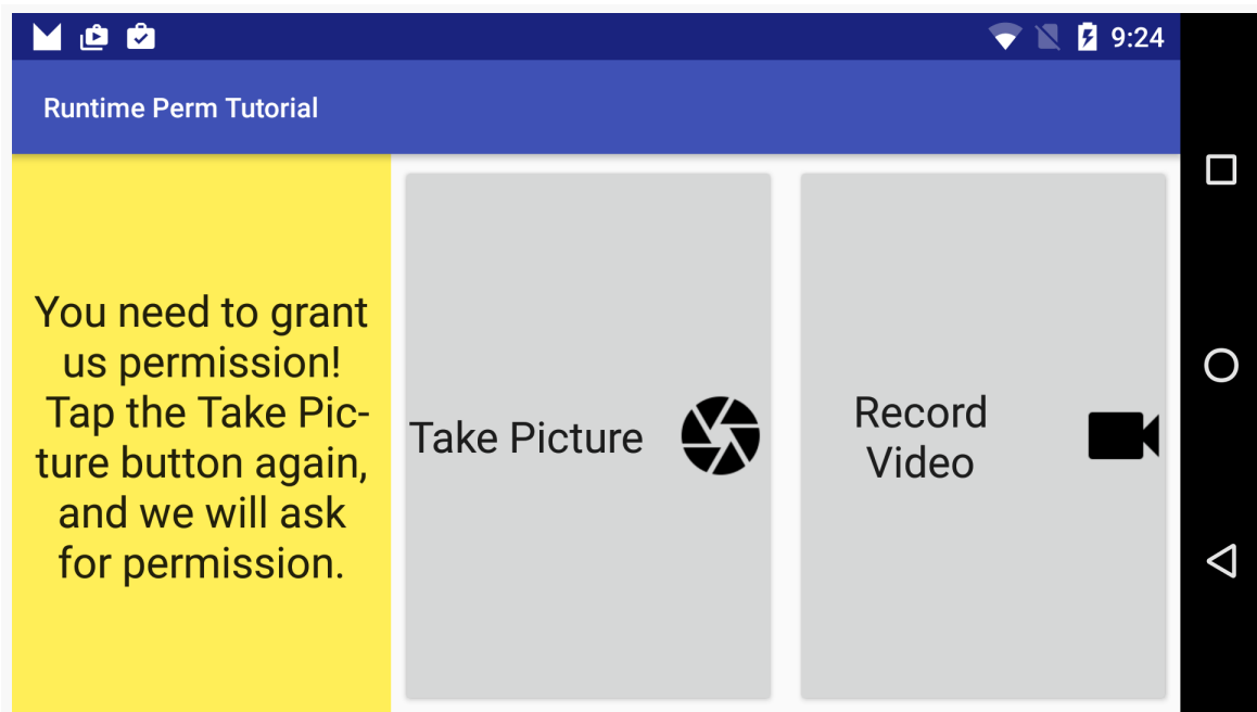
Figure 283: Tutorial App, Showing Breadcrumb
