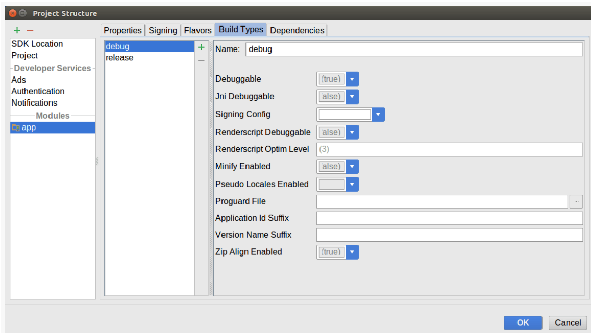
Figure 913: Project Structure Dialog, Module Category, Build Types Tab
