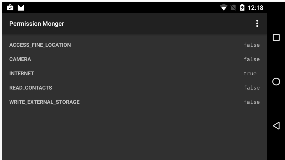
Figure 205: Permission Monger, Showing Initial Permissions
