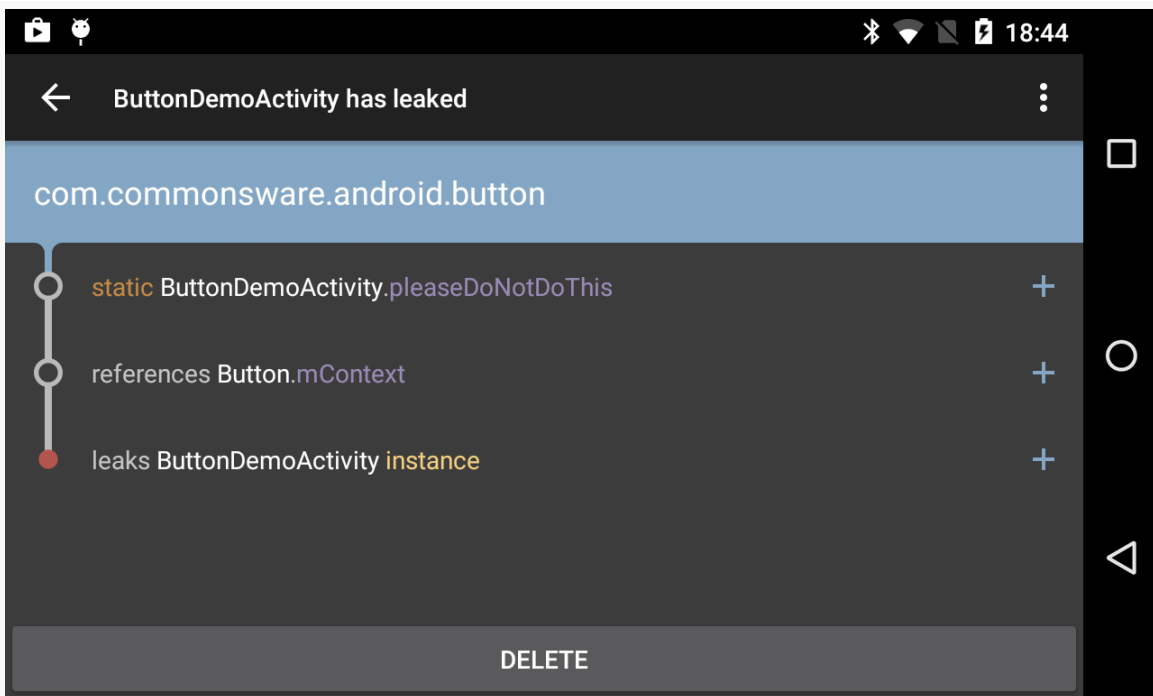
Figure 904: LeakCanary Diagnostic Activity, As Launched From the Notification
