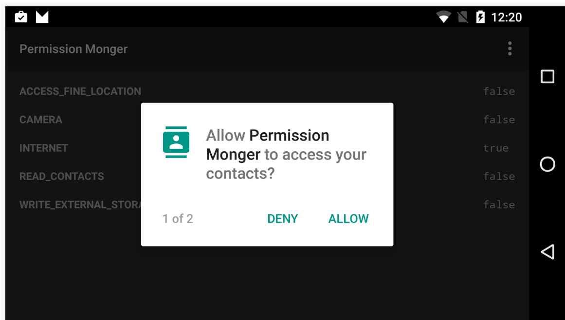
Figure 206: Permission Monger, Requesting READ_CONTACTS Permission
