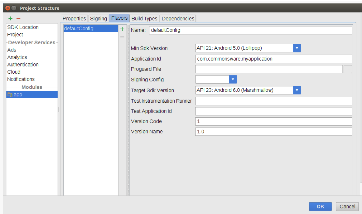
Figure 801: Project Structure Dialog, Module Category, Flavors Tab
