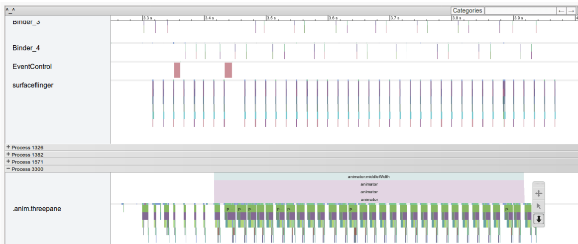
Figure 861: Systrace Output, Zoomed In on 0.7 Seconds of Profiling
