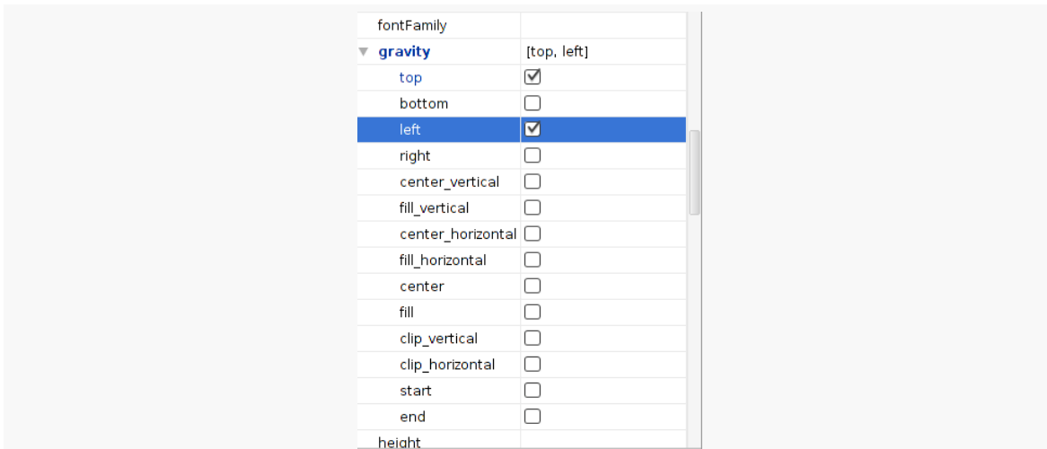
Figure 238: Android Studio Layout Editor Properties Pane, Showing Gravity Options
