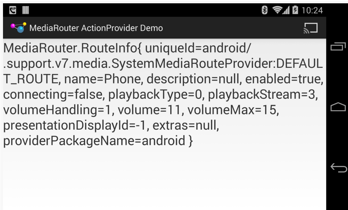
Figure 699: MediaRouter ActionProvider Demo, on a Nexus 4, Showing Default Route and Provider
