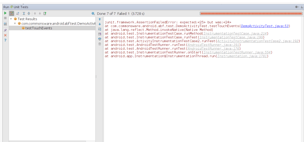
Figure 293: Android Studio, Showing Run Unit Tests Results With a Failure
