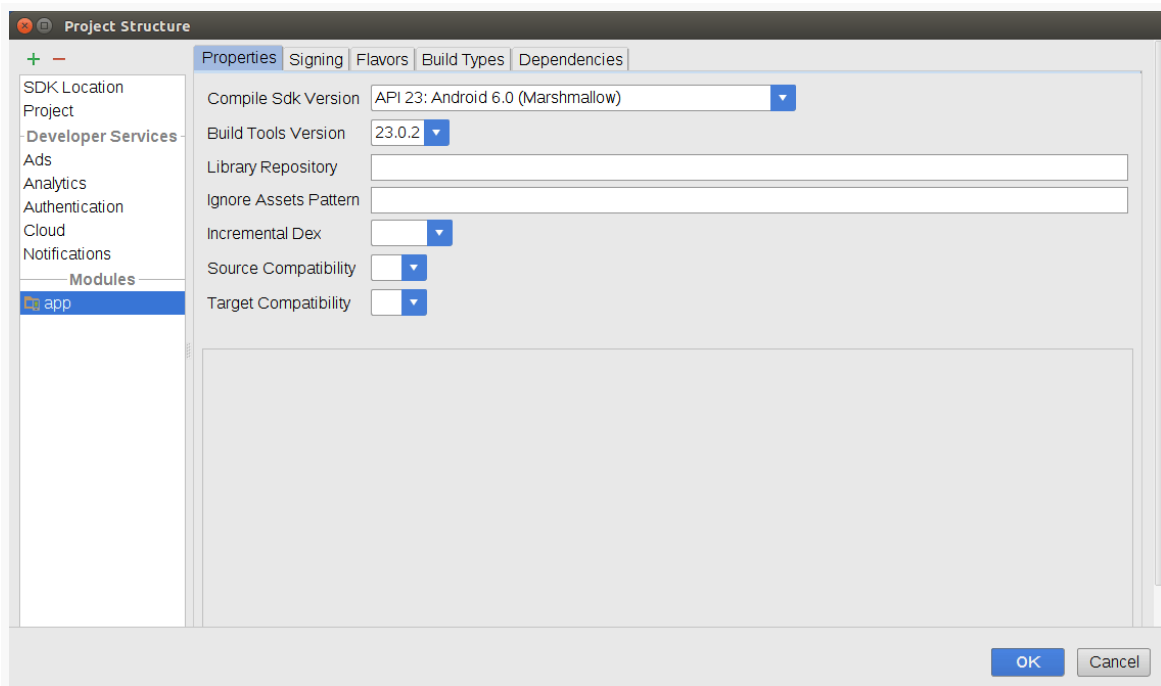
Figure 799: Project Structure Dialog, Module Category, Properties Tab
