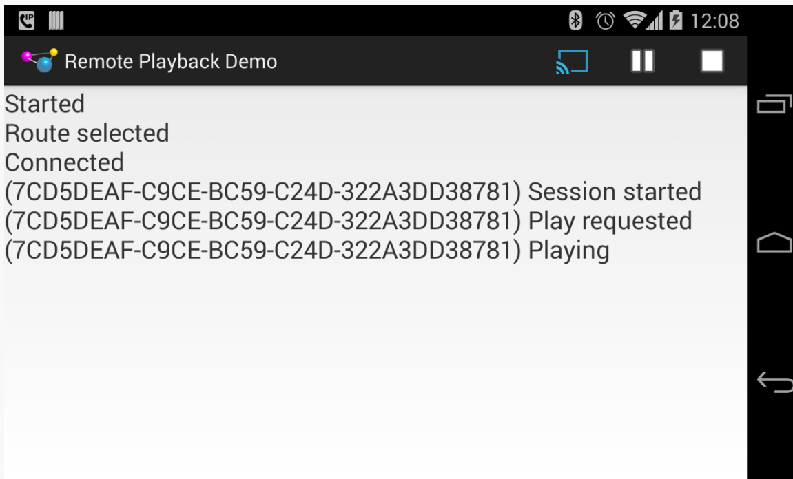
Figure 710: RemotePlaybackClient Demo, on a Nexus 4, After Playback Has Started
