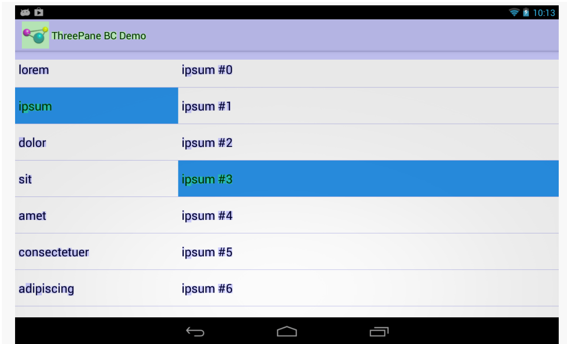
Figure 868: Three-Pane Demo, Left and Middle Panes Via BACK, Showing Overdraw
