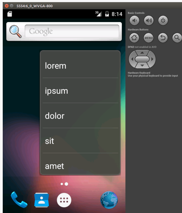
Figure 645: Resized LoremWidget on Android Home Screen
