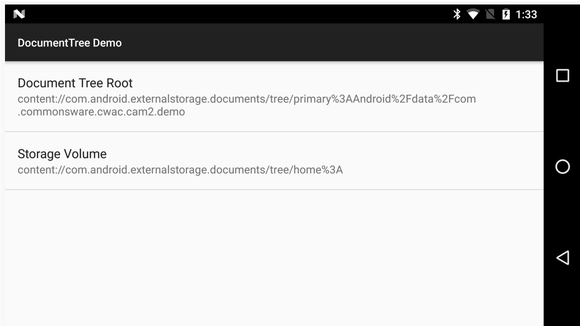
Figure 665: DocumentTree Demo, Showing Selected Storage Volume Directory
