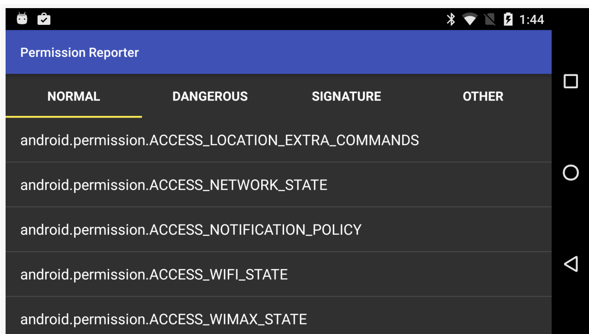
Figure 735: PermissionReporter, Normal Tab, on Android 6.0
