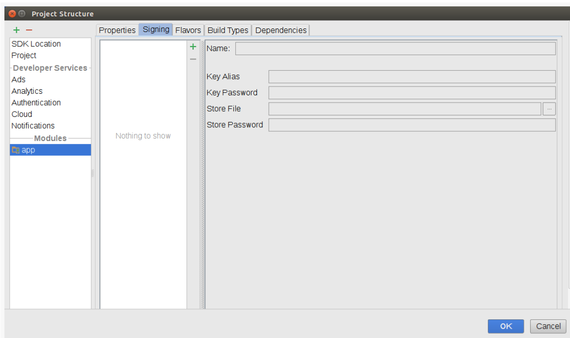
Figure 800: Project Structure Dialog, Module Category, Signing Tab
