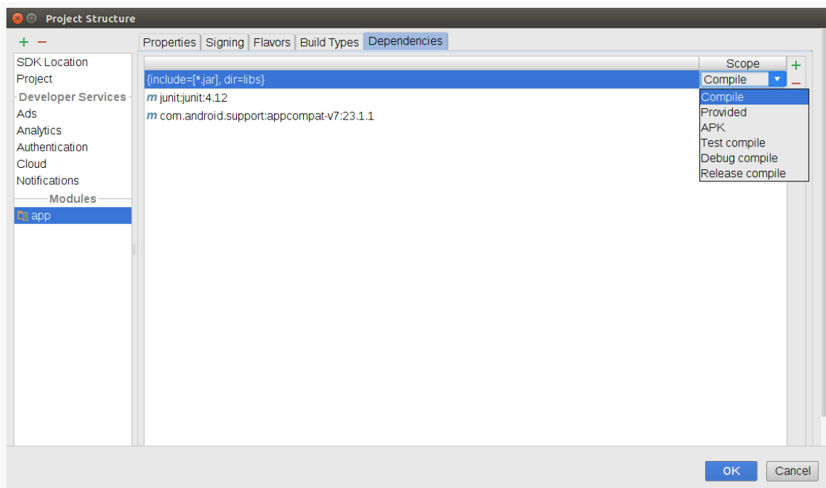
Figure 8o4: Dependencies Tab, Showing Scope Drop-Down
