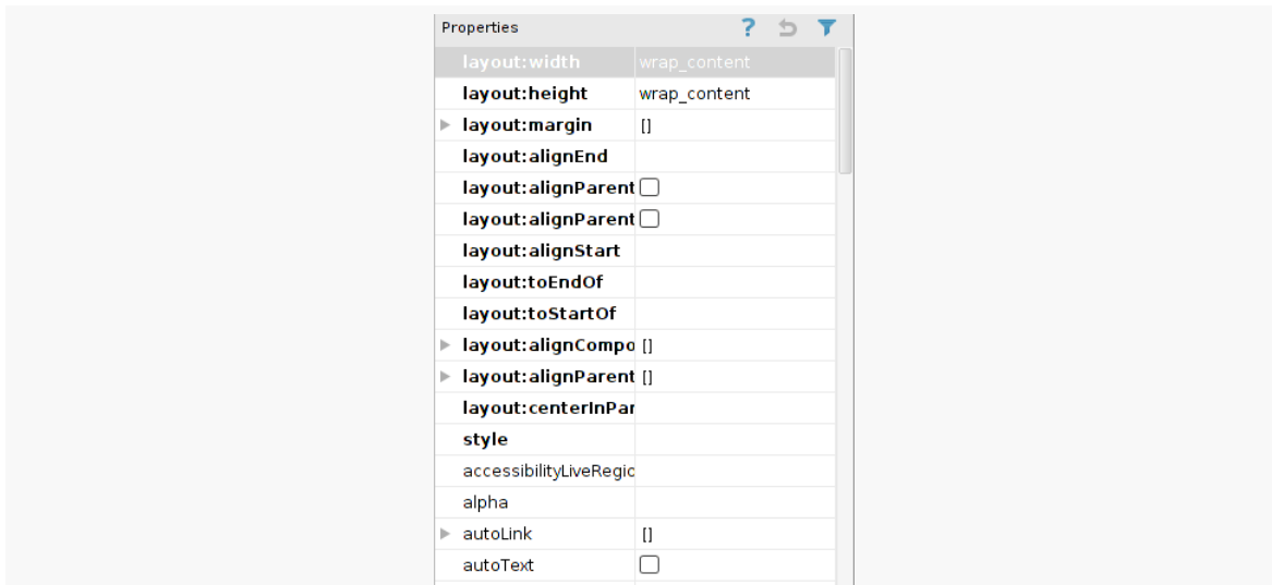
Figure 71: Properties Pane, for a TextView Inside a RelativeLayout
