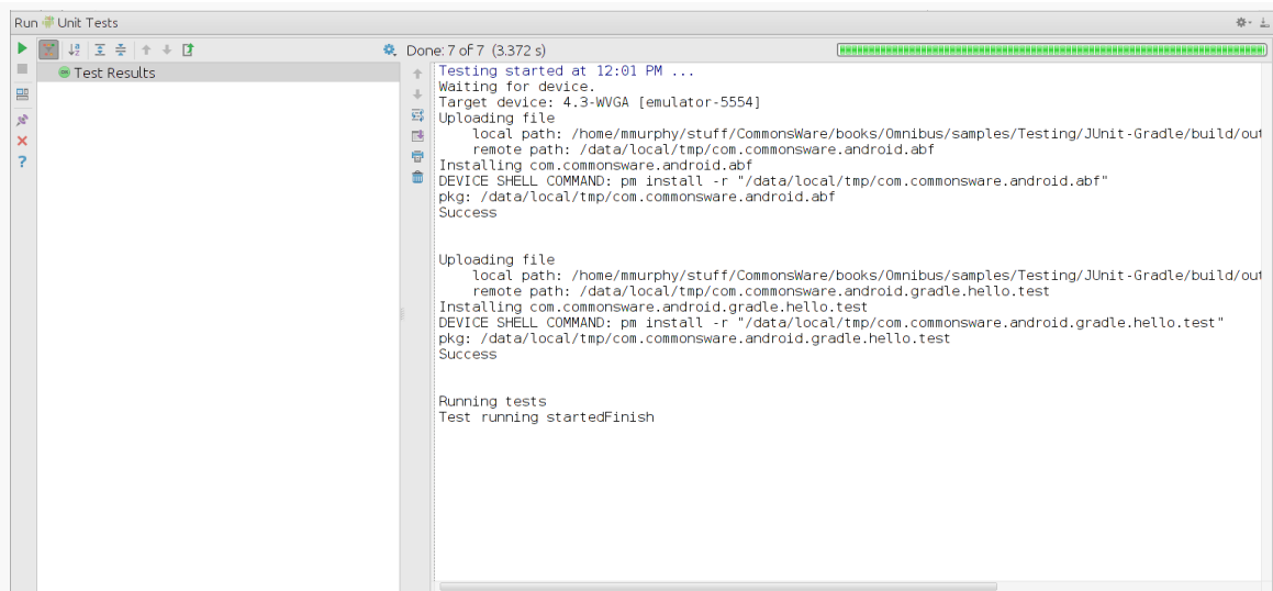
Figure 292: Android Studio, Showing Run Unit Tests Results
