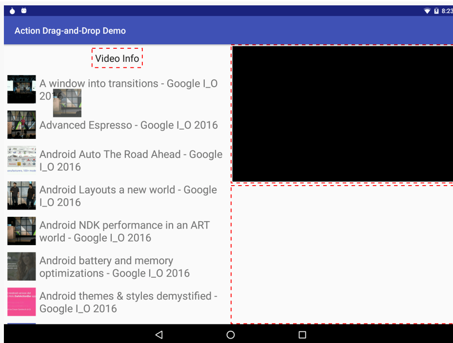
Figure 629: Drag-And-Drop, Showing Special Drop Target
