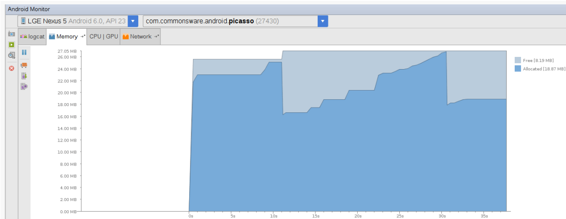
Figure 885: Android Studio, Android Monitor, Memory Tab
