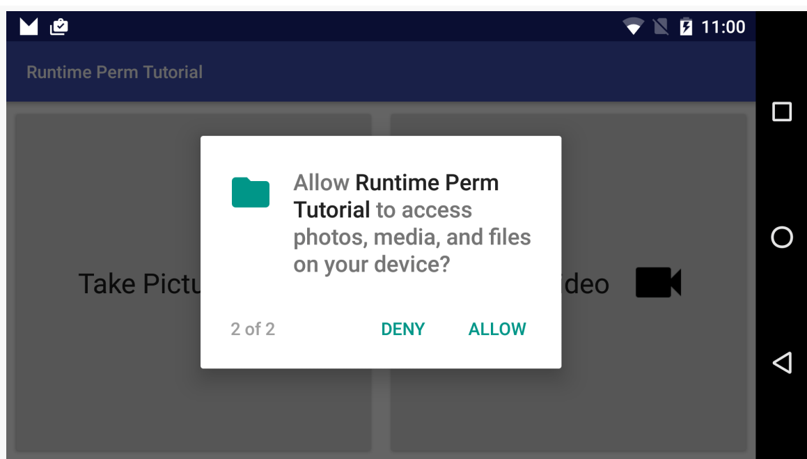
Figure 217: Tutorial App, Showing WRITE_EXTERNAL_STORAGE Permission Request
