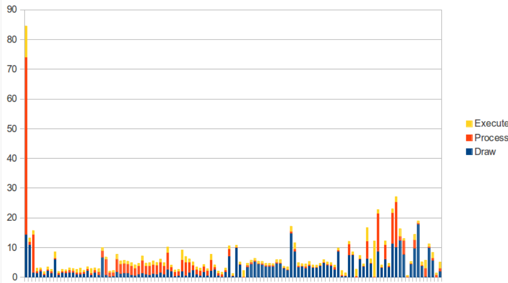
Figure 846: gfxinfo Output, In Stacked Column Chart
