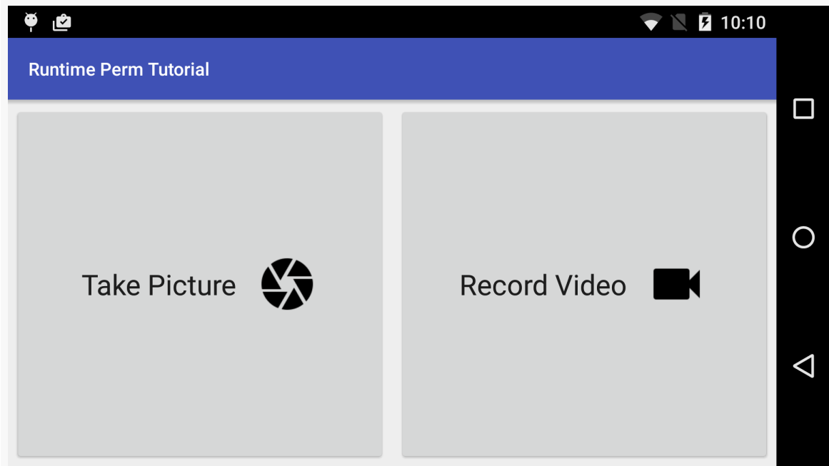
Figure 211: Runtime Permissions Tutorial App, As Initially Written and Launched
