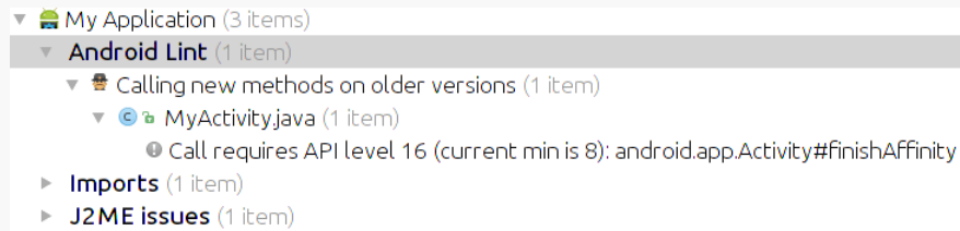
Figure 825: Android Studio Inspection Results
