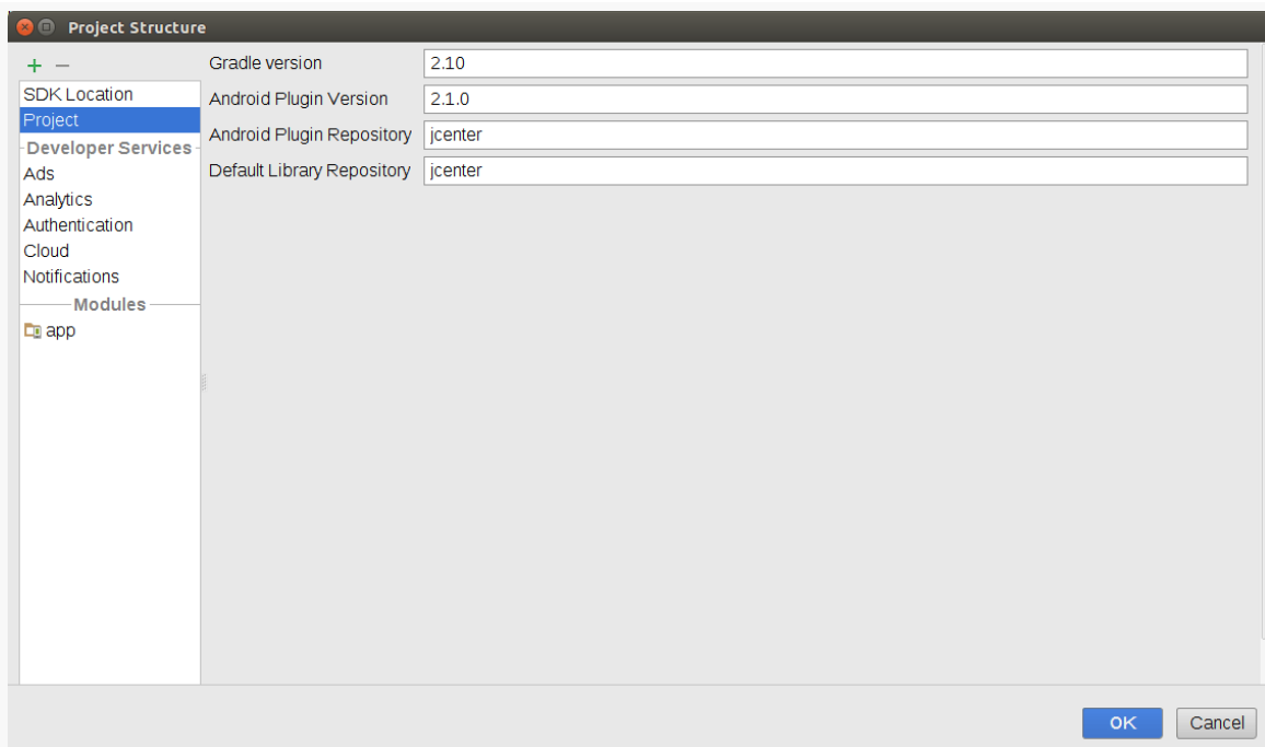
Figure 793: Project Structure Dialog, Project Settings Category
