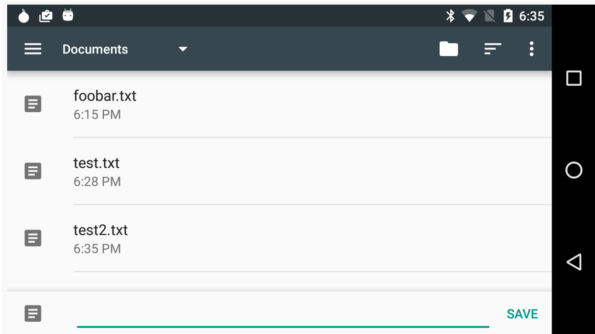
Figure 654: Storage Access Framework Create-Document Activity
