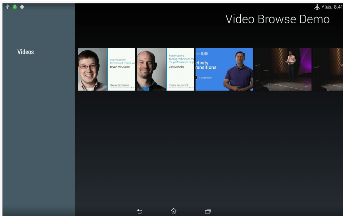
Figure 717: VideoBrowse Sample App, As Initially Launched
