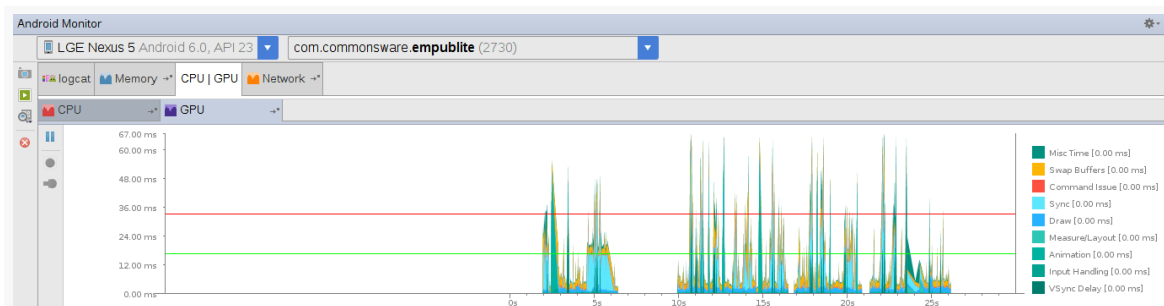
Figure 844: Android Studio, Android Monitor, CPU|GPU Tab, GPU Sub-Tab
