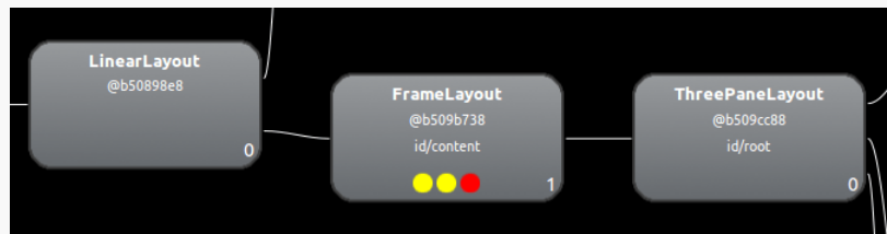
Figure 866: Single-Child FrameLayout in Three-Pane Demo, from Hierarchy View
