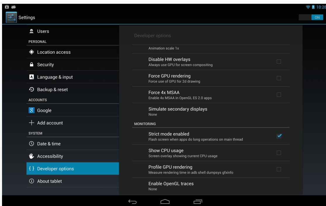
Figure 708: Nexus 10 “Simulate secondary displays” Preference
