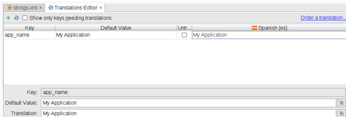
Figure 8o8: Translations Editor, Showing Spanish Translation
