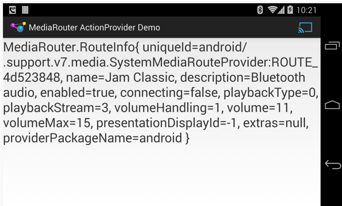
Figure 693: MediaRouter ActionProvider Demo, on a Nexus 4, Showing Live Audio Route
