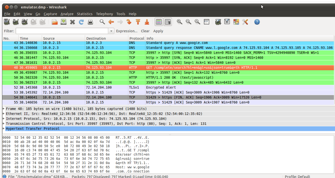
Figure 875: Wireshark examining captured emulator packets
