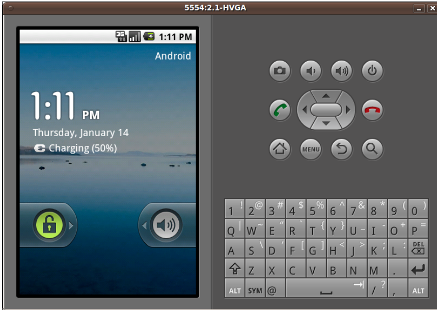
Figure 3. Android emulator
