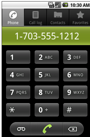
Figure 63. The Dialer
