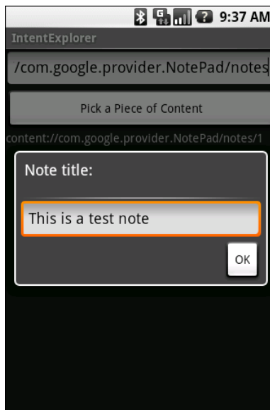
Figure 61. Notepad's edit-title dialog, shown over the IntentExplorer UI
