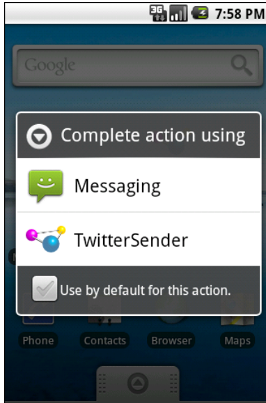
Figure 100. The ACTION_SEND request, as triggered by the shortcut
