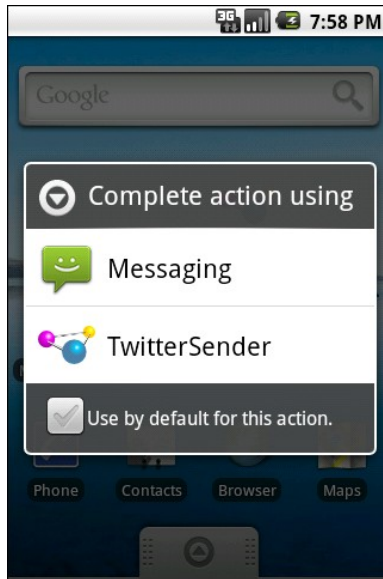
Figure 91. The ACTION_SEND request, as triggered by the shortcut
