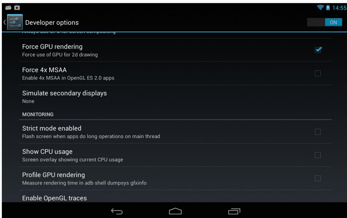
Figure 772: Developer Options, Showing “Force GPU rendering” and “Profile GPU rendering”
