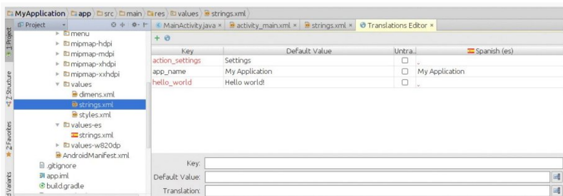
Figure 737: Spanish Strings in Resource File and Translations Editor
