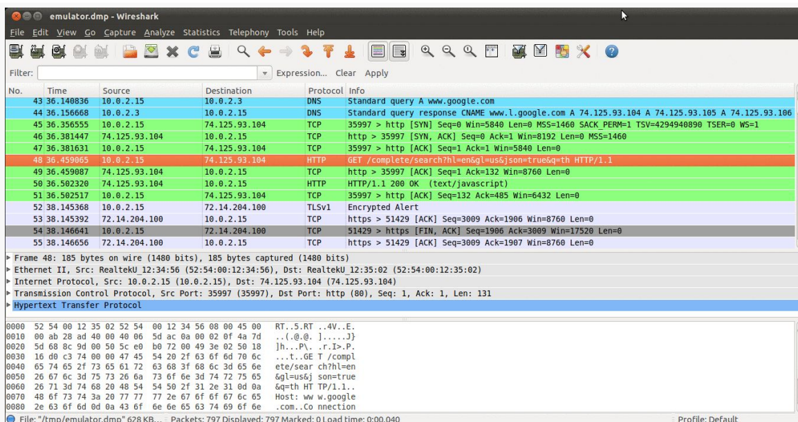
Figure 793: Wireshark examining captured emulator packets
