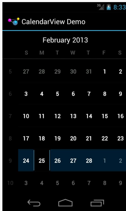
Figure 860: Android 4.0
