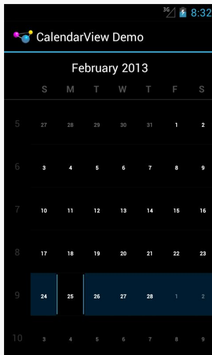
Figure 861: Android 4.1
