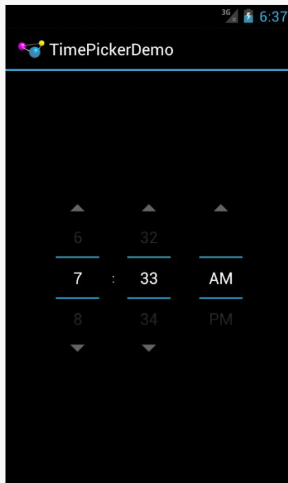
Figure 878: Android 4.0.3
