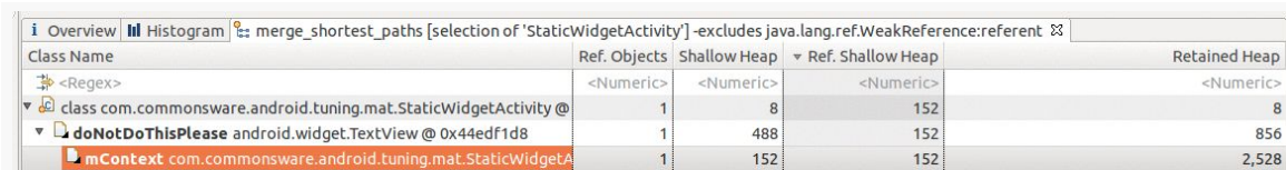
Figure 8o8: The GC roots holding onto an activity
