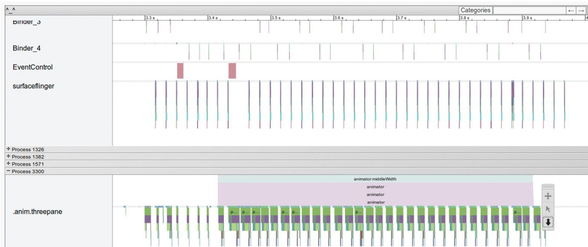
Figure 778: Systrace Output, Zoomed In on 0.7 Seconds of Profiling
