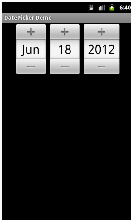
Figure 862: Android 2.3.3
