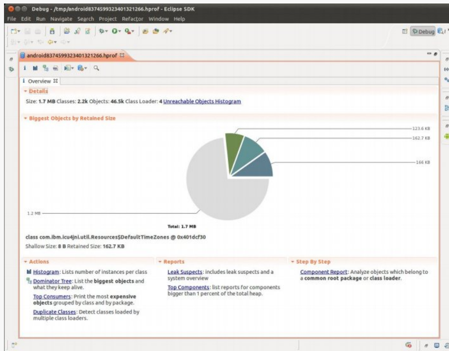
Figure 803: The Overview tool inside the MAT Eclipse perspective
