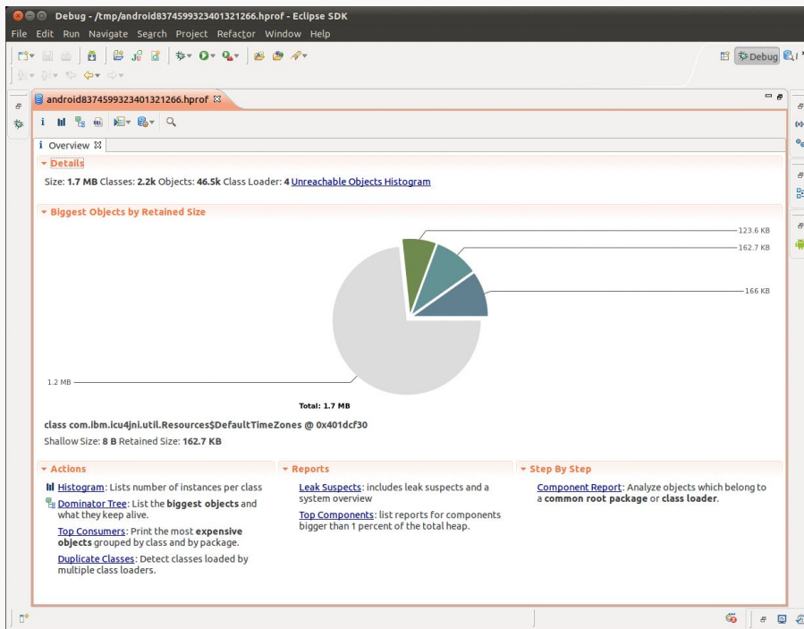
Figure 799: The Overview tool inside the MAT Eclipse perspective
