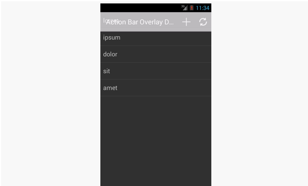
Figure 392: AppCompatActivity with FEATURE_ACTION_BAR_OVERLAY on an Android 4.3 Emulator
