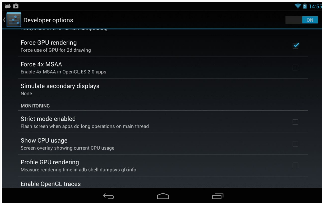
Figure 768: Developer Options, Showing “Force GPU rendering” and “Profile GPU rendering”
