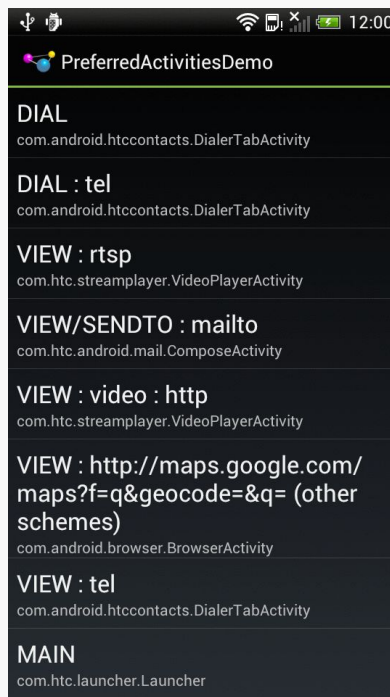
Figure 703: Preferred Activities on a Stock HTC One S
