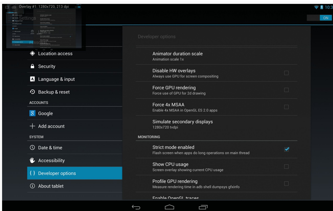
Figure 649: Nexus 10, Simulating a 720p external display
