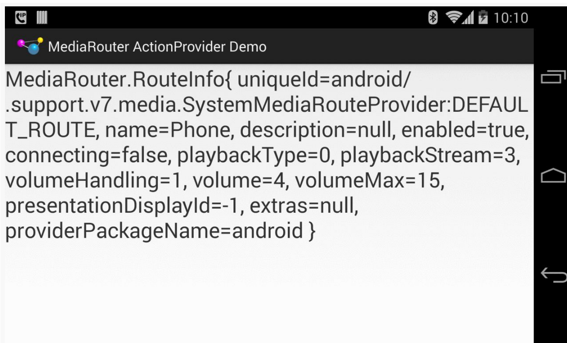
Figure 631: MediaRouter ActionProvider Demo, on a Nexus 4, Showing Default Route
