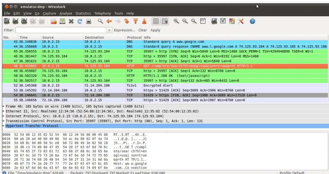
Figure 789: Wireshark examining captured emulator packets
