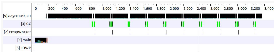
Figure 761: Zoomed in look at the TraceView thread timelines
