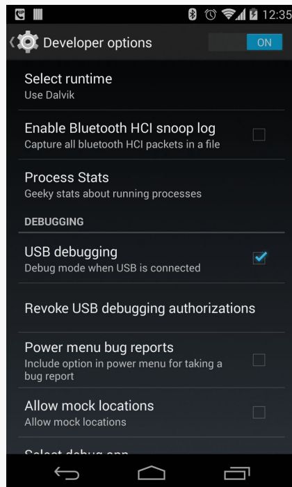
Figure 813: Developer Options in Android 4.4, Showing “Process Stats”
