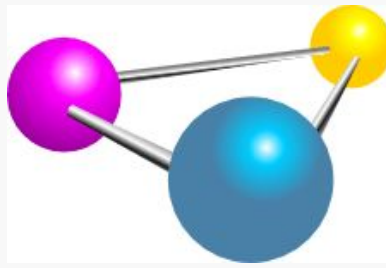
Figure 83: CommonsWare
