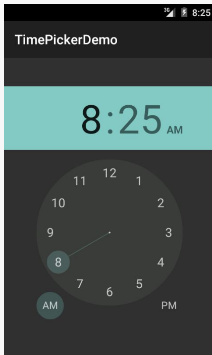
Figure 839: Android 5.0
