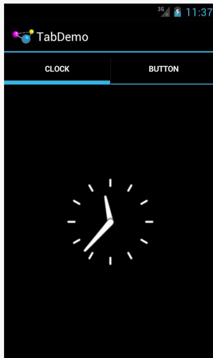
Figure 836: Android 4.0.3
