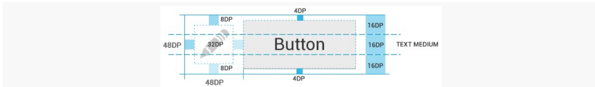
Figure 317: 48dp Rhythm, Depicted (image courtesy of Android Open Source Project)
