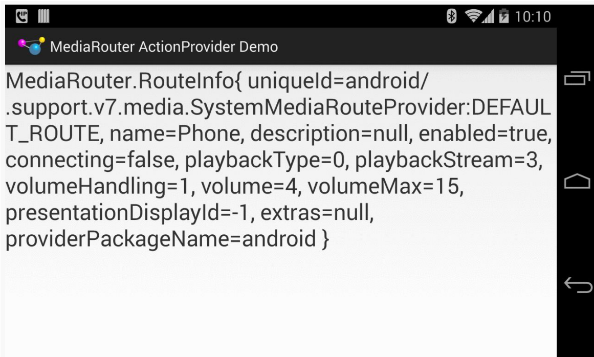
Figure 575: MediaRouter ActionProvider Demo, on a Nexus 4, Showing Default Route
