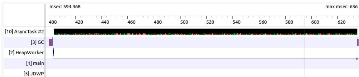
Figure 701: Traceview, zoomed in on ~230 milliseconds of run time
