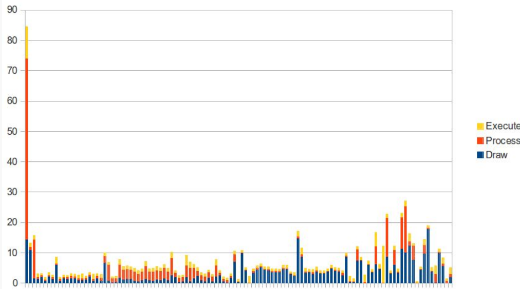
Figure 704: gfxinfo Output, In Stacked Column Chart
