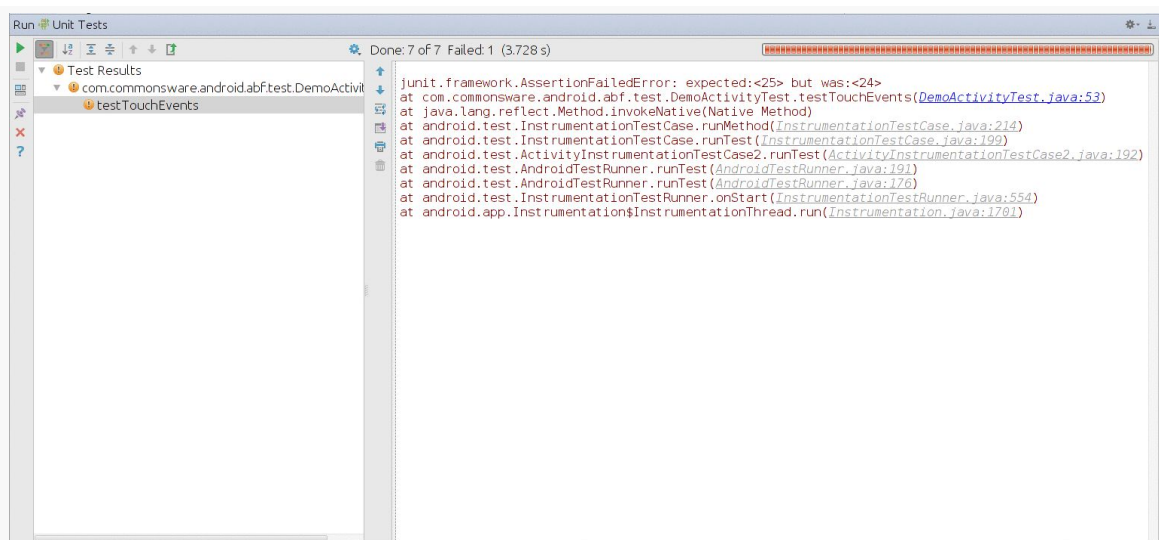
Figure 313: Android Studio, Showing Run Unit Tests Results With a Failure
