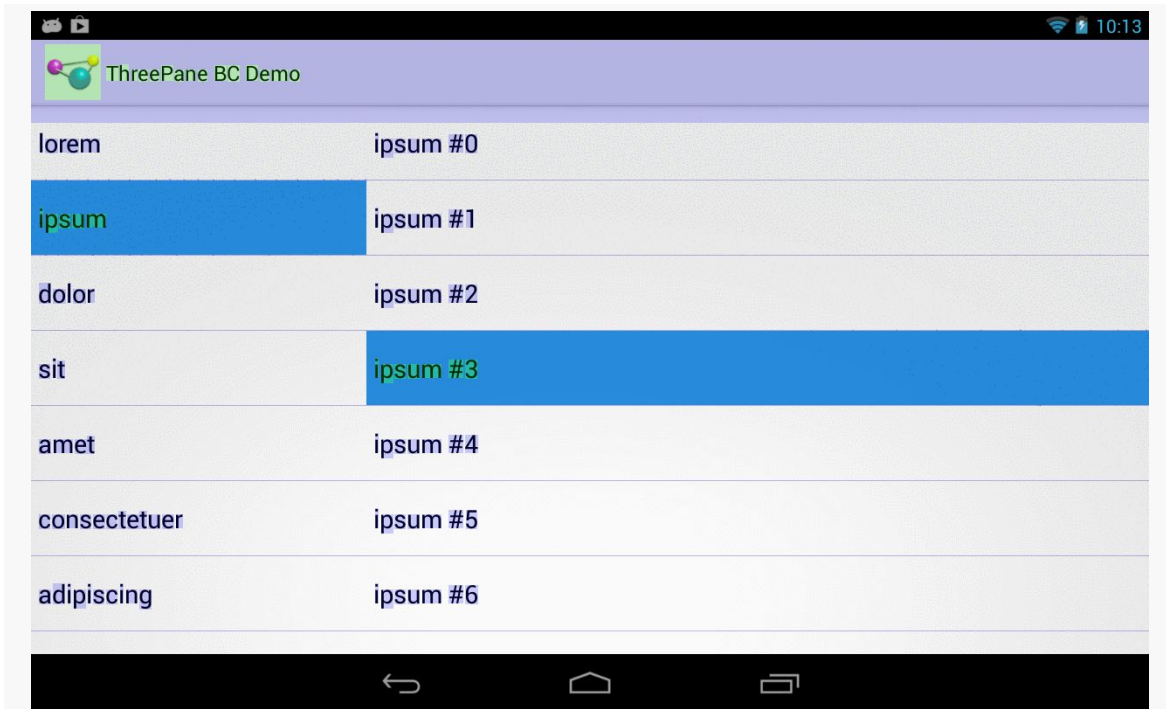
Figure 716: Three-Pane Demo, Left and Middle Panes Via BACK, Showing Overdraw
