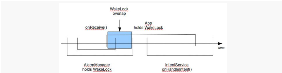
Figure 630: The WakeLock Overlap
