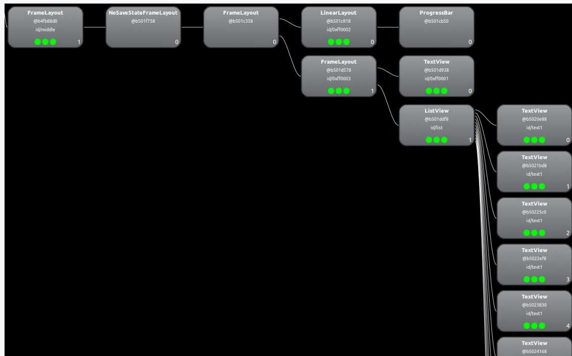
Figure 720: Contents of a ListFragment, from Hierarchy View
