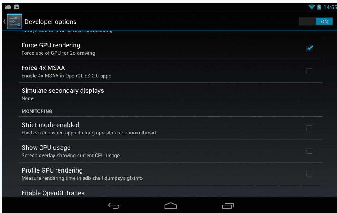
Figure 703: Developer Options, Showing “Force GPU rendering” and “Profile GPU rendering”
