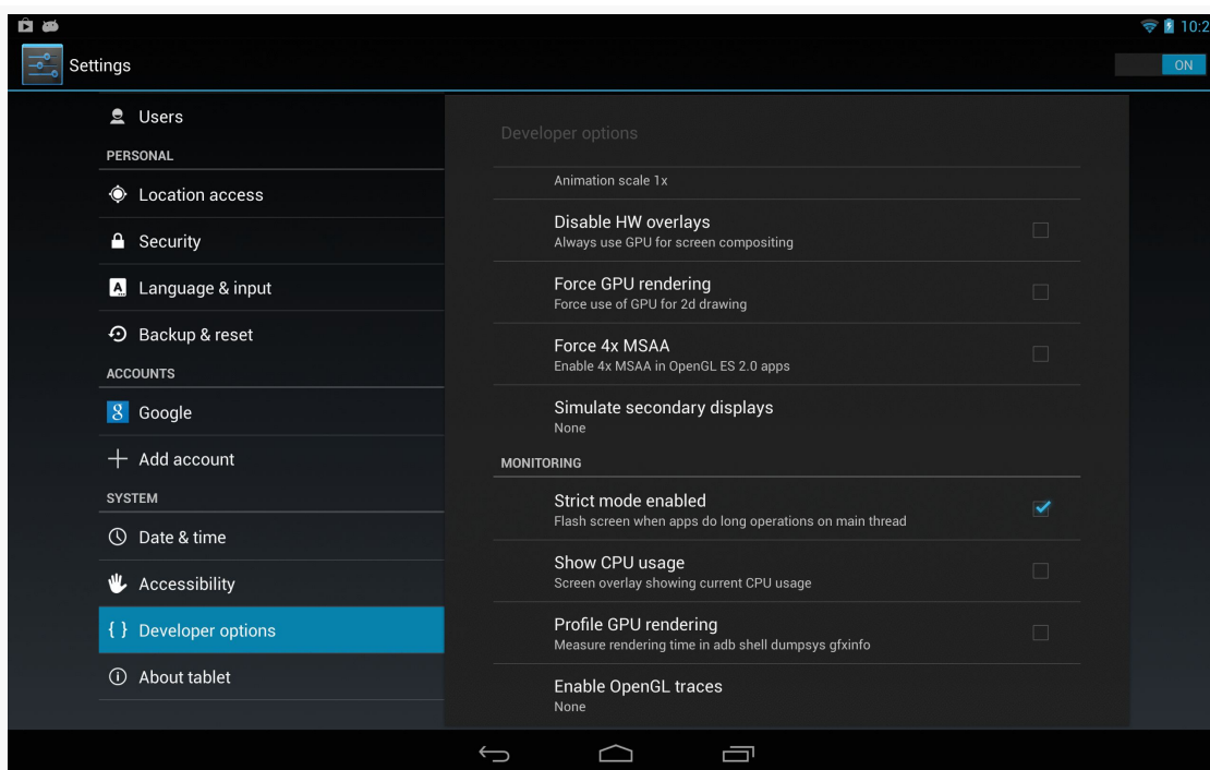
Figure 591: Nexus 10 “Simulate secondary displays” Preference
