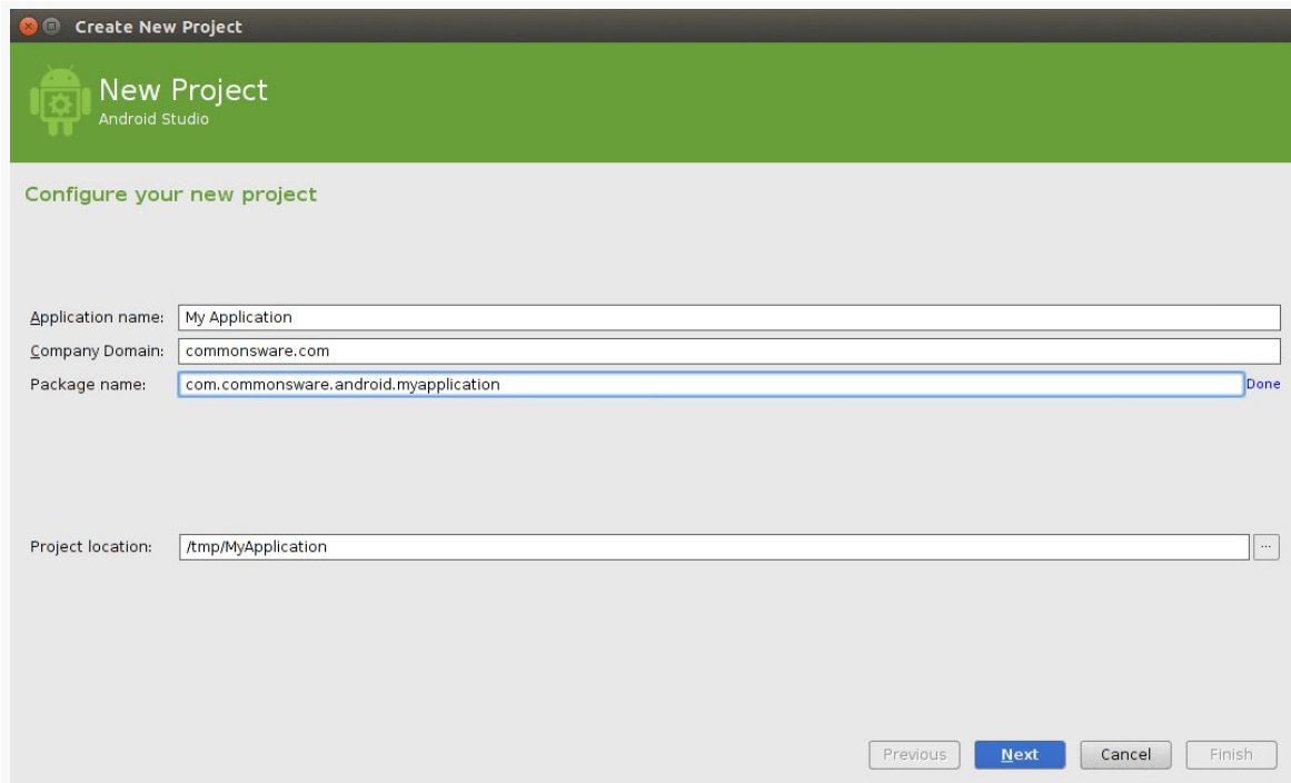
Figure 12: Android Studio Create-Project Wizard, First Page, with Editable Package Name
