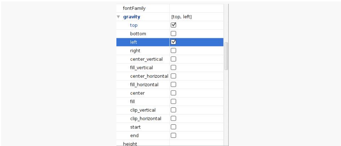
Figure 239: Android Studio Layout Editor Properties Pane, Showing Gravity Options
