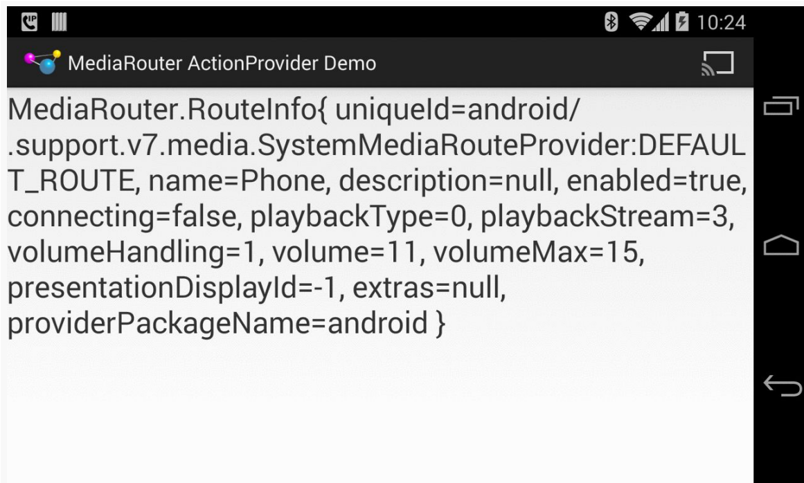
Figure 442: MediaRouter ActionProvider Demo, on a Nexus 4, Showing Default Route and Provider
