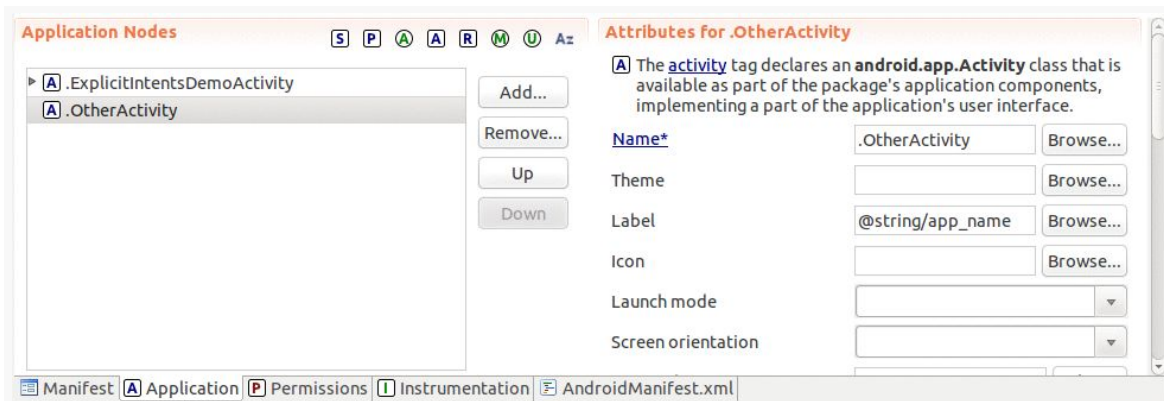
Figure 146: The Eclipse Manifest Editor Application Nodes
