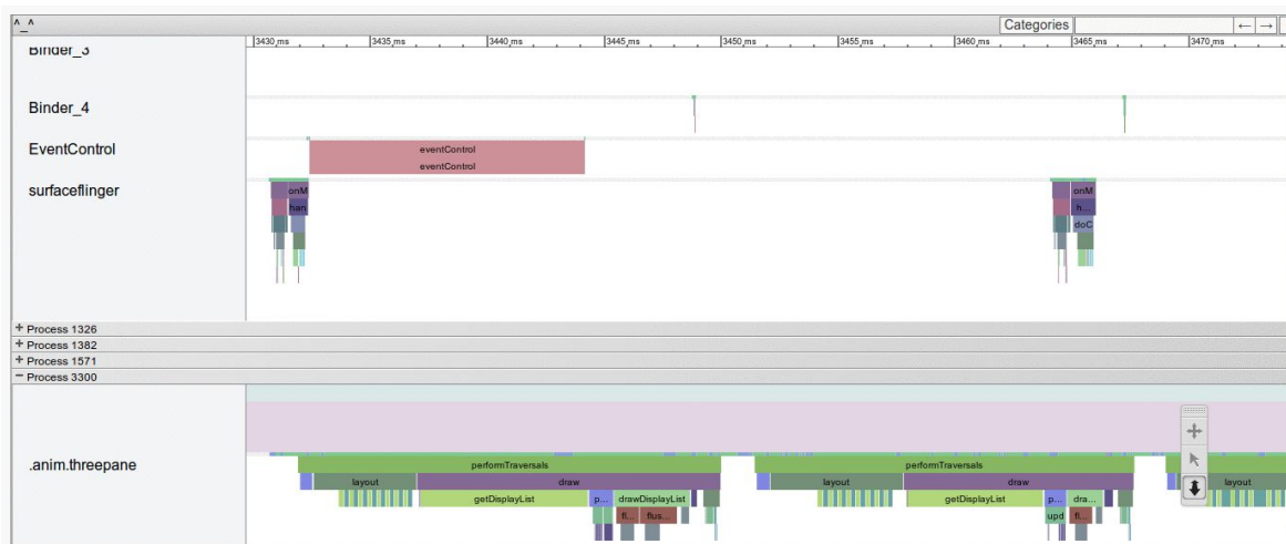
Figure 610: Systrace Output, Zoomed In on 40 Milliseconds of Profiling
