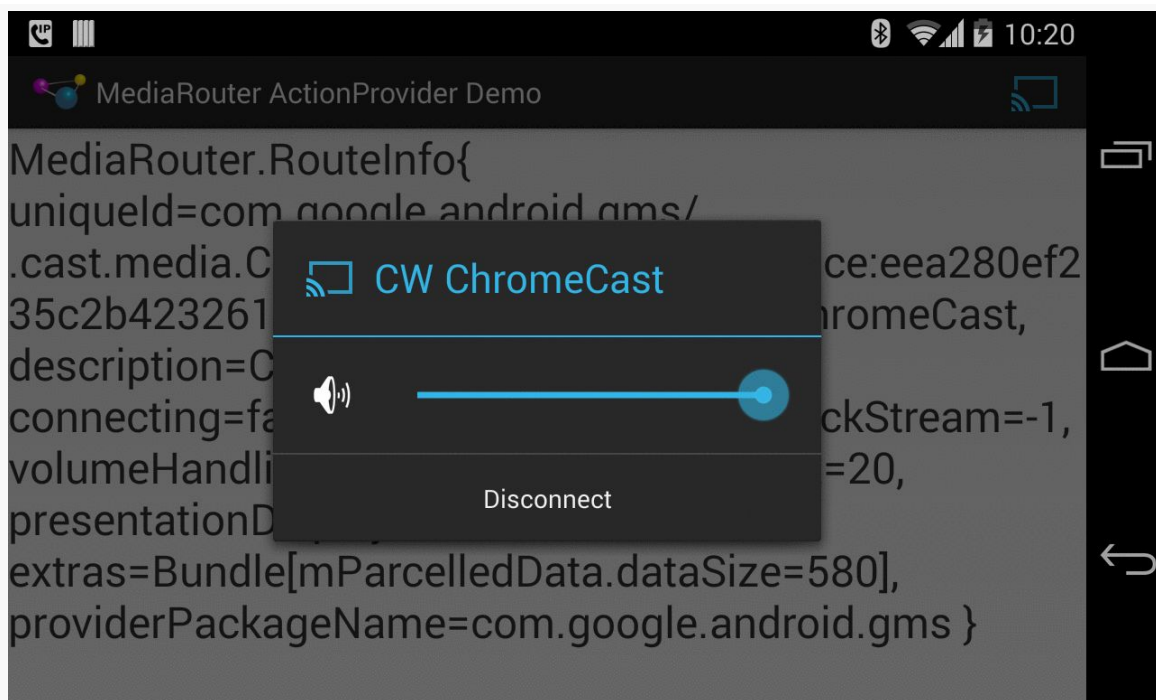
Figure 449: MediaRouter ActionProvider Demo, on a Nexus 4, Showing Route Dialog
