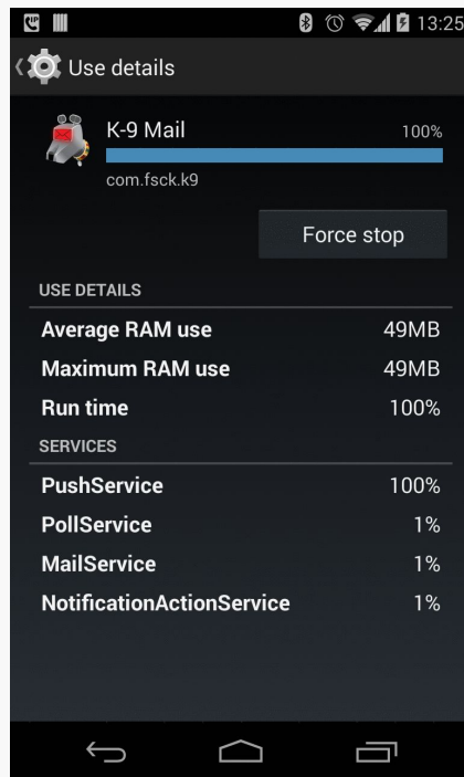
Figure 650: Process Stats Details for K-9 Mail
