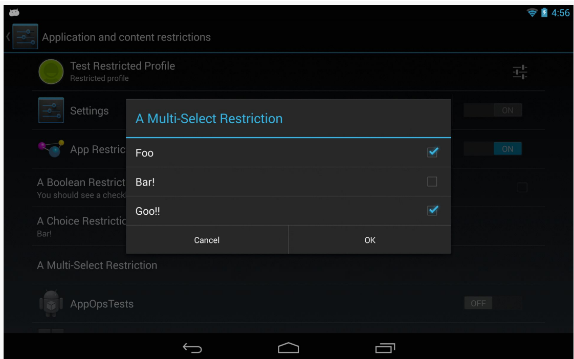
Figure 476: Restricted Profile, Showing Multi-Select Restriction
