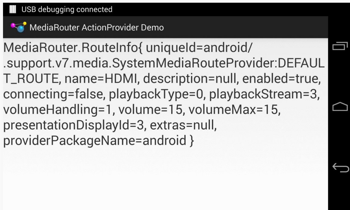
Figure 444: MediaRouter ActionProvider Demo, on a Nexus 4, Showing Live Video Route
