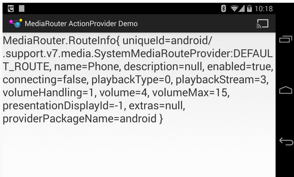
Figure 445: MediaRouter ActionProvider Demo, on a Nexus 4, Showing ActionProvider
