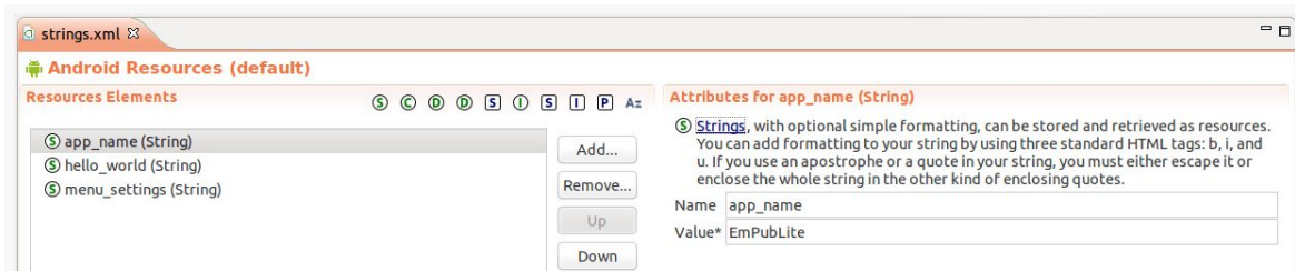
Figure 47: Eclipse String Resources Editor with Details
