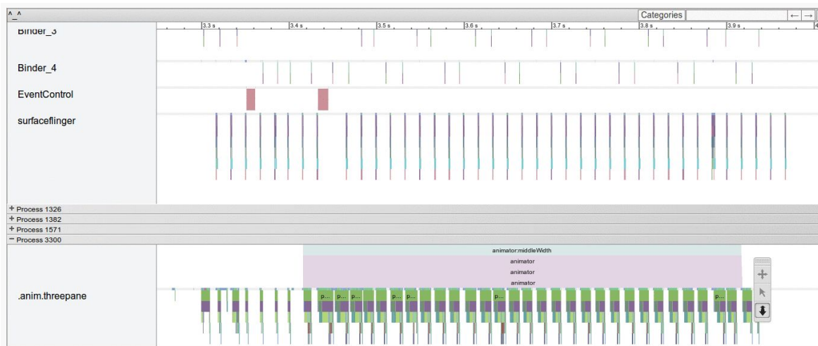
Figure 609: Systrace Output, Zoomed In on 0.7 Seconds of Profiling
