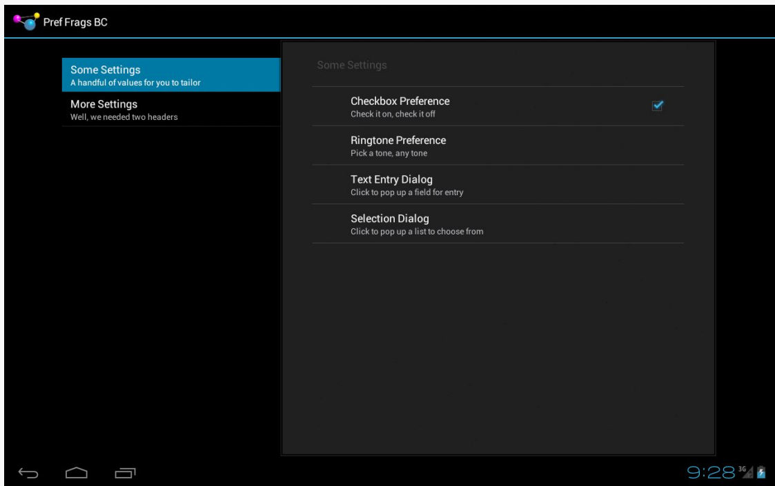
Figure 173: Android 4.0 PreferenceActivity, on Tablet
