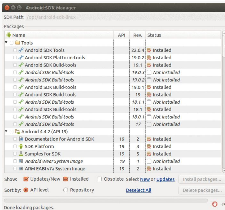
Figure 5: Android SDK Manager
