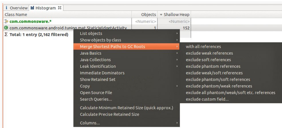
Figure 636: A filtered histogram, showing com.commonware.* objects
