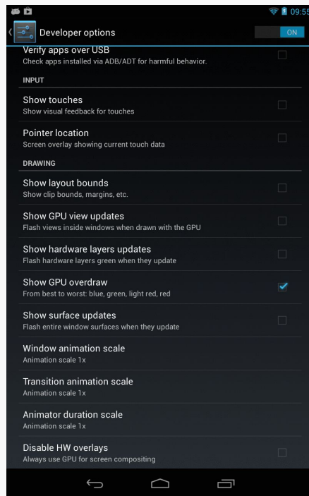
Figure 612: Nexus 7 Developer Options, with “Show GPU overdraw”
