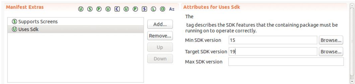
Figure 39: Eclipse Manifest Extras, Showing “Uses Sdk” Filled In
