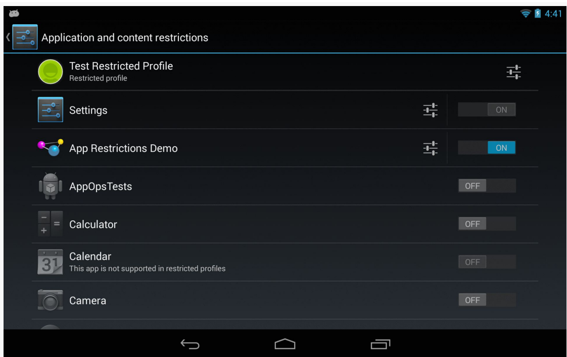
Figure 473: Restricted Profile, Showing App Settings Icon
