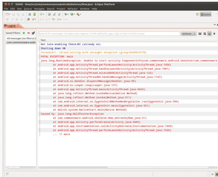
Figure 77: Eclipse Window with LogCat View Scrolled Right
