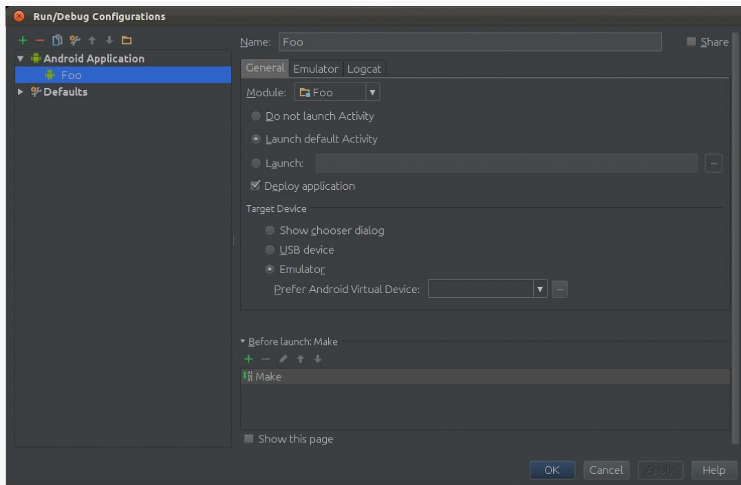
Figure 567: IDEA Run/Debug Configurations Dialog
