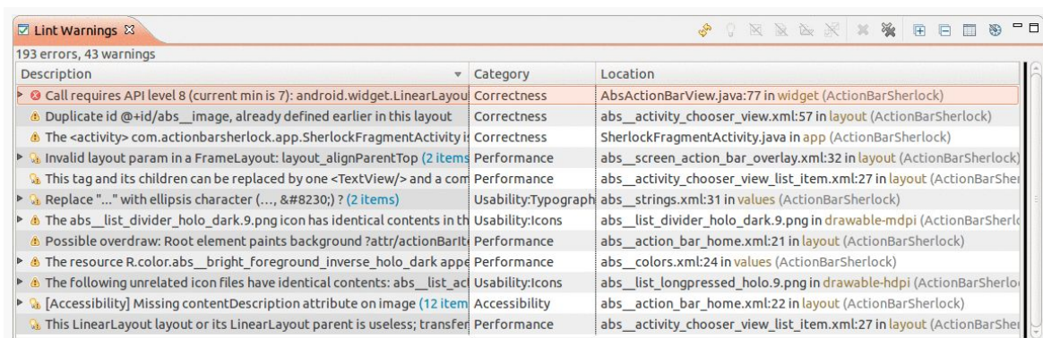
Figure 540: Eclipse Lint Warnings View
