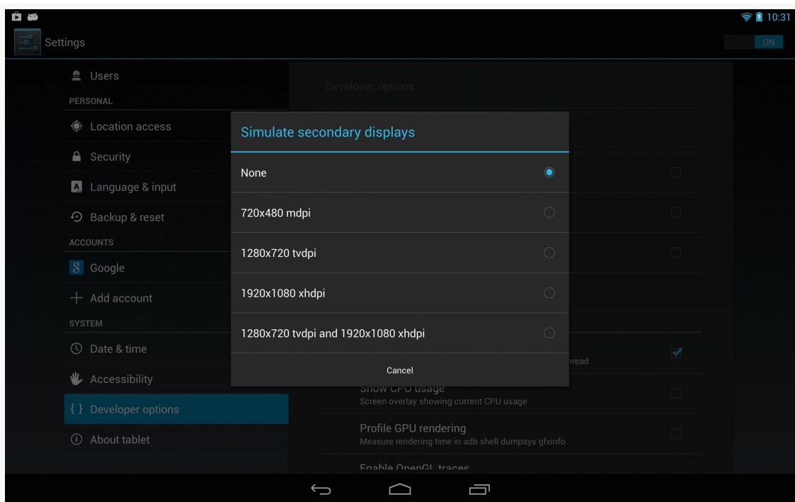
Figure 393: Nexus 10 “Simulate secondary displays” Options
