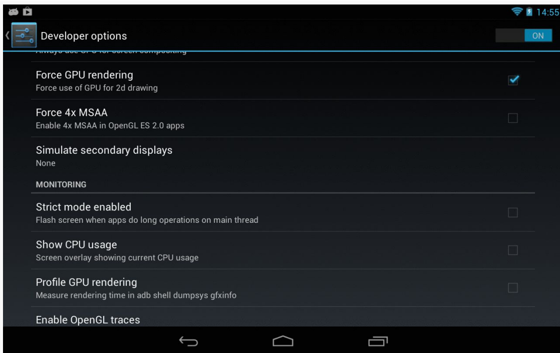
Figure 583: Developer Options, Showing “Force GPU rendering” and “Profile GPU rendering”
