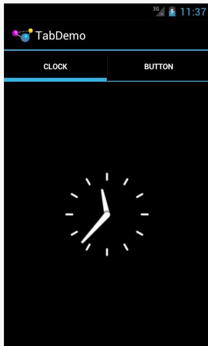
Figure 656: Android 4.0.3
