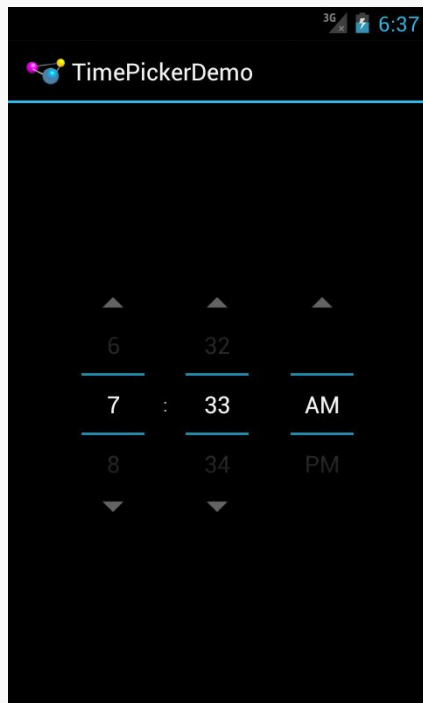
Figure 658: Android 4.0.3
