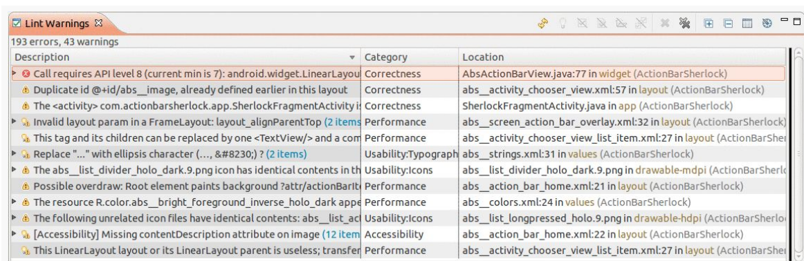
Figure 541: Eclipse Lint Warnings View
