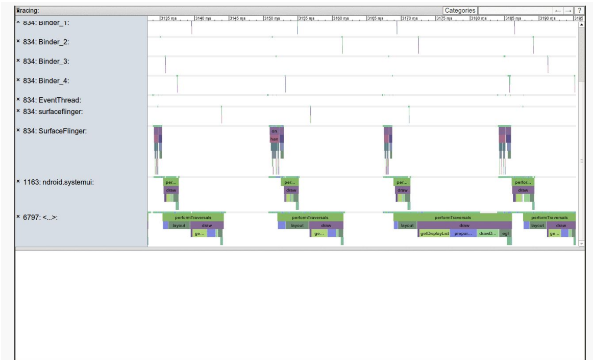
Figure 591: Systrace Output, Showing Semi-Relevant Information
