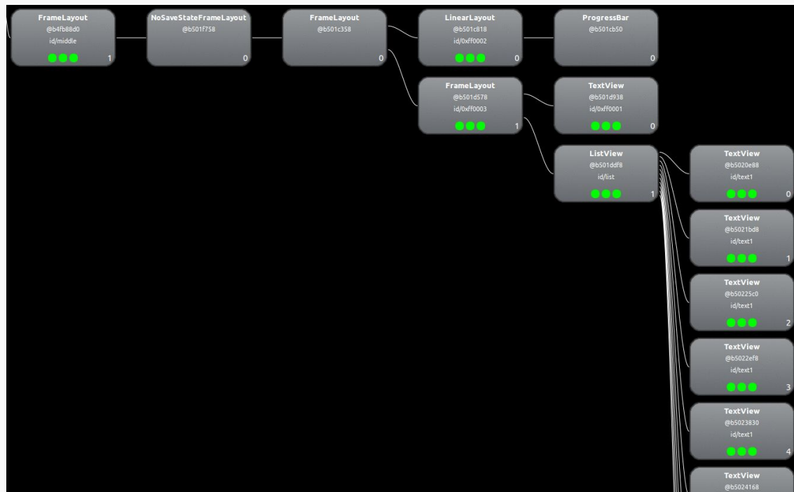
Figure 601: Contents of a ListFragment, from Hierarchy View
