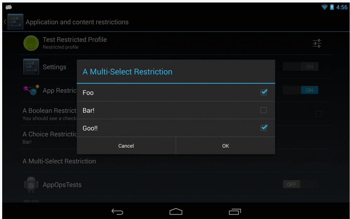
Figure 459: Restricted Profile, Showing Multi-Select Restriction
