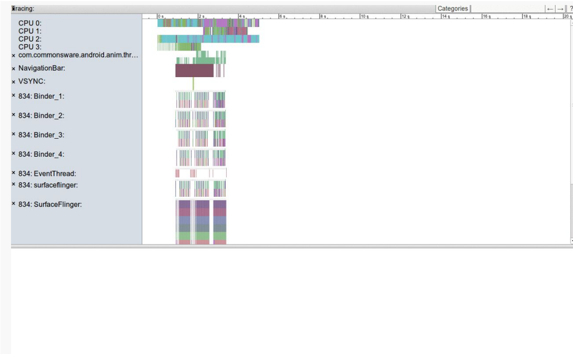
Figure 589: Systrace Output, As Initially Viewed
