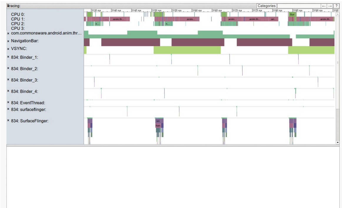
Figure 590: Systrace Output, Zoomed In, Showing 3135ms to 3190ms
