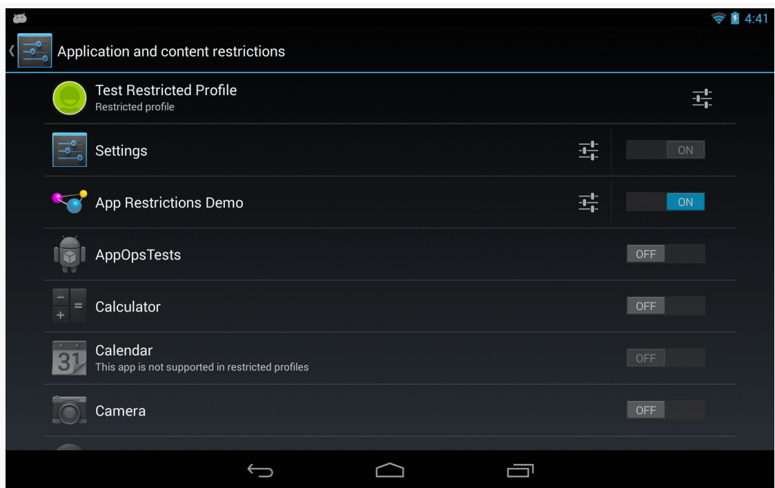
Figure 456: Restricted Profile, Showing App Settings Icon
