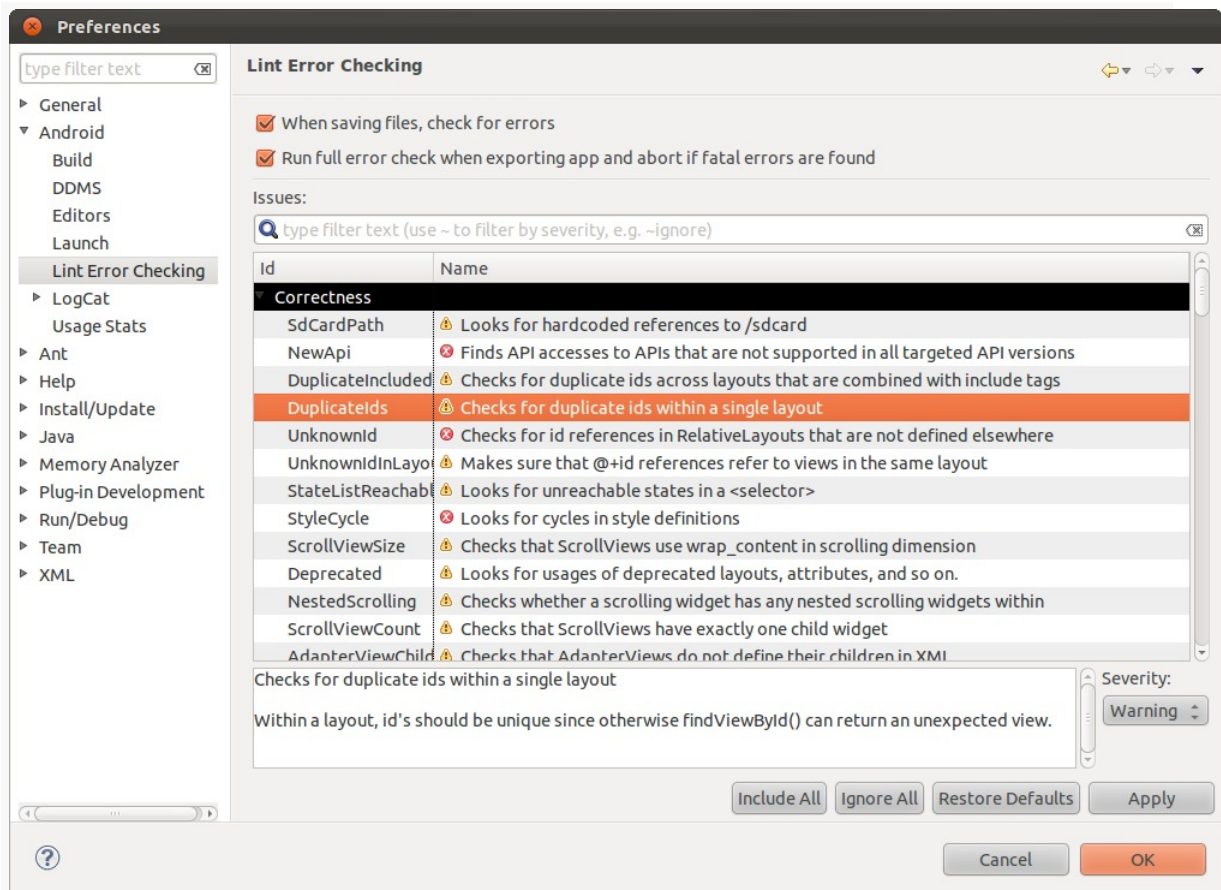
Figure 542: Lint Error Checking Preferences
