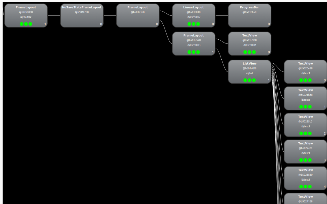
Figure 537: Contents of a ListFragment, from Hierarchy View
