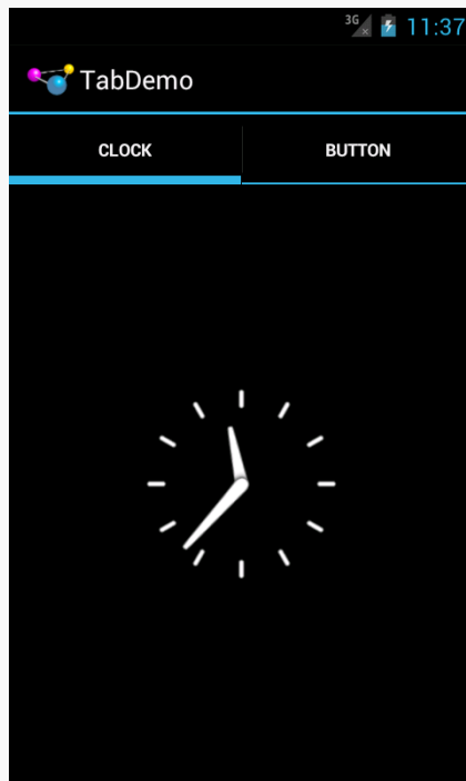
Figure 593: Android 4.0.3
