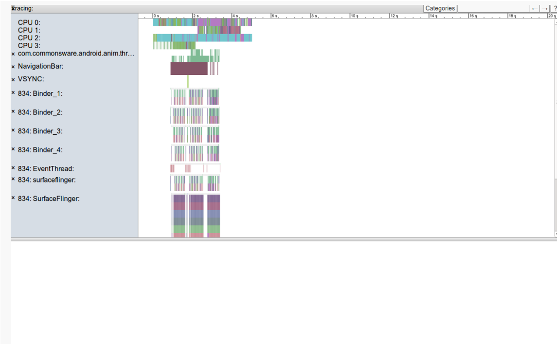
Figure 525: Systrace Output, As Initially Viewed
