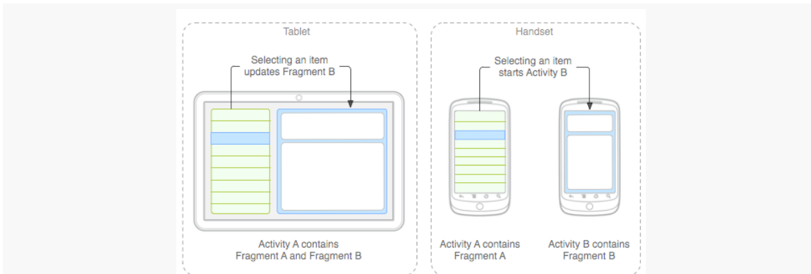
Figure 217: Tablets vs. Handsets (image courtesy of Android Open Source Project)
