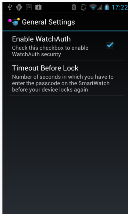
Figure 613: WatchAuth Preferences
