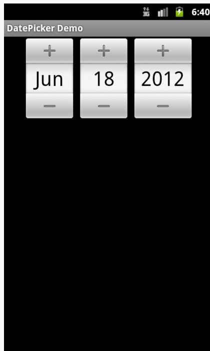
Figure 580: Android 2.3.3
