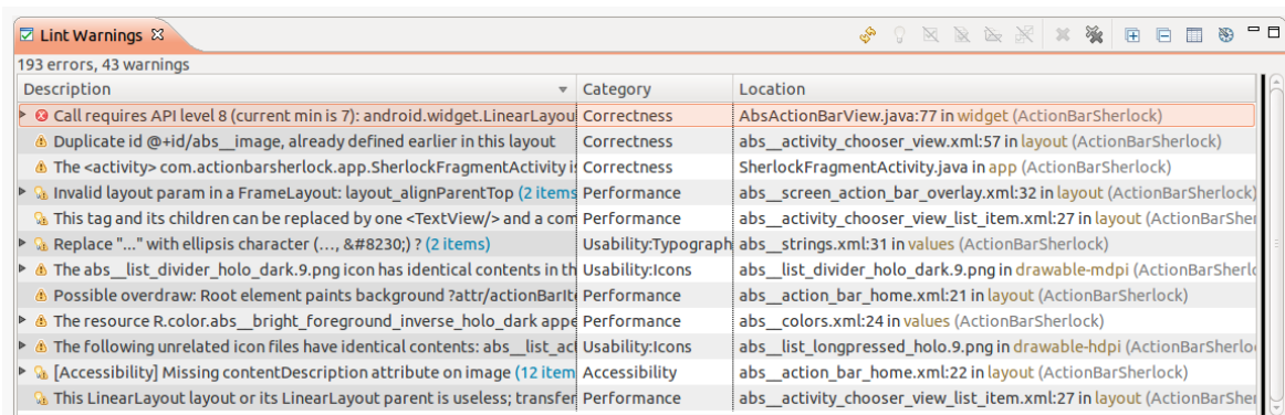
Figure 498: Eclipse Lint Warnings View
