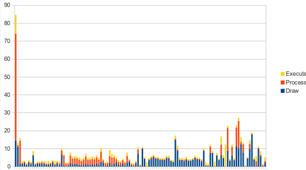
Figure 521: gfxinfo Output, In Stacked Column Chart
