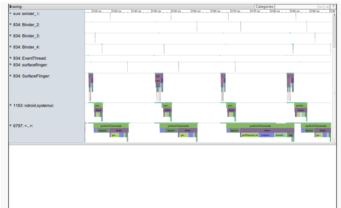
Figure 527: Systrace Output, Showing Semi-Relevant Information
