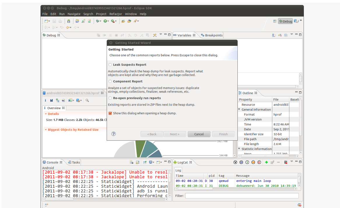
Figure 543: The MAT Eclipse perspective, as initially opened
