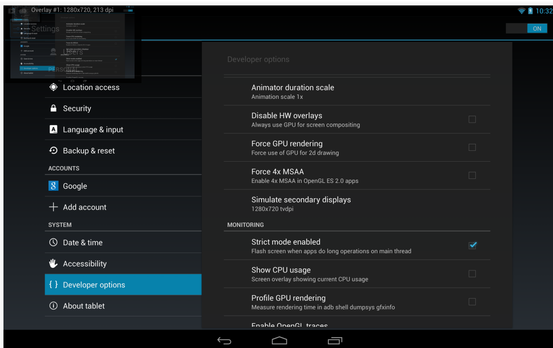
Figure 373: Nexus 10, Simulating a 720p Secondary Screen
