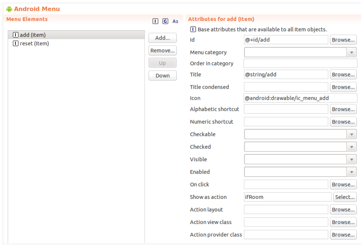
Figure 122: Eclipse Menu Resource Editor
