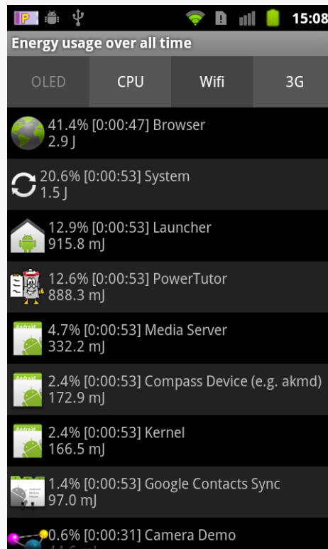
Figure 488: The PowerTutor application roster
