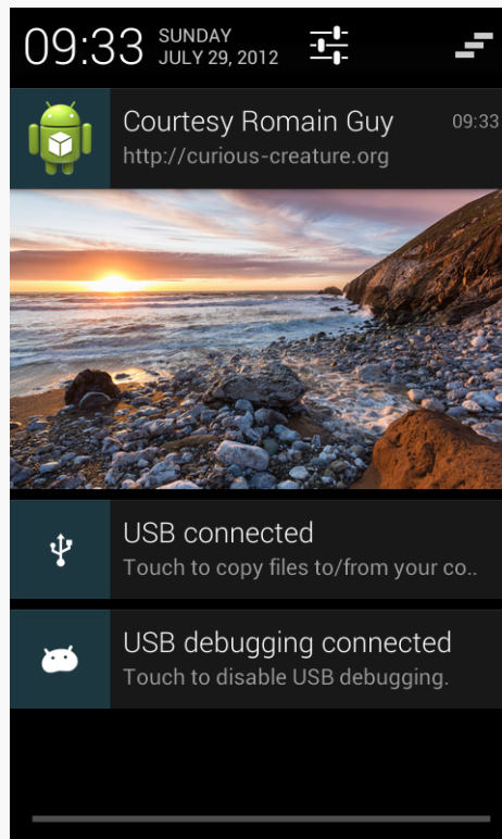
Figure 189: BigPicture Notification, from NotificationCompat2 Sample App, on a Nexus S
