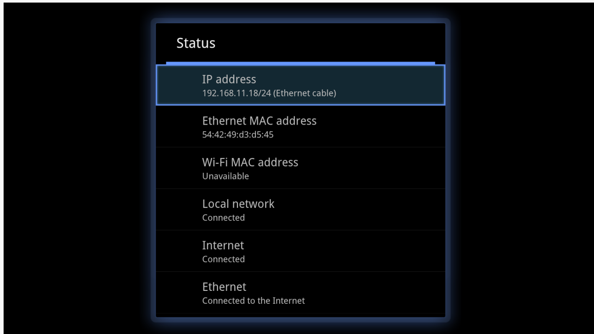
Figure 353: IP Address on Google TV
