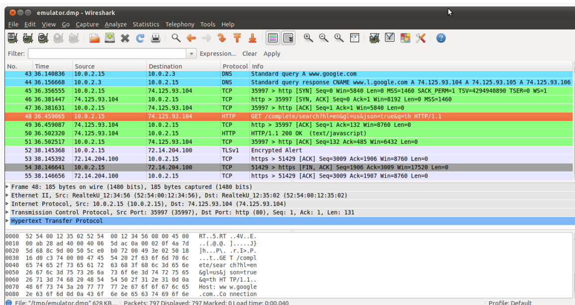
Figure 410: Wireshark examining captured emulator packets
