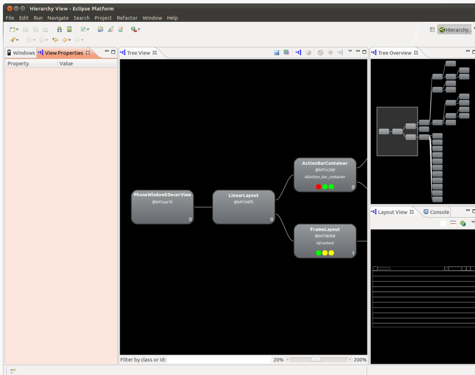
Figure 389: Hierarchy View, in Eclipse, Showing an Activity
