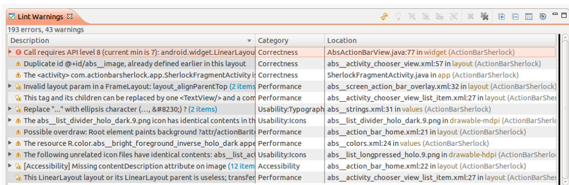
Figure 490: Eclipse Lint Warnings View
