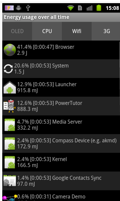
Figure 553: The PowerTutor application roster
