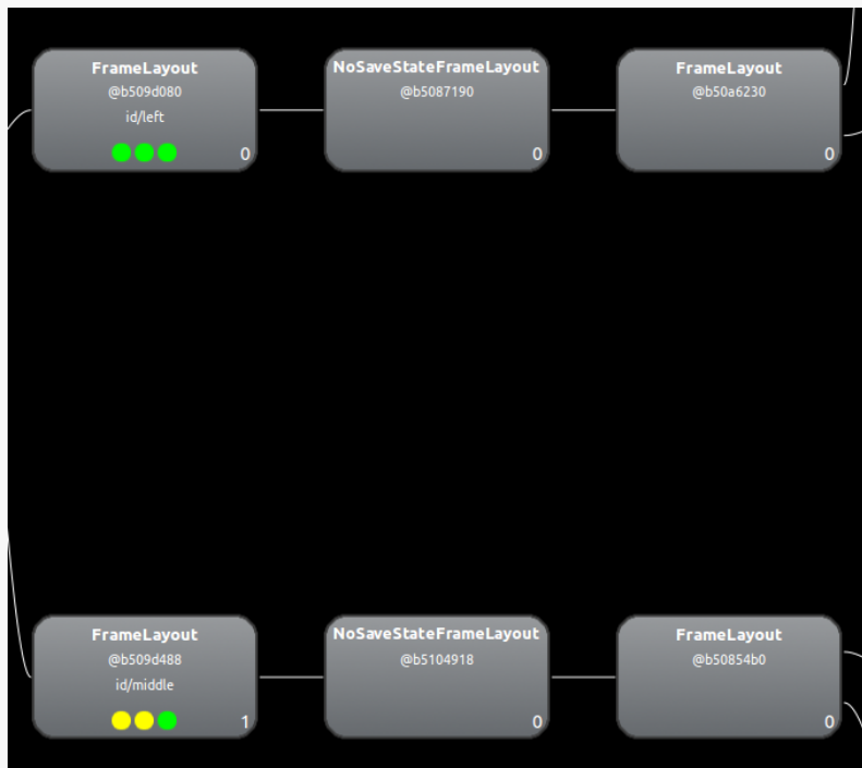
Figure 528: More Single-Child Containers in Three-Pane Demo, from Hierarchy View
