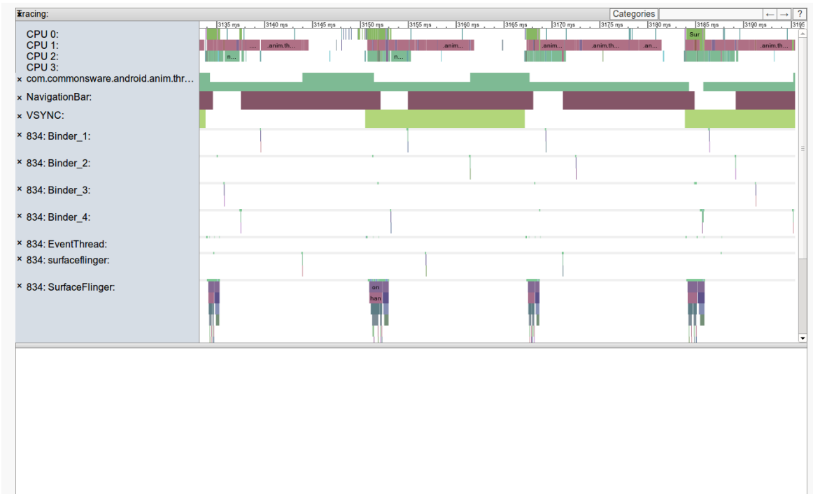
Figure 518: Systrace Output, Zoomed In, Showing 3135ms to 3190ms
