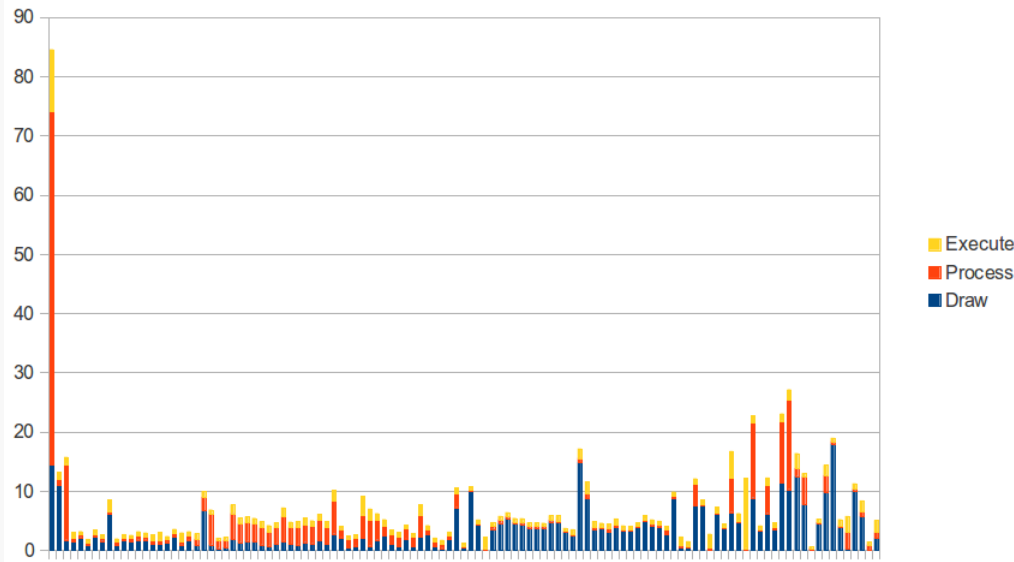
Figure 513: gfxinfo Output, In Stacked Column Chart
