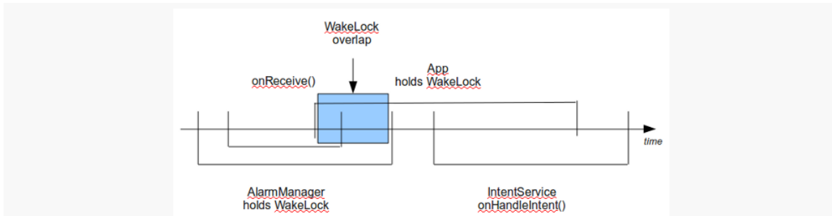
Figure 433: The WakeLock Overlap
