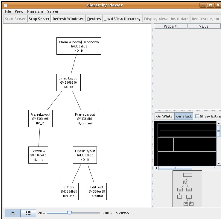
Figure 119. Hierarchy Viewer Layout View
