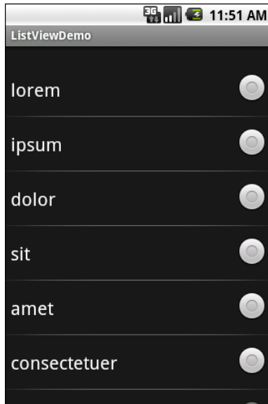
Figure 20. Single-select mode
