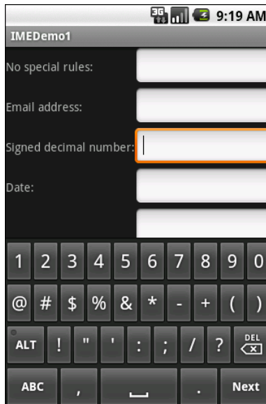
Figure 50. The input method editor for signed decimal numbers
