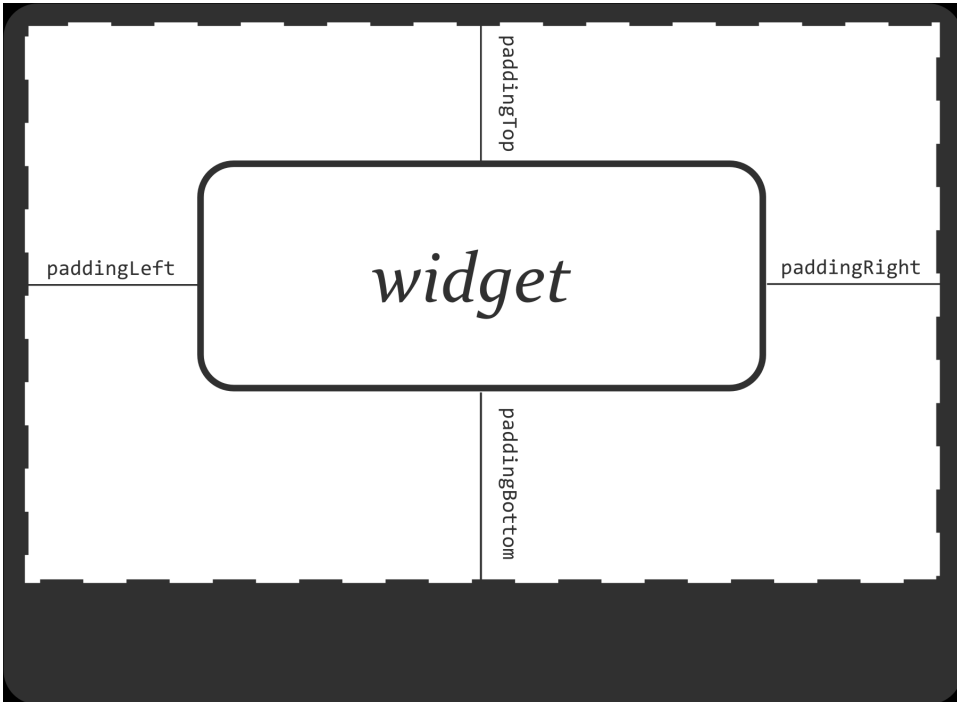
Figure 11. The relationship between a widget, its cell, and the padding values
