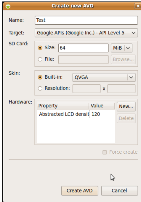
Figure 2. Create new AVD dialog
